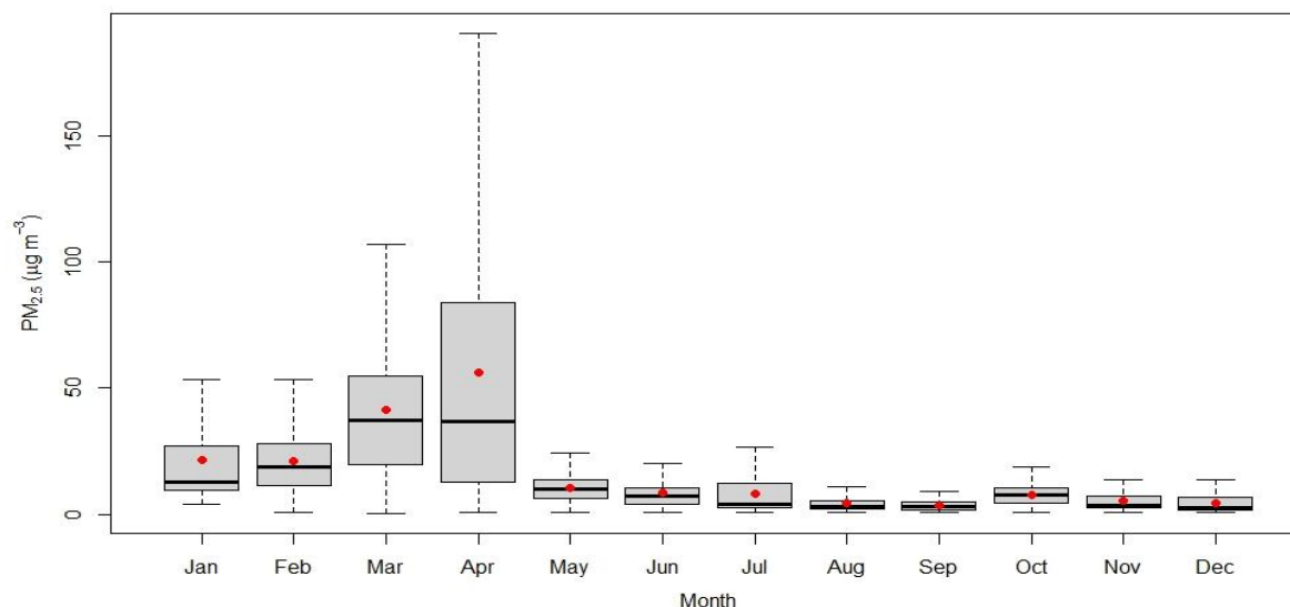
Figure 2.3.5: Monthly variation of PM_{2.5}
