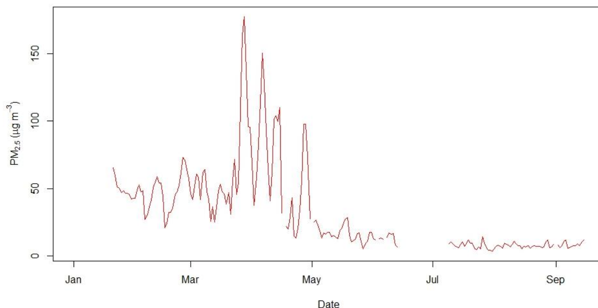
Figure 2.7.4: Daily mean concentration of PM 2.5
