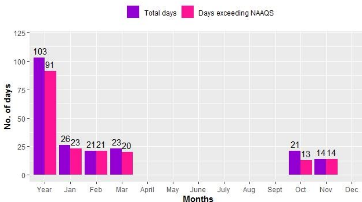
Figure 2.1.8: Compliance status of PM 2.5
