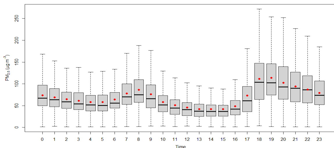
Figure 2.1.3: Diurnal variation of PM 2.5
