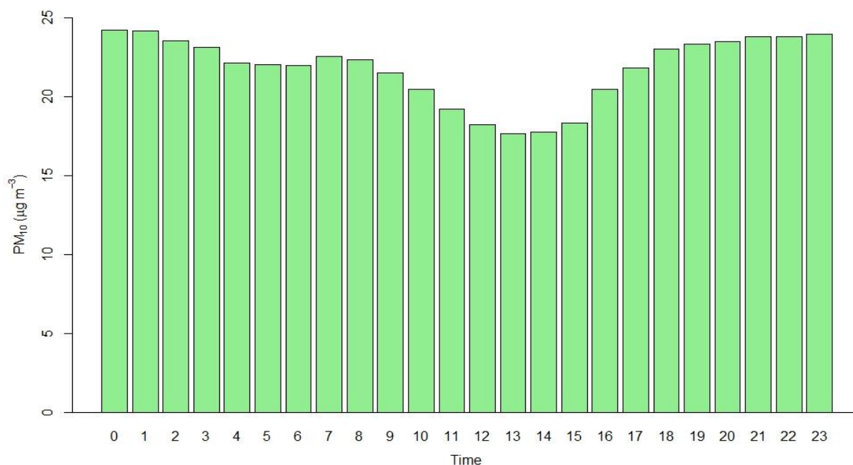
Figure 2.3.10: Hourly average of PM 10 .
