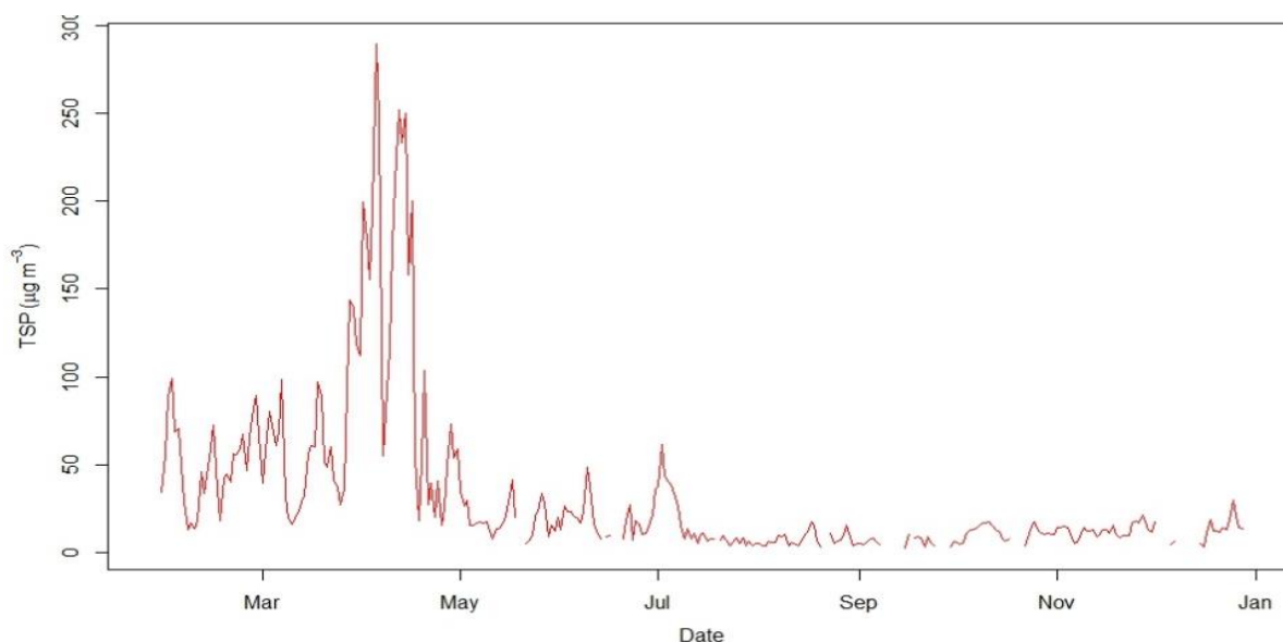
Figure 2.3.20: Daily mean concentration of TSP
