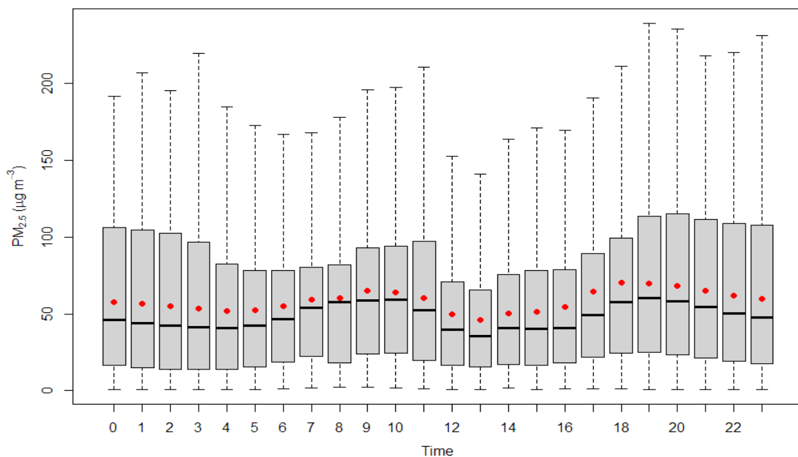
Figure 2.6.3: Diurnal variation of PM 2.5
