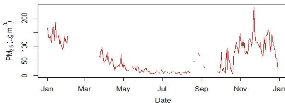
Figure 2.14.4: Daily mean concentration of PM 2.5
