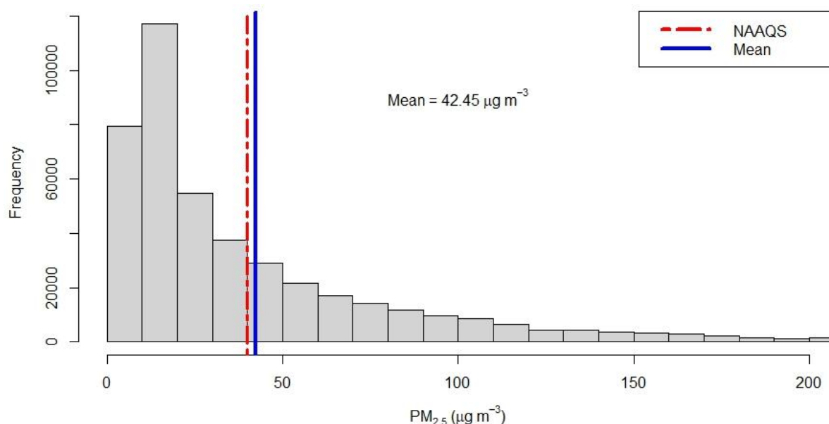
Figure 2.8.1: Histogram of PM 2.5
