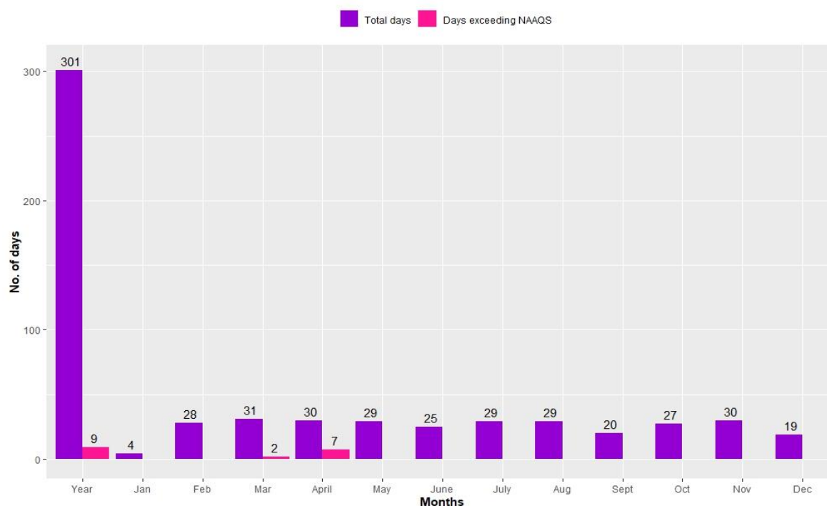
Figure 2.3.16: Compliance status of PM 10
