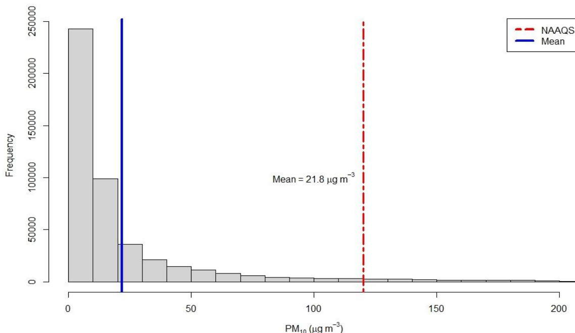
Figure 2.3.9: Histogram of PM 10
