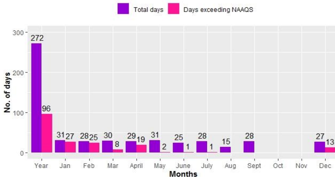
Figure 2.5.8: Compliance status of PM 2.5
