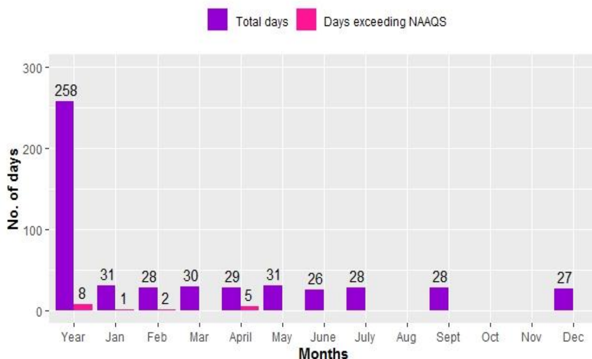
Figure 2.5.24: Compliance status of TSP
