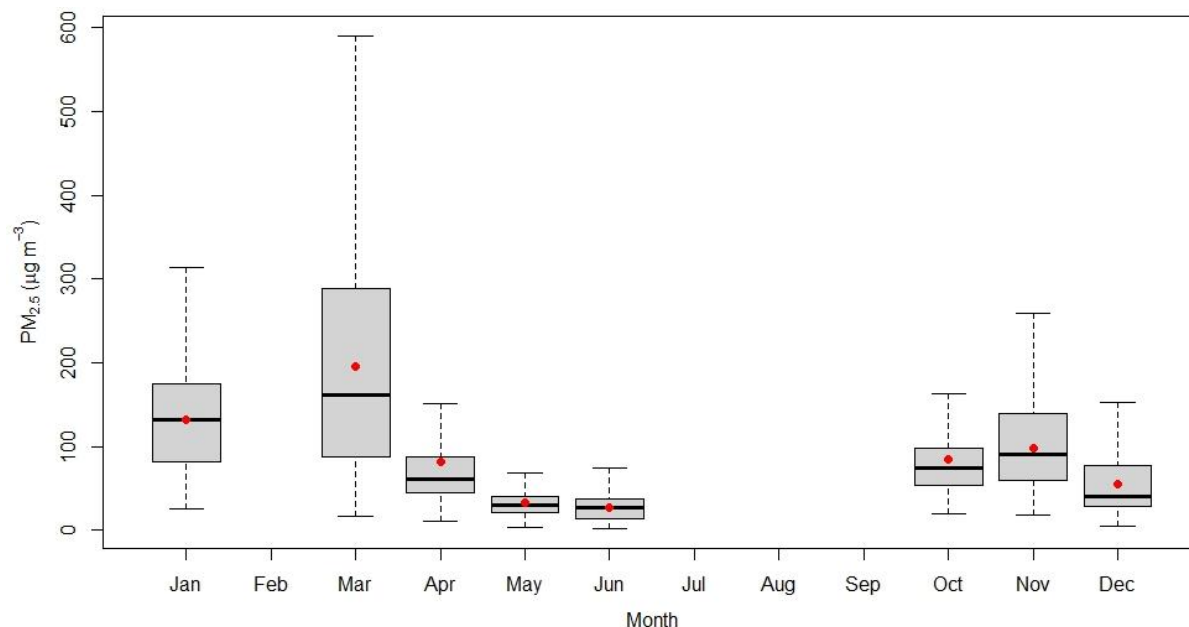
Figure 2.12.5: Monthly variation of PM 2.5
