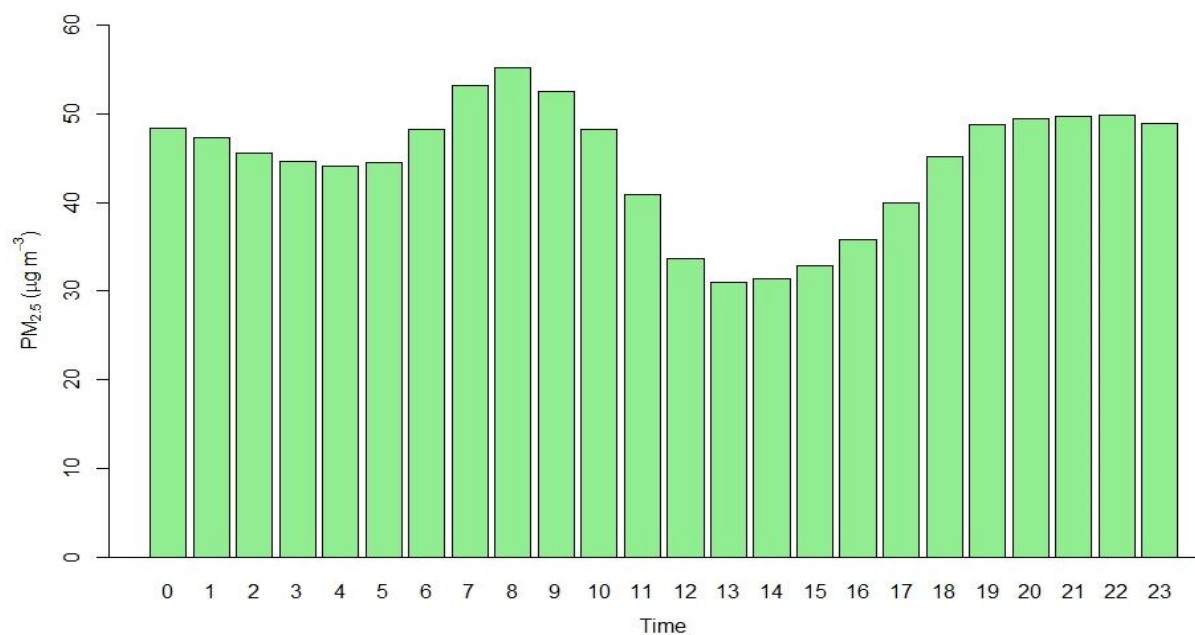
Figure 2.11.2: Hourly average of PM 2.5
