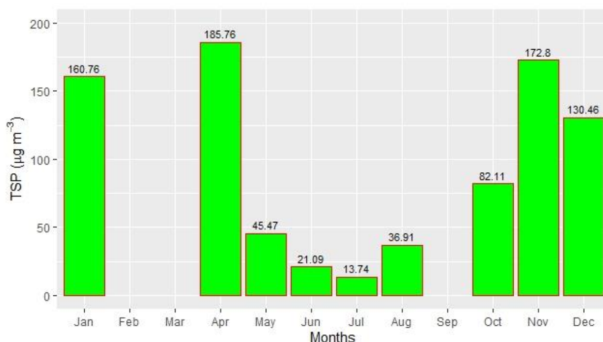
Figure 2.14.21: Monthly average of TSP
