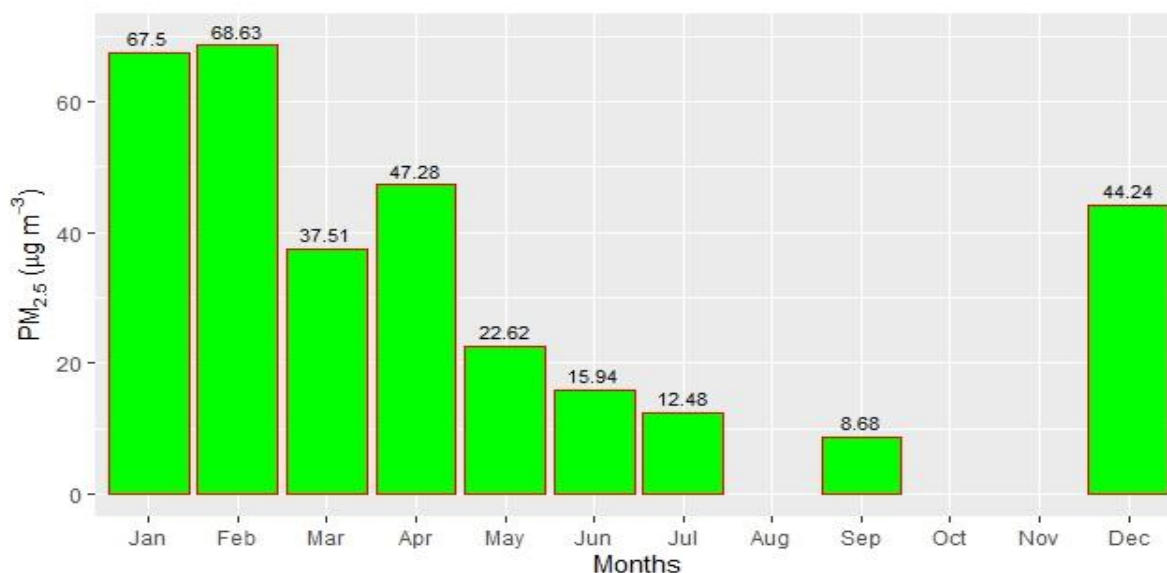
Figure 2.5.6: Monthly average PM 2.5
