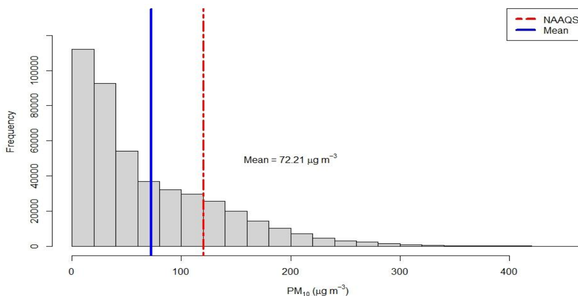
Figure 2.11.9: Histogram of PM 10
