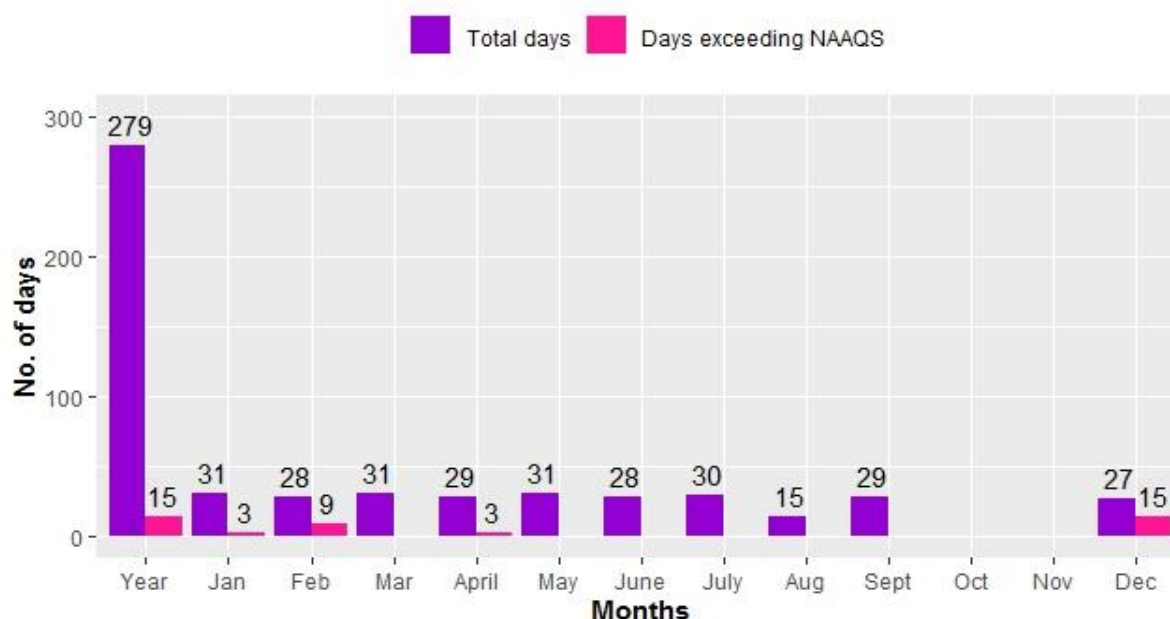
Figure 2.5.16: Compliance status of PM 10
