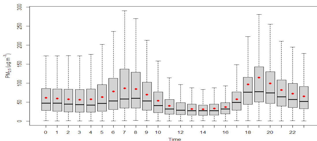
Figure 2.2.3: Diurnal variation of PM 2.5
