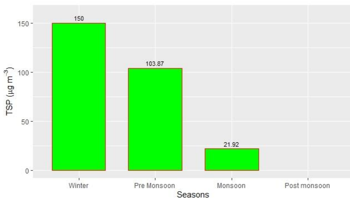
Figure 2.5.23: Seasonal variation of TSP
