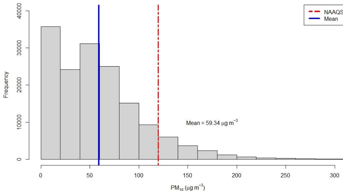
Figure 2.15.8: Histogram of PM 10
