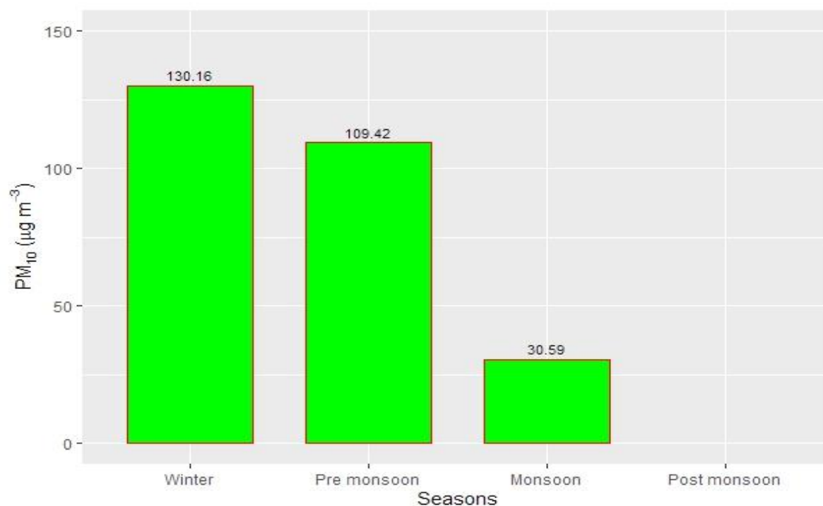
Figure 2.10.15: Seasonal variation of PM 10
