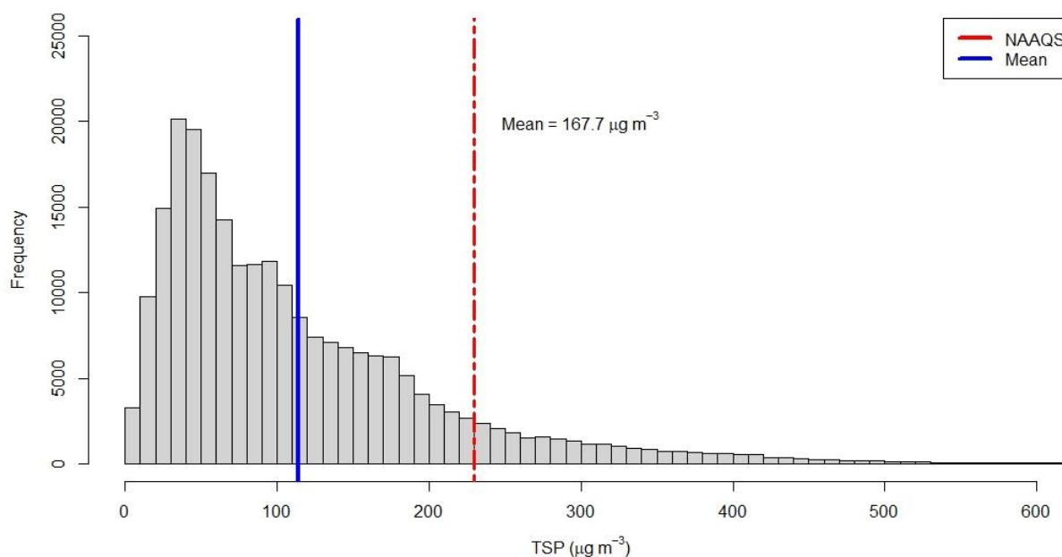
Figure 2.12.15: Histogram of TSP
