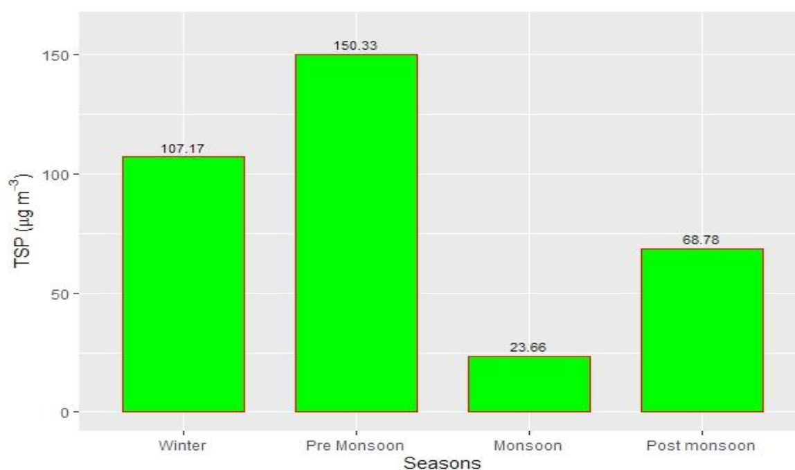
Figure 2.6.23: Seasonal variation of TSP
