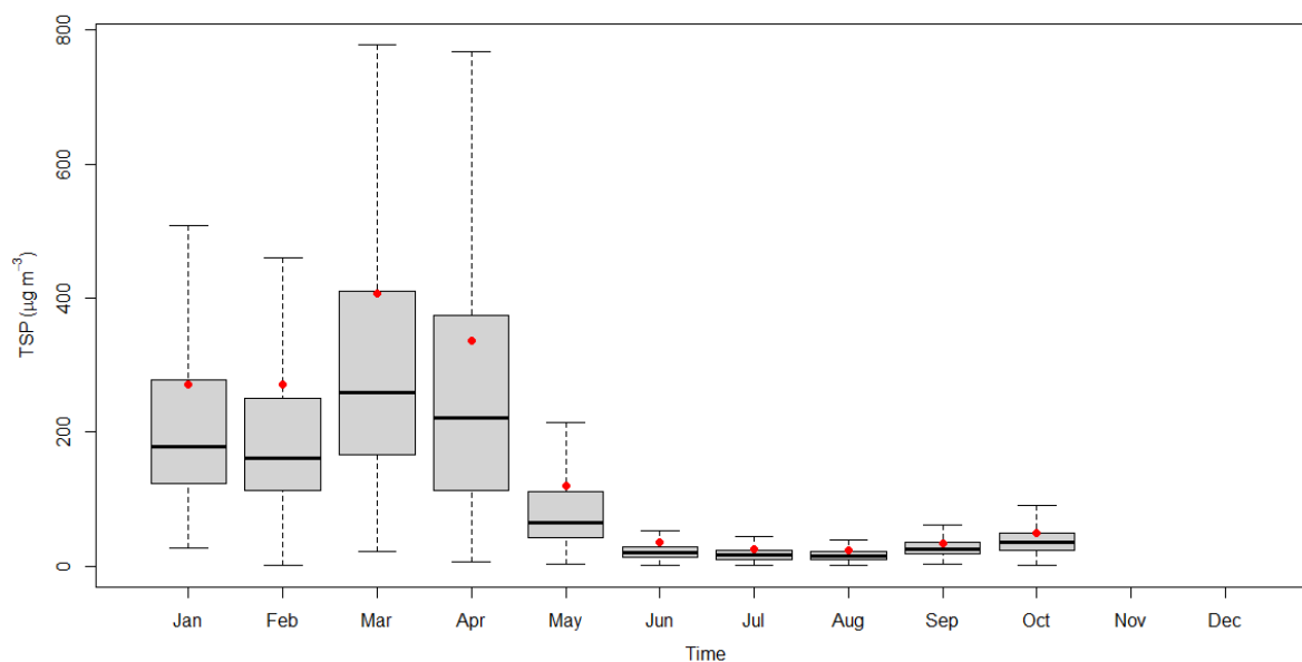
Figure 2.9.22: Monthly variation of TSP
