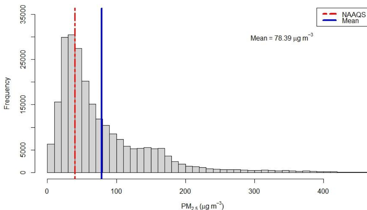
Figure 2.12.1: Histogram of PM 2.5
