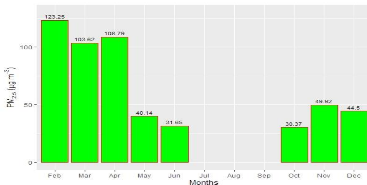
Figure 2.2.6: Monthly average PM 2.5
