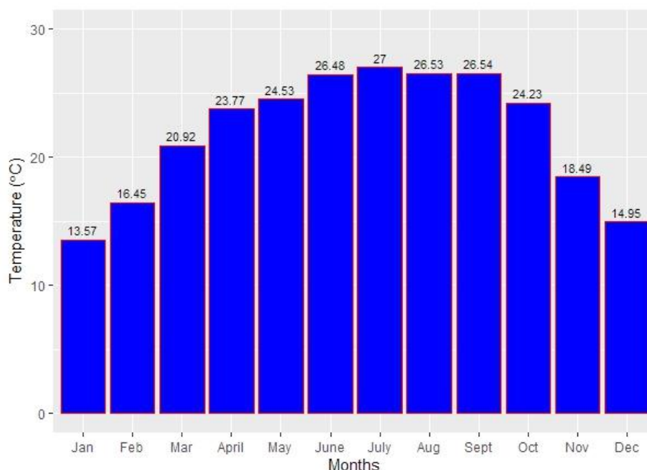
Figure 2.18.2: Monthly average temperature with months in year 2021
