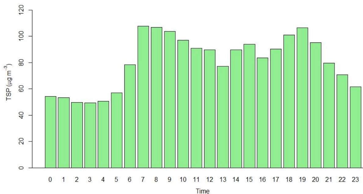
Figure 2.15.16: Hourly average of TSP
