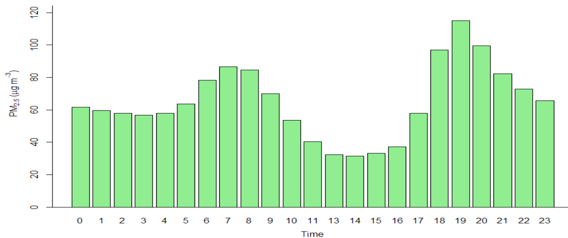
Figure 2.2.2: Hourly average of PM 2.5
