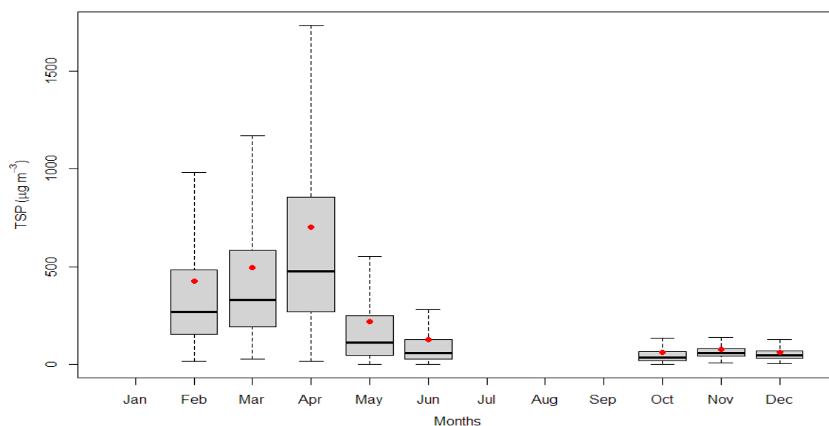
Figure 2.2.21: Monthly variation of TSP
