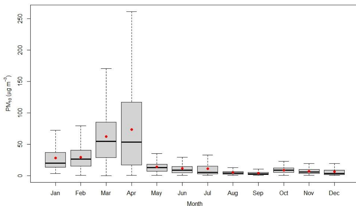
Figure 2.3.13: Monthly variation of PM 10
