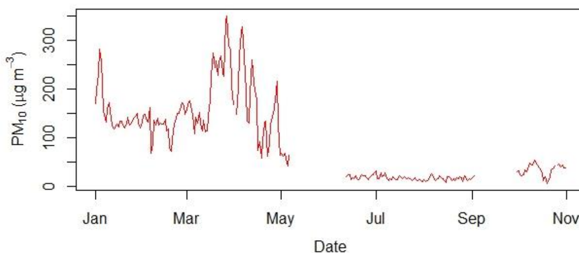
Figure 2.9.12: Daily mean concentration of PM 10
