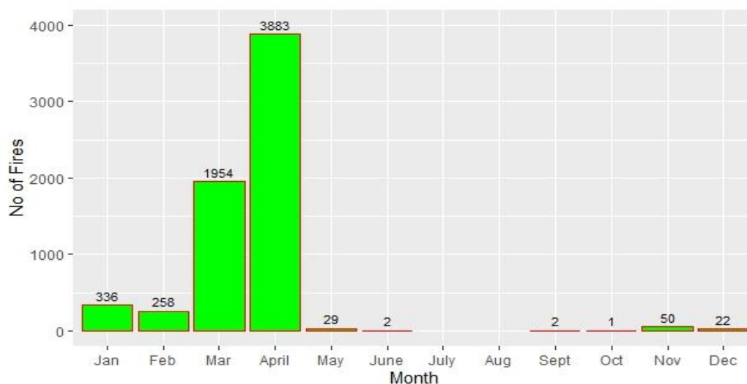
Figure 2.18.1: Number of fires with months in year 2021
