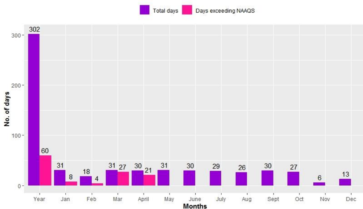
Figure 2.8.16: Compliance status of PM 10
