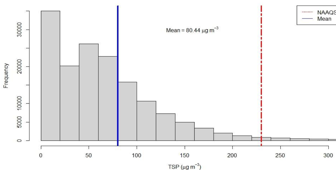
Figure 2.15.15: Histogram of TSP
