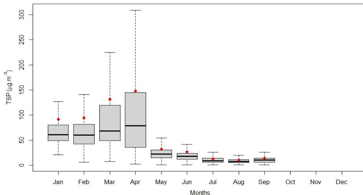
Figure 2.7.21: Monthly variation of TSP
