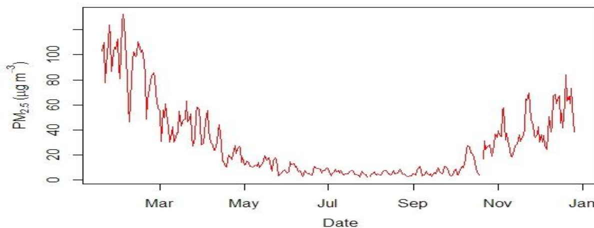
Figure 2.13.4: Daily mean concentration of PM 2.5
