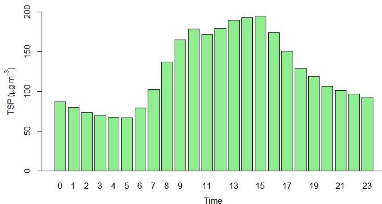
Figure 2.11.18: Hourly average of TSP
