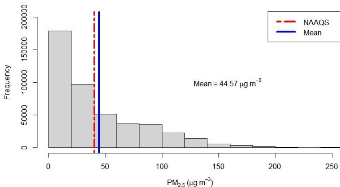
Figure 2.11.1: Histogram of PM 2.5
