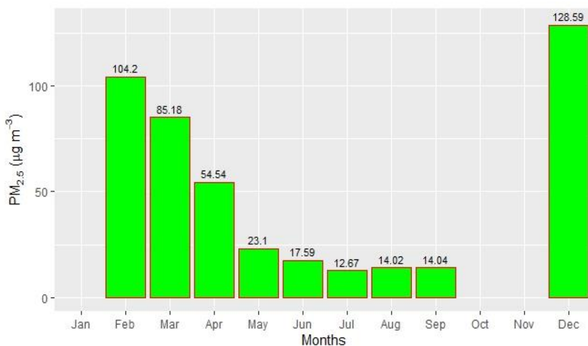
Figure 2.17.6: Monthly average PM_{2.5}
