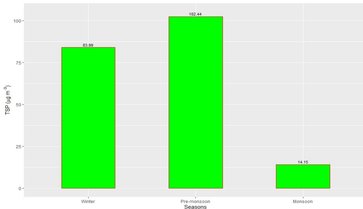
Figure 2.7.23: Seasonal variation of TSP
