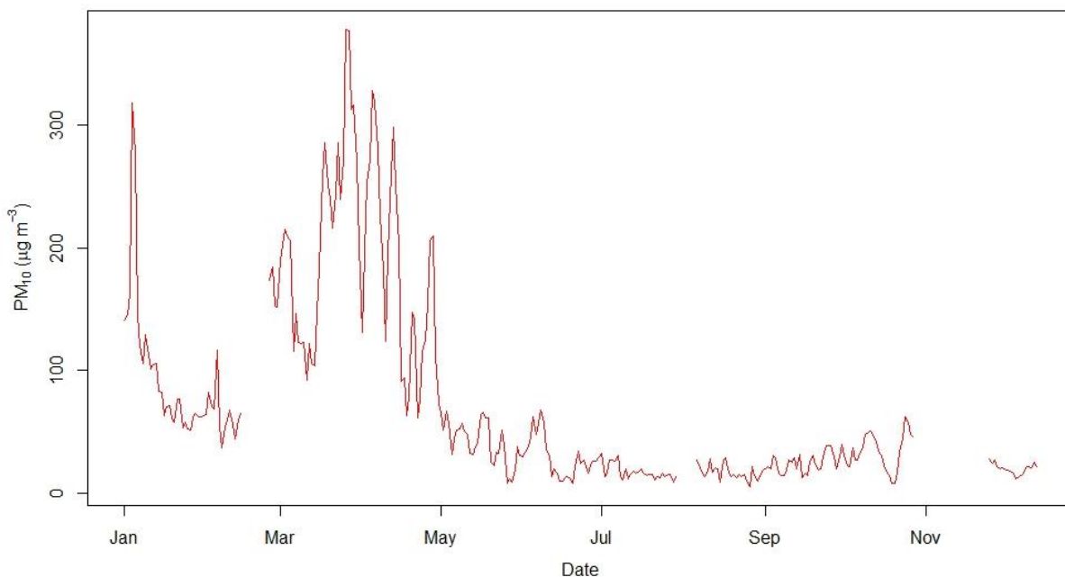
Figure 2.8.12: Daily mean concentration of PM_{10}
