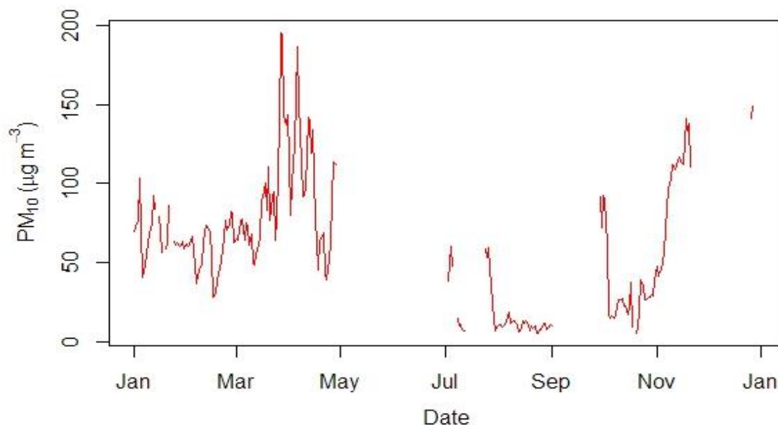
Figure 2.6.12: Daily mean concentration of PM 10
