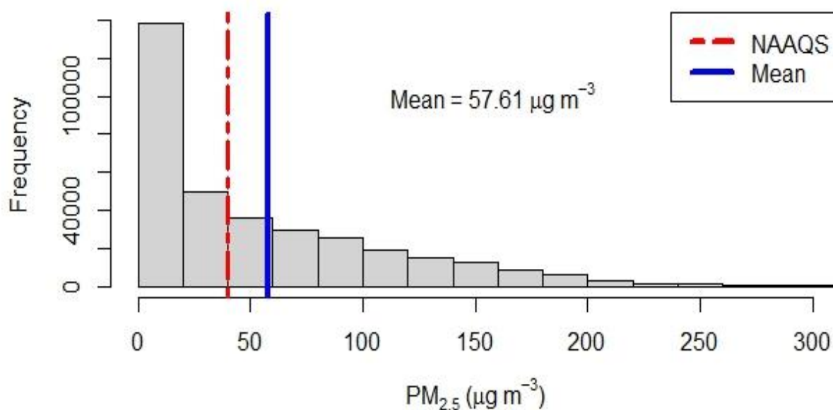
Figure 2.17.1: Histogram of PM 2.5
