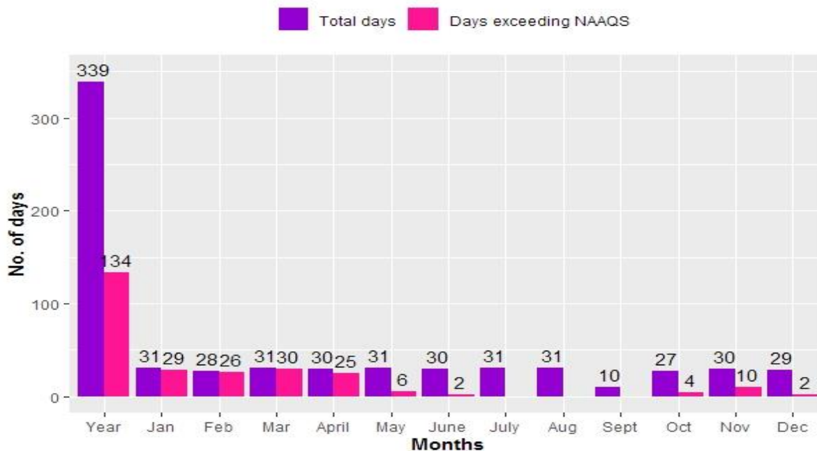
Figure 2.16.8: Compliance status of PM 2.5
