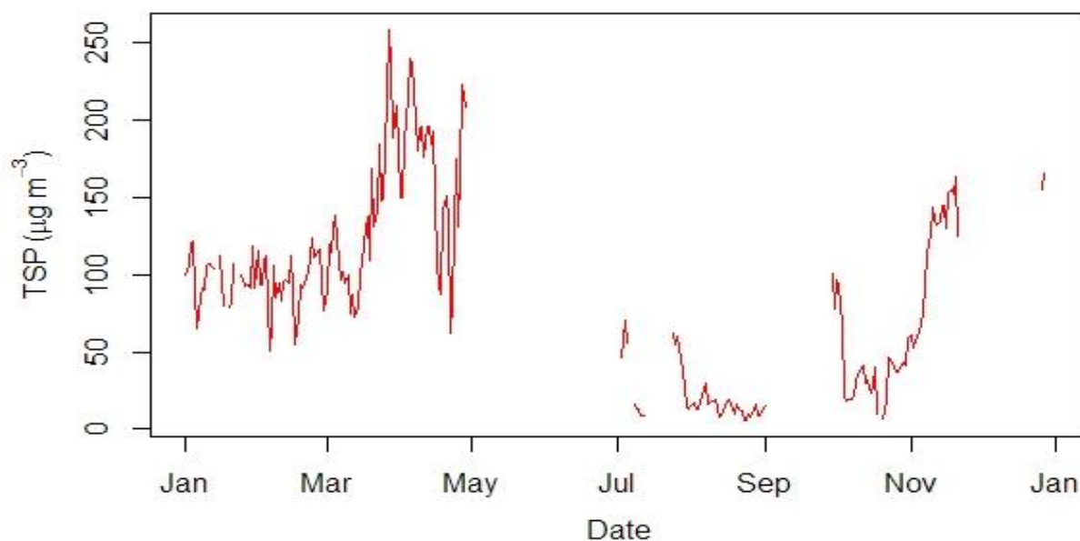
Figure 2.6.20: Daily mean concentration of TSP
