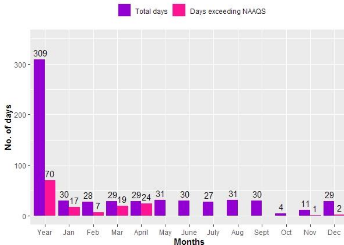
Figure 2.10.24: Compliance status of TSP
