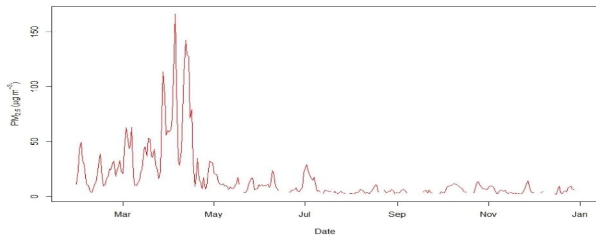
Figure 2.3.4: Daily mean concentration of PM 2.5
