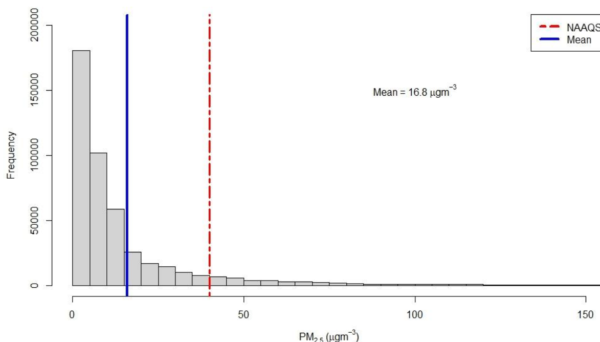
Figure 2.3.1: Histogram of PM 2.5
