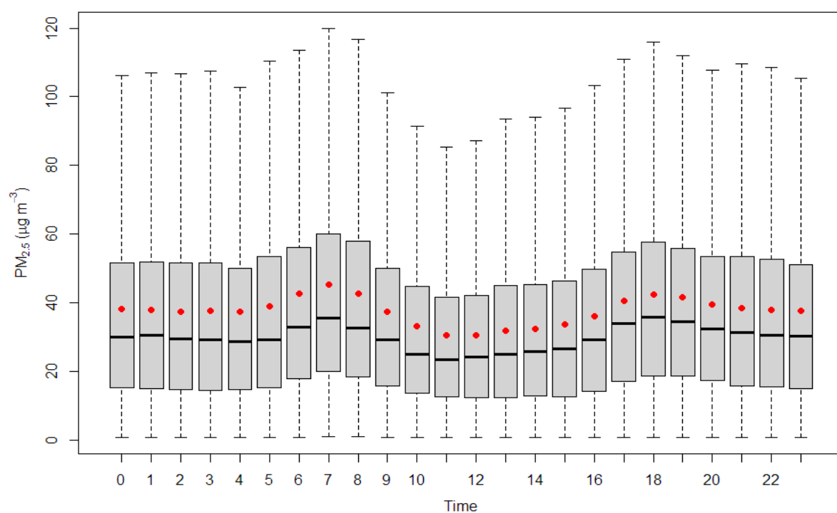
Figure 2.16.3: Diurnal variation of PM 2.5 .
