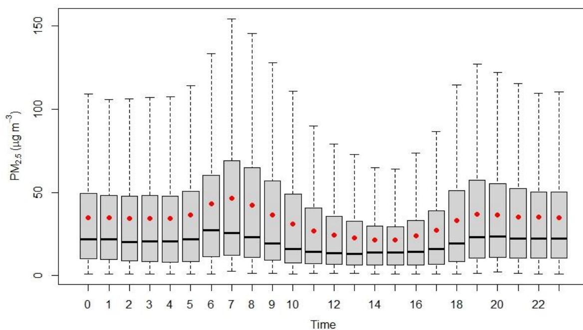
Figure 2.7.3: Diurnal variation of PM 2.5
