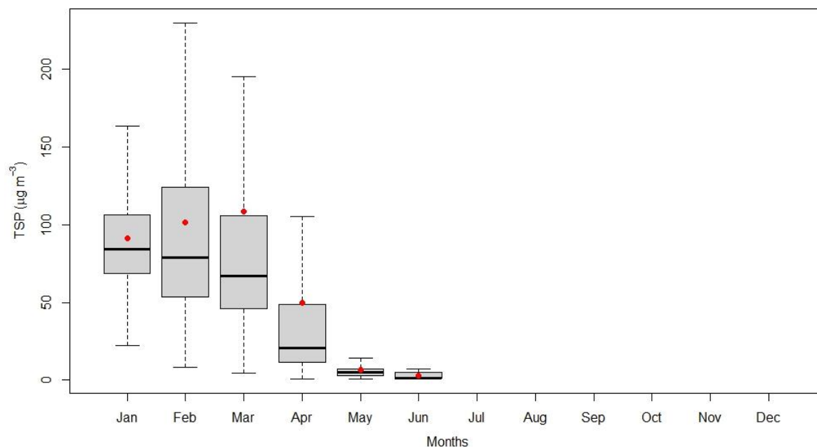
Figure 2.15.19: Monthly variation of TSP
