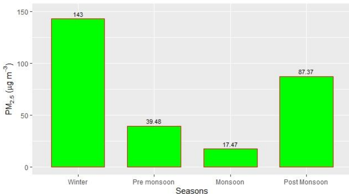
Figure 2.14.7: Seasonal variation of \text{PM}_{2.5}
