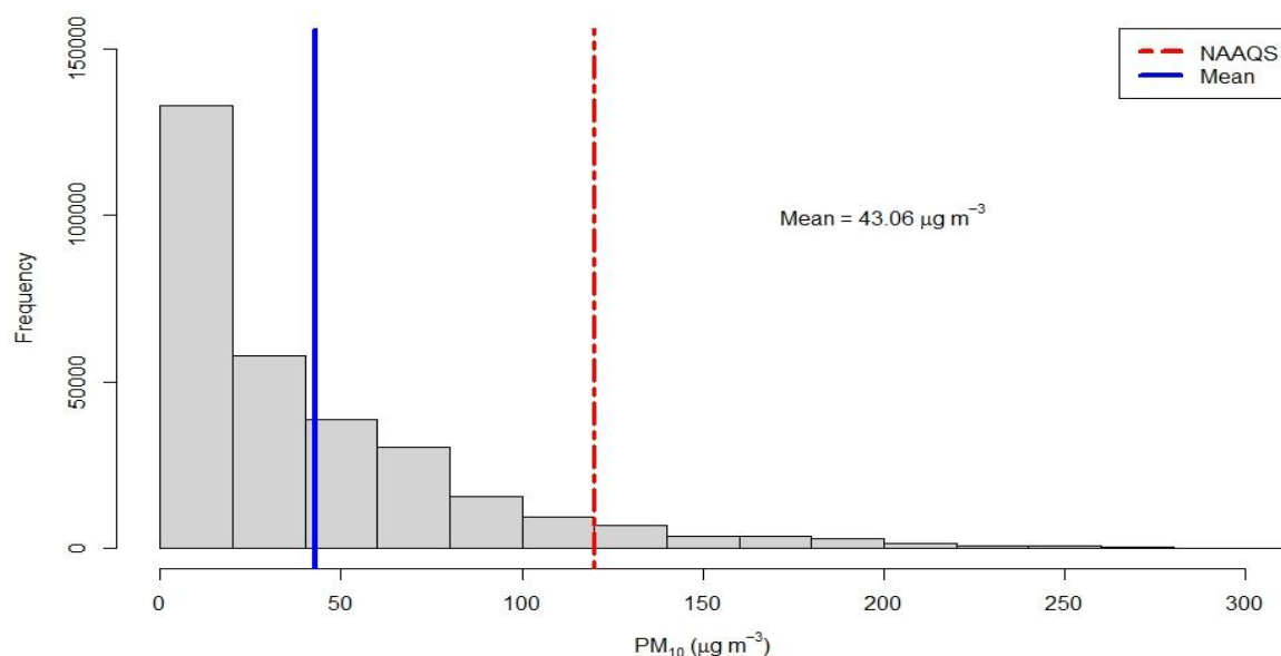
Figure 2.7.9: Histogram of PM 10
