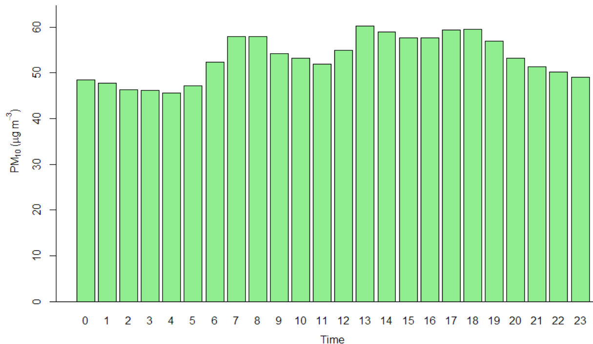
Figure 2.16.10: Hourly average of PM 10
