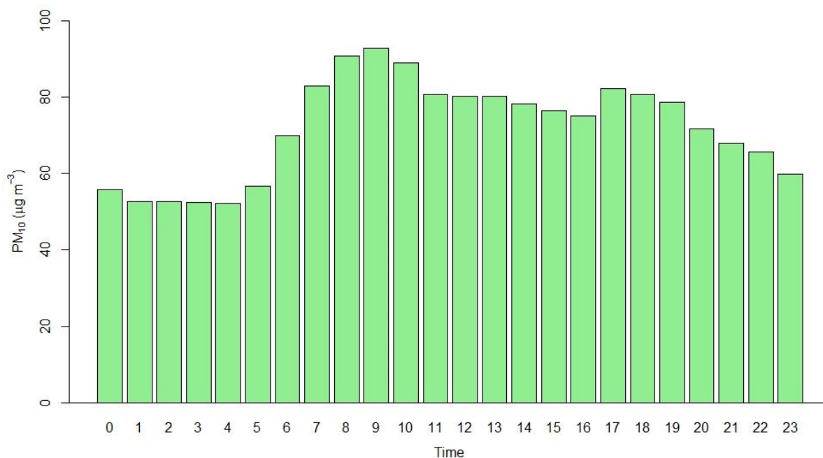
Figure 2.8.10: Hourly average of PM 10
