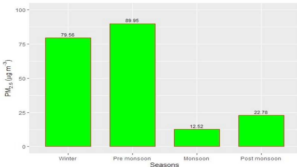
Figure 2.9.7: Seasonal variation of \text{PM}_{2.5}
