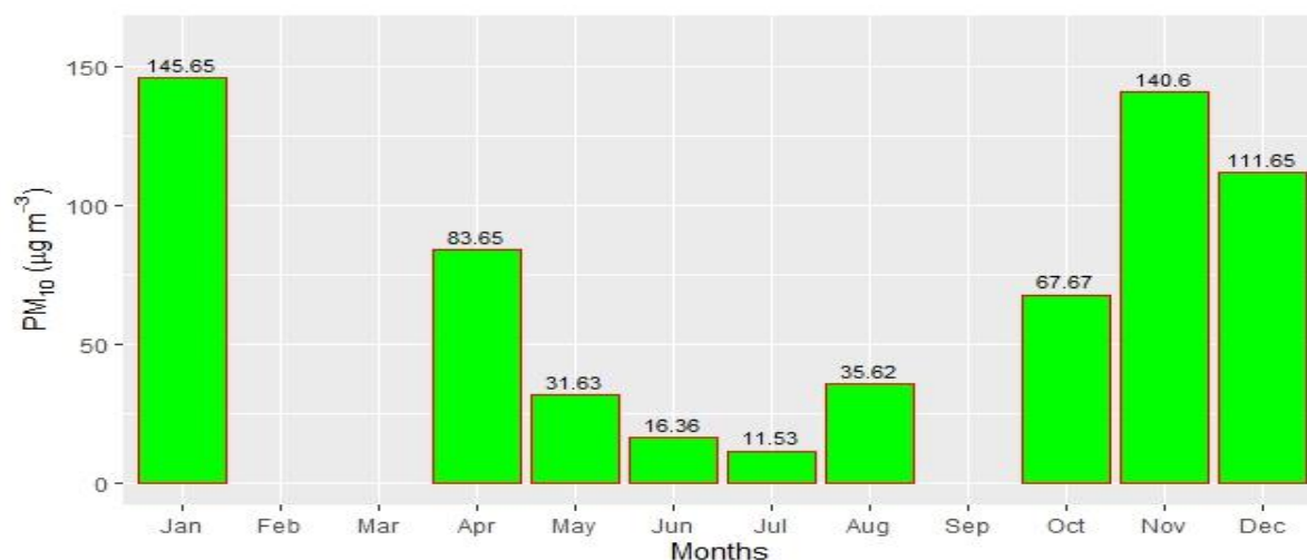
Figure 2.14.13: Monthly average of PM 10
