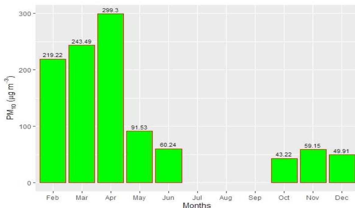
Figure 2.2.14: Monthly average of PM 10
