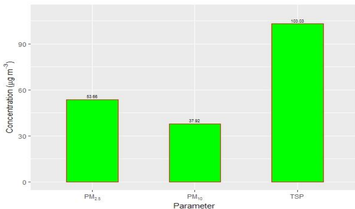
Figure 2.16.25: Annual average of \text{PM}_{2.5} , \text{PM}_{10} and TSP
