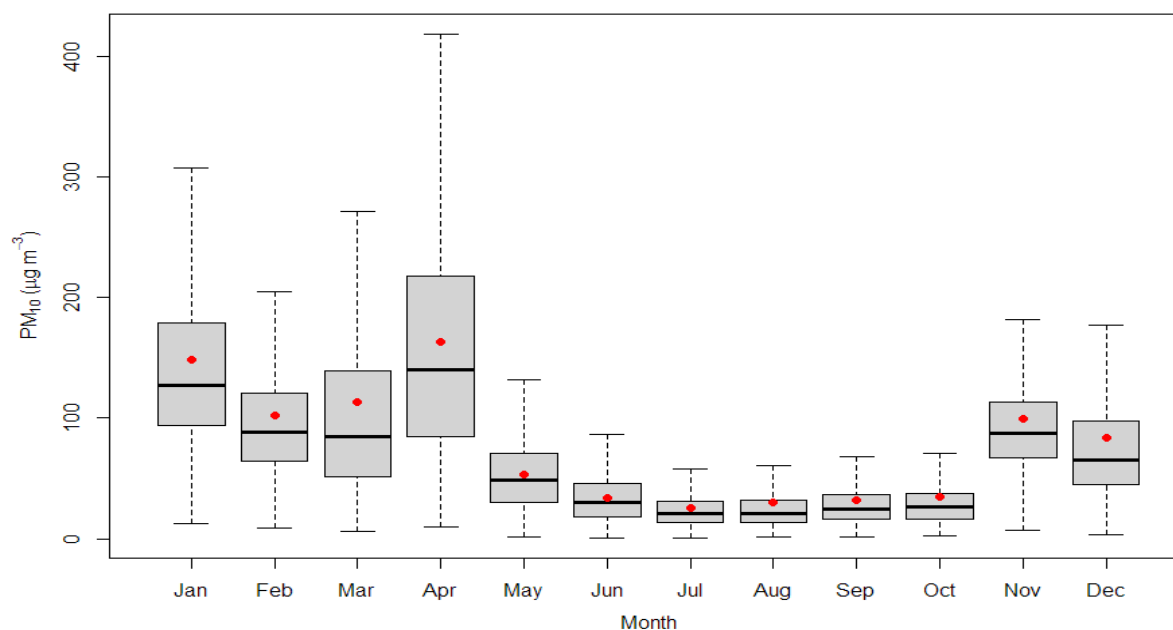
Figure 2.10.13: Monthly variation of PM_{10}
