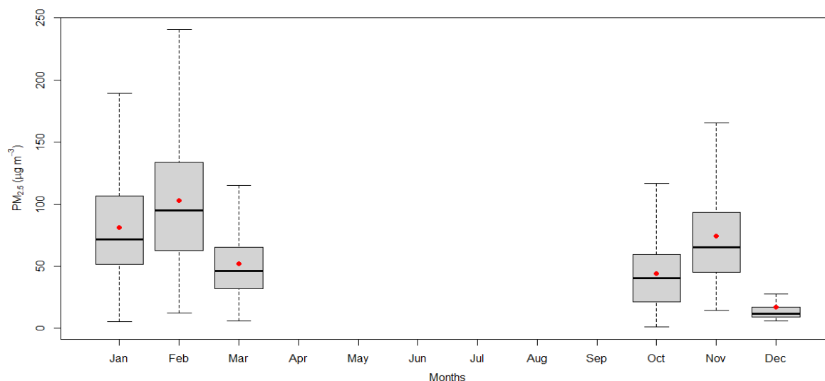
Figure 2.1.6: Monthly variation of PM 2.5
