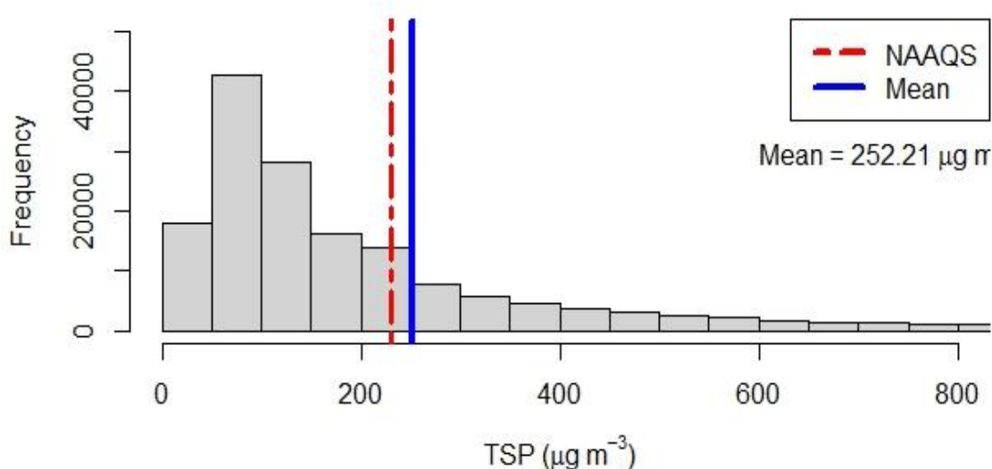
Figure 2.1.17: Histogram of TSP
