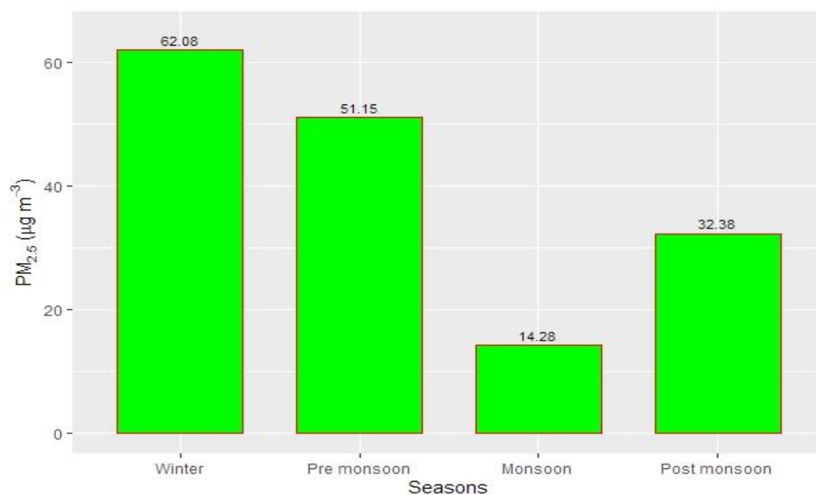
Figure 2.16.7: Seasonal variation of PM 2.5
