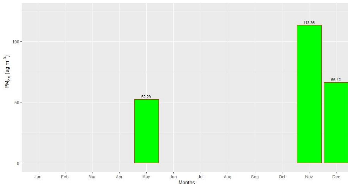
Figure 2.12.6: Monthly average PM 2.5
