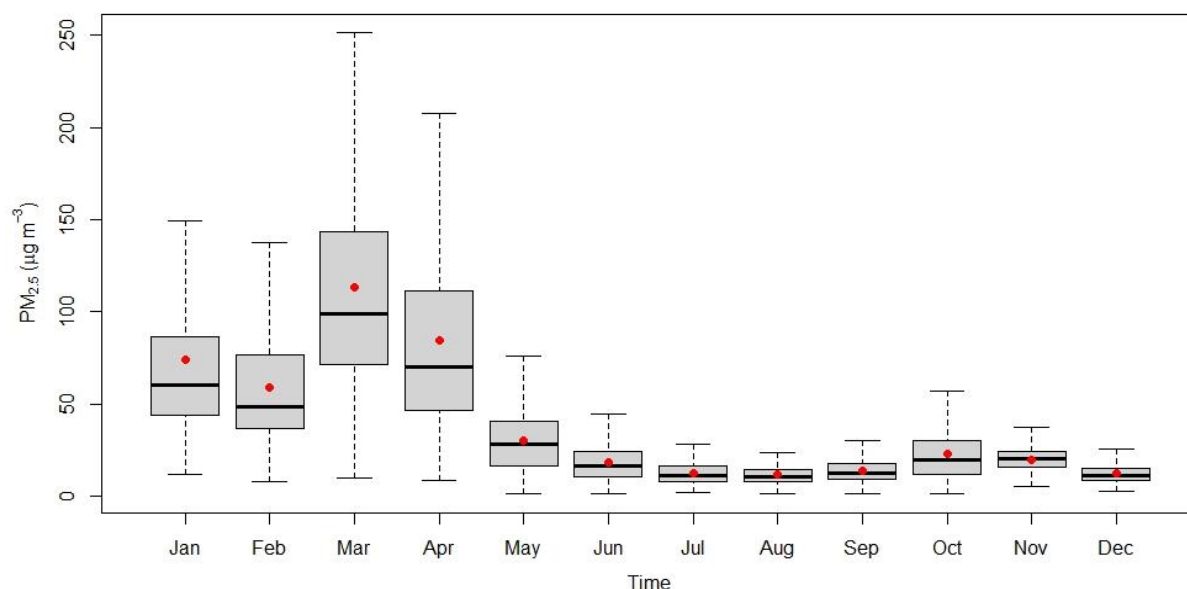
Figure 2.8.5: Monthly variation of PM_{2.5}
