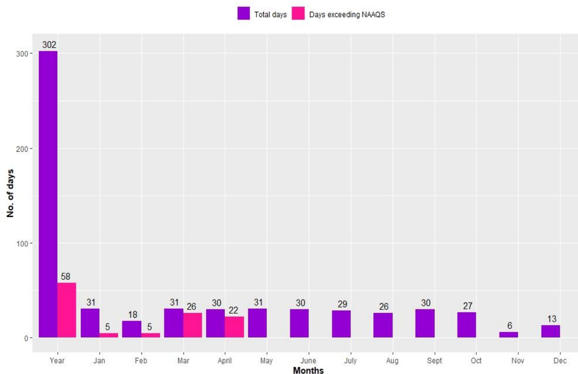
Figure 2.8.24: Compliance status of TSP
