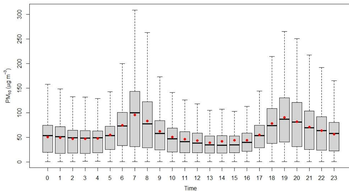
Figure 2.17.11: Diurnal variation of PM 10
