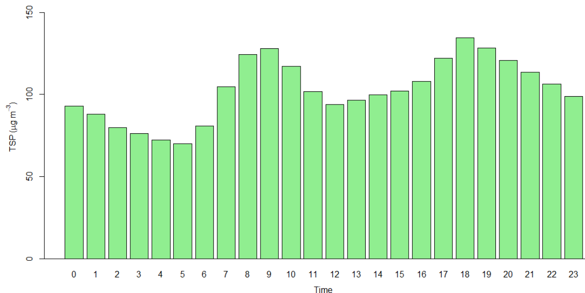
Figure 2.14.18: Hourly average of TSP
