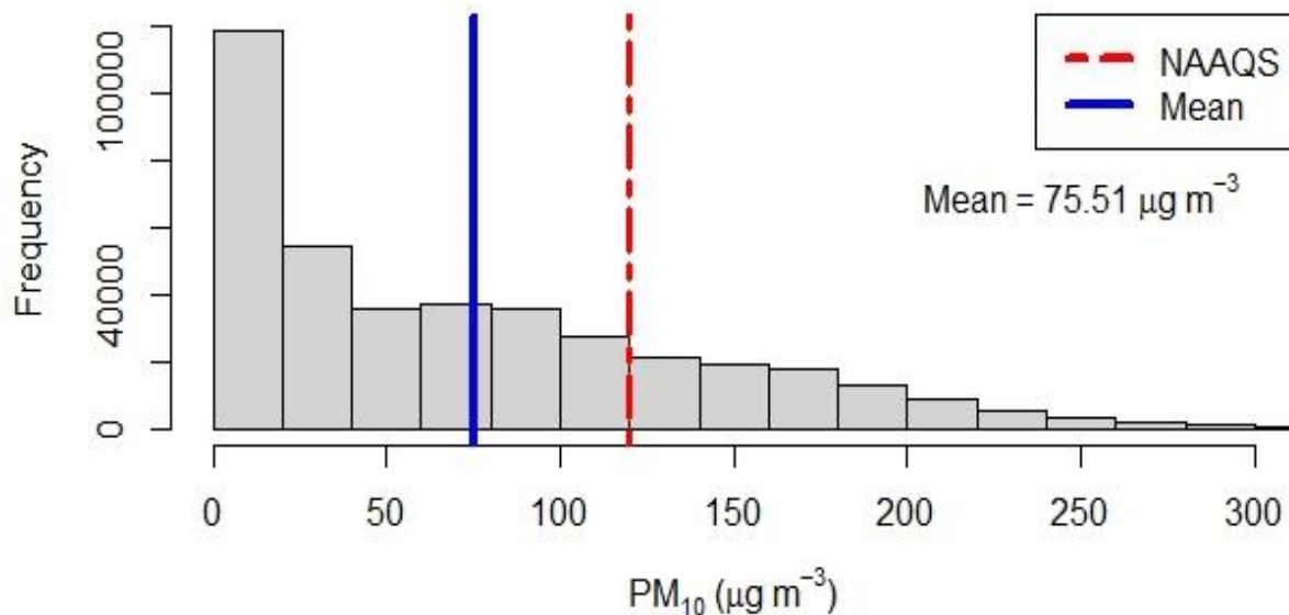
Figure 2.14.9: Histogram of PM 10
