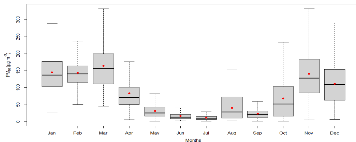
Figure 2.14.14: Monthly variation of PM 10
