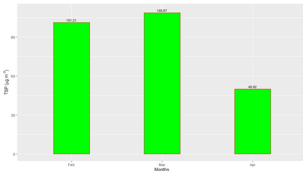
Figure 2.15.20: Monthly average of TSP
