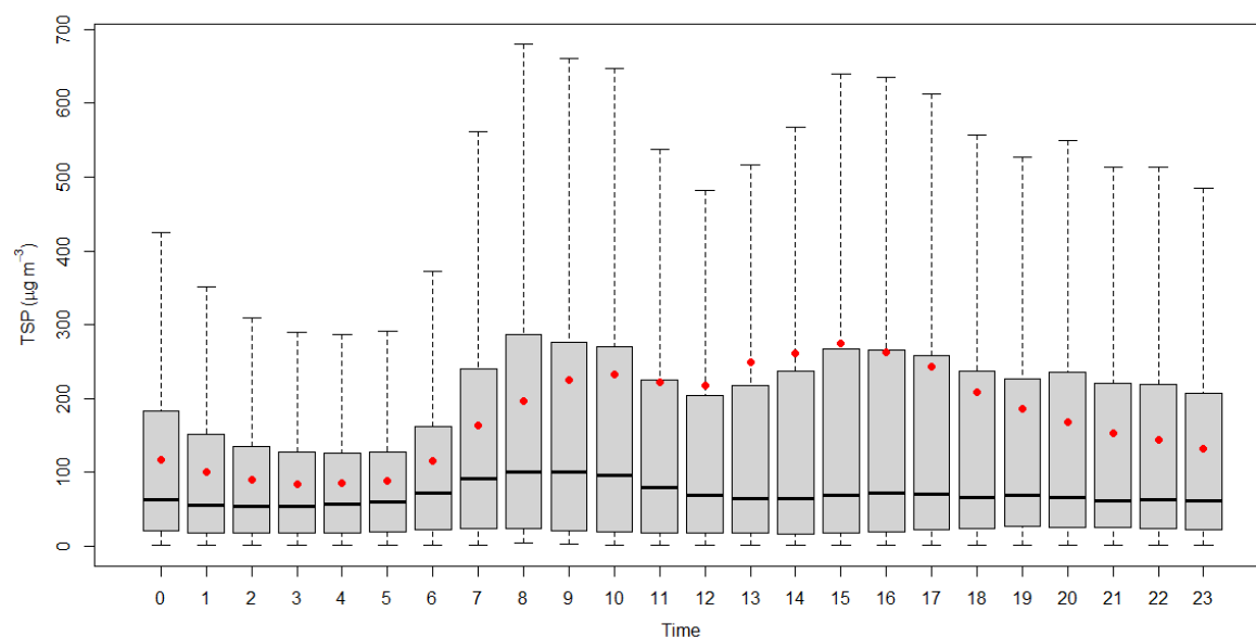
Figure 2.9.19: Diurnal variation of TSP
