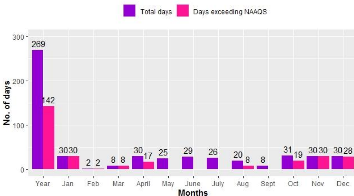
Figure 2.14.8: Compliance status of \text{PM}_{2.5}
