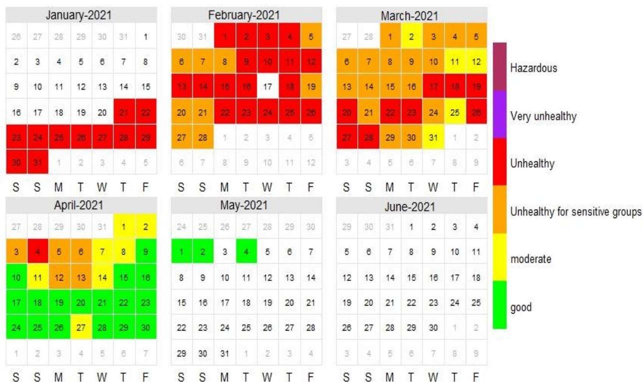
Figure 2.15.22: Calendar plot for PM 2.5 for the year 2021
