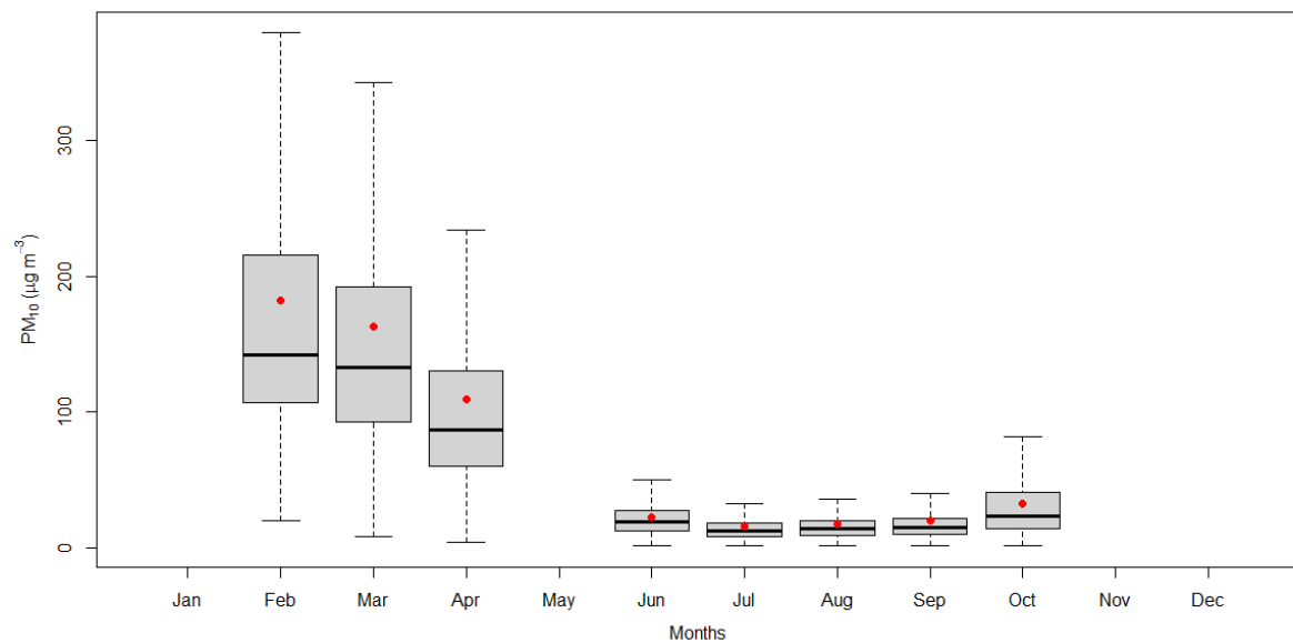
Figure 2.17.13: Monthly variation of PM 10
