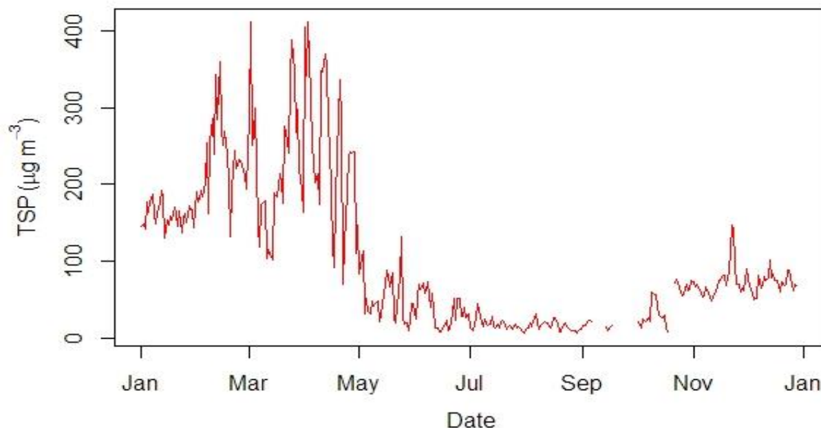
Figure 2.16.20: Daily mean concentration of TSP
