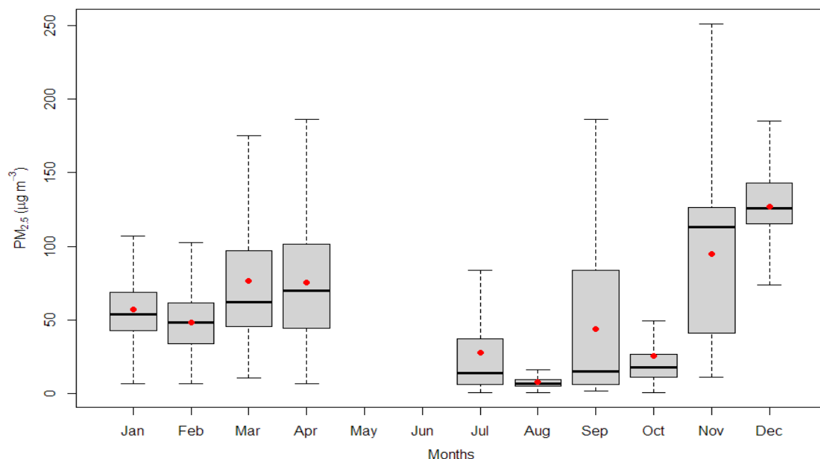
Figure 2.6.5: Monthly variation of PM 2.5
