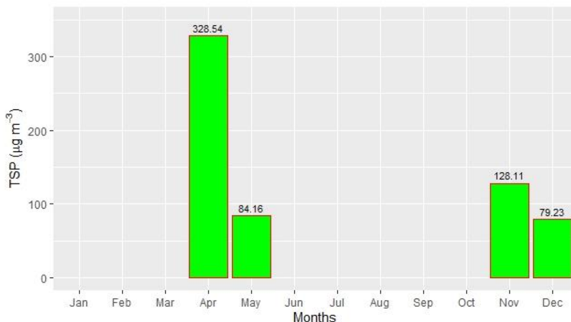
Figure 2.12.20: Monthly average of TSP
