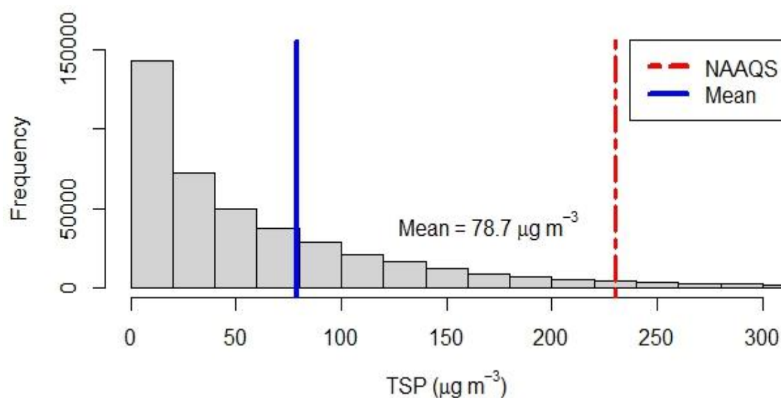
Figure 2.5.17: Histogram of TSP
