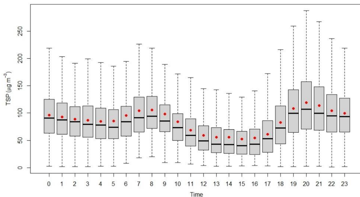
Figure 2.4.19: Diurnal variation of TSP.
