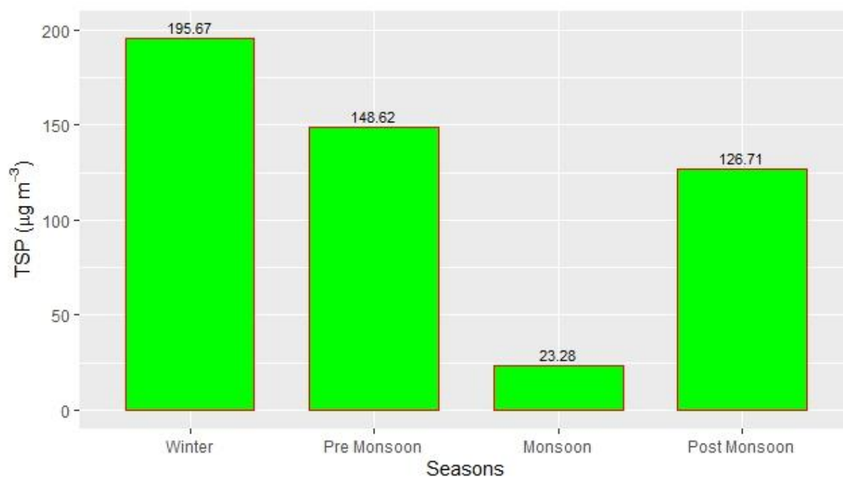
Figure 2.14.23: Seasonal variation of TSP
