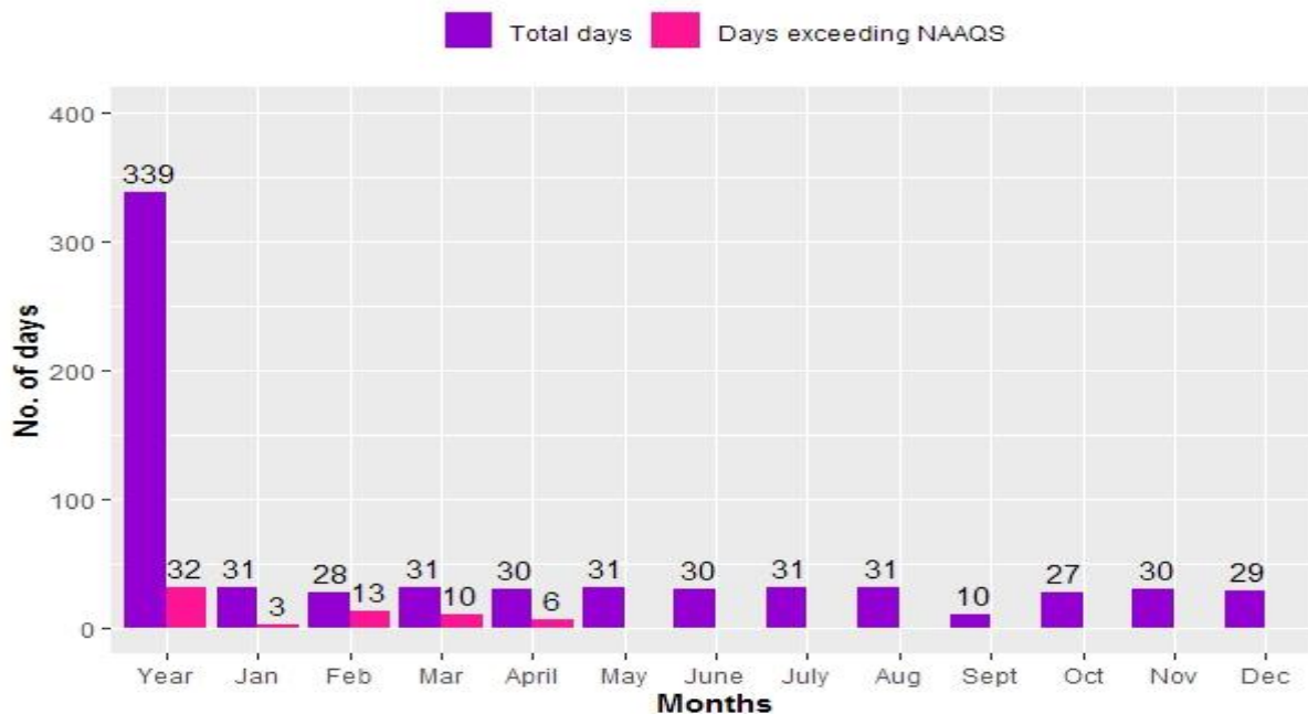
Figure 2.16.16: Compliance status of \text{PM}_{10}
