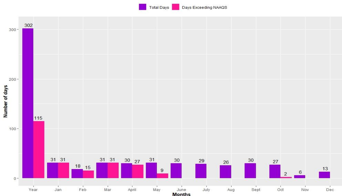
Figure 2.8.8: Compliance status of PM 2.5
