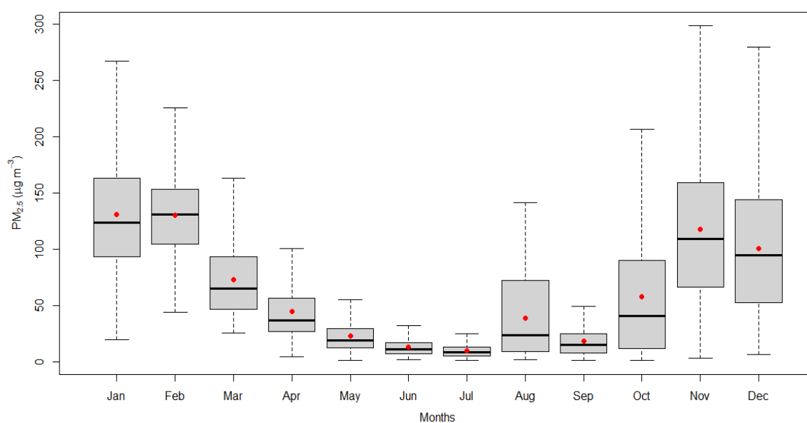
Figure 2.14.6: Monthly variation of PM 2.5
