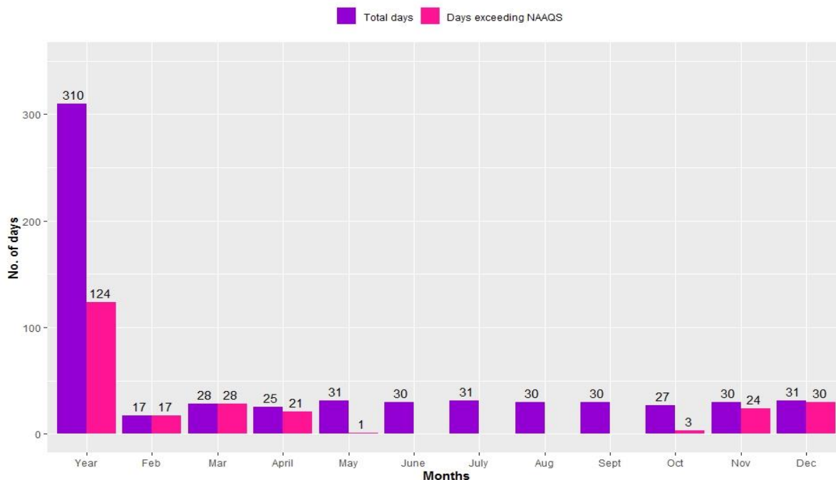
Figure 2.11.8: Compliance status of PM 2.5
