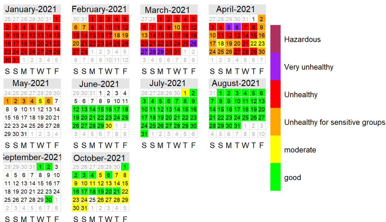
Figure 2.9.25: Calendar plot for PM 2.5 for the year 2021
