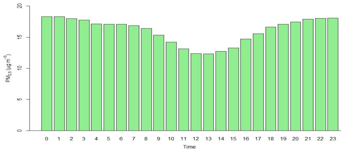
Figure 2.3.2: Hourly average of PM 2.5
