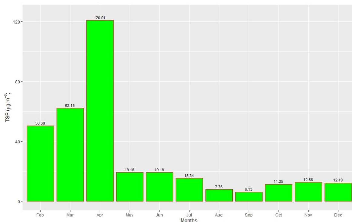
Figure 2.3.22: Monthly average of TSP
