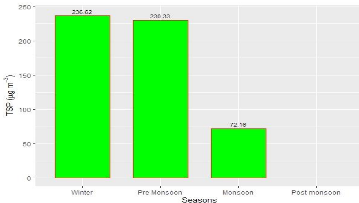
Figure 2.10.23: Seasonal variation of TSP
