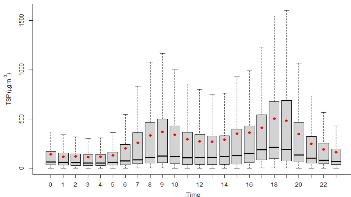
Figure 2.2.19: Diurnal variation of TSP.
