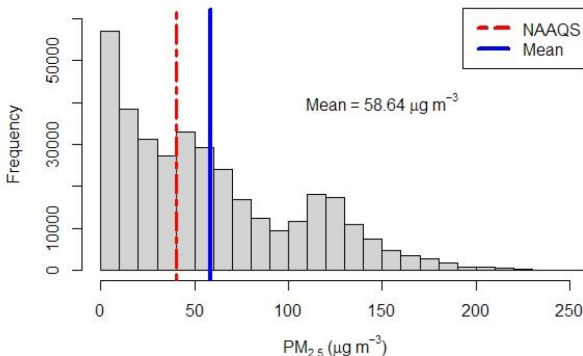
Figure 2.6.1: Histogram of PM 2.5
