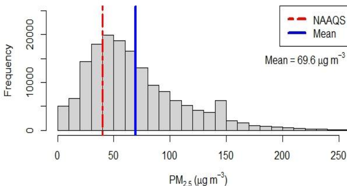
Figure 2.1.1: Histogram of PM 2.5
