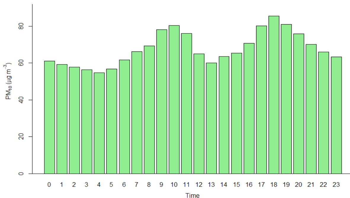
Figure 2.6.10: Hourly average of PM 10 .
