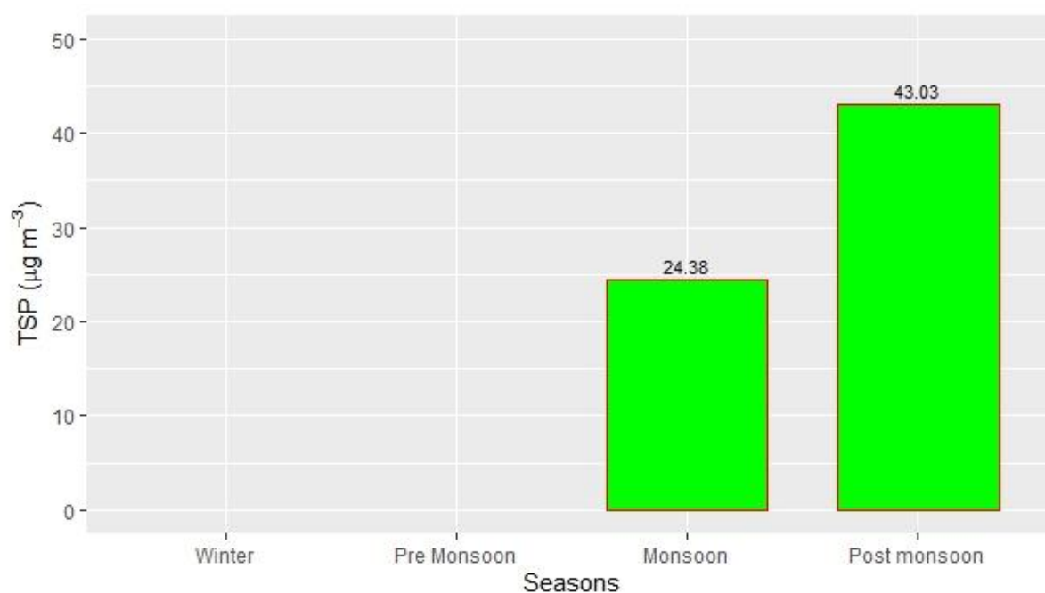
Figure 2.17.23: Seasonal variation of TSP
