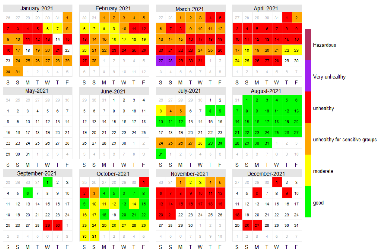
Figure 2.6.25: Calendar plot for PM 2.5 for the year 2021
