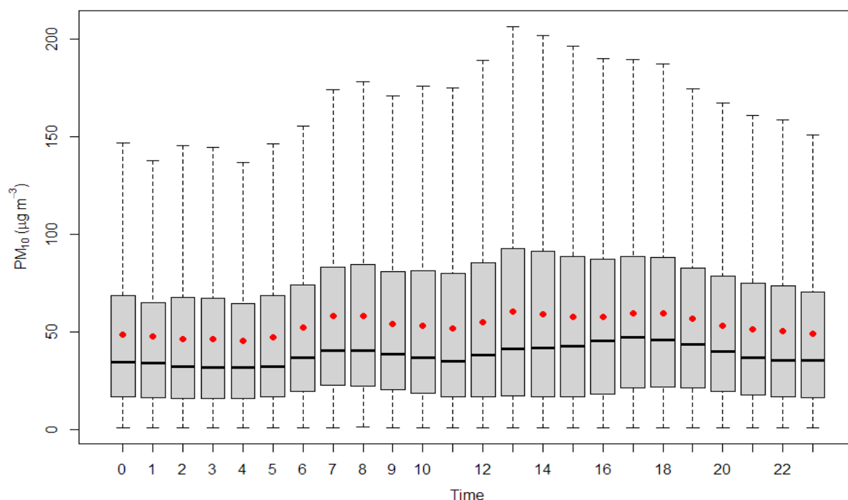
Figure 2.16.11: Diurnal variation of PM 10
