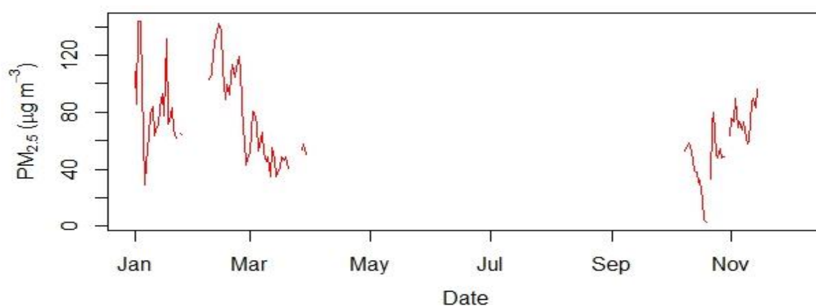
Figure 2.1.4: Daily mean concentration of PM 2.5
