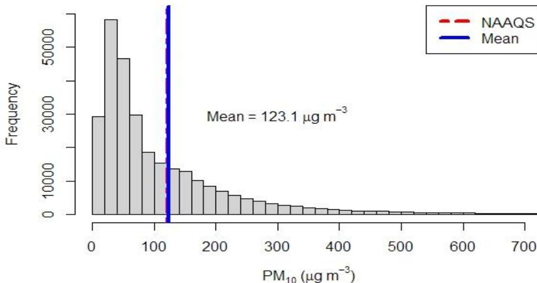
Figure 2.2.9: Histogram of PM 10
