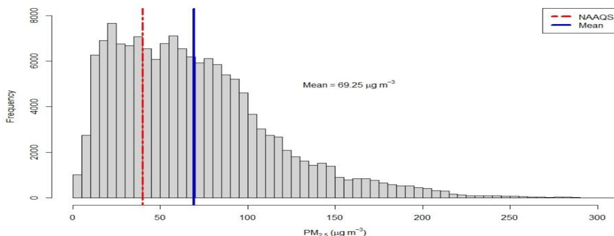
Figure 2.4.1: Histogram of PM 2.5
