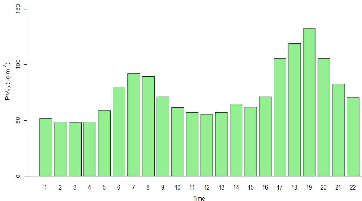
Figure 2.17.10: Hourly average of PM 10 .
