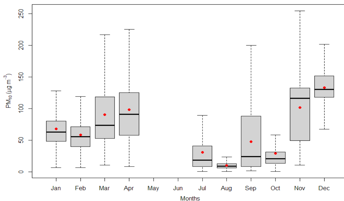
Figure 2.6.13: Monthly variation of PM 10
