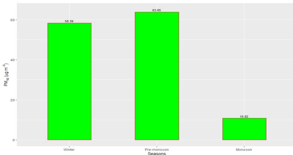
Figure 2.7.15: Seasonal variation of PM 10
