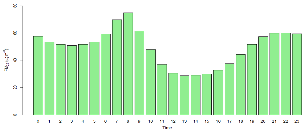
Figure 2.9.2: Hourly average of PM 2.5 .
