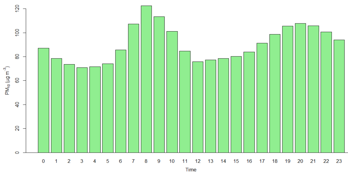
Figure 2.9.10: Hourly average of PM 10
