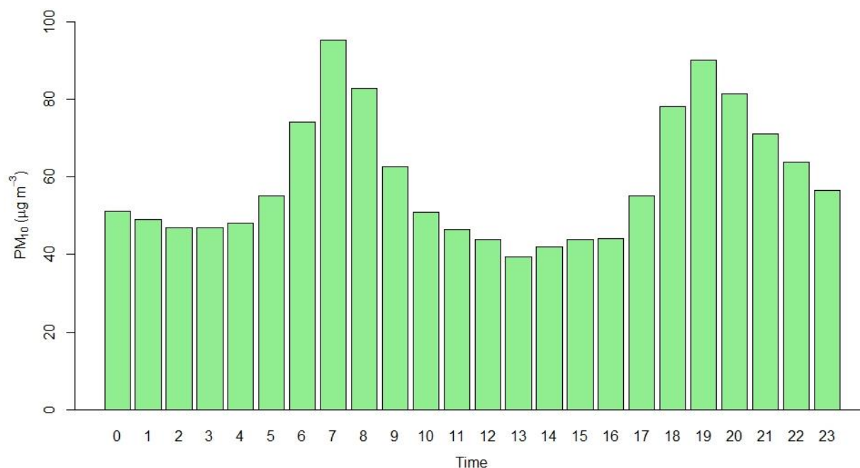
Figure 2.15.9: Hourly average of PM 10
