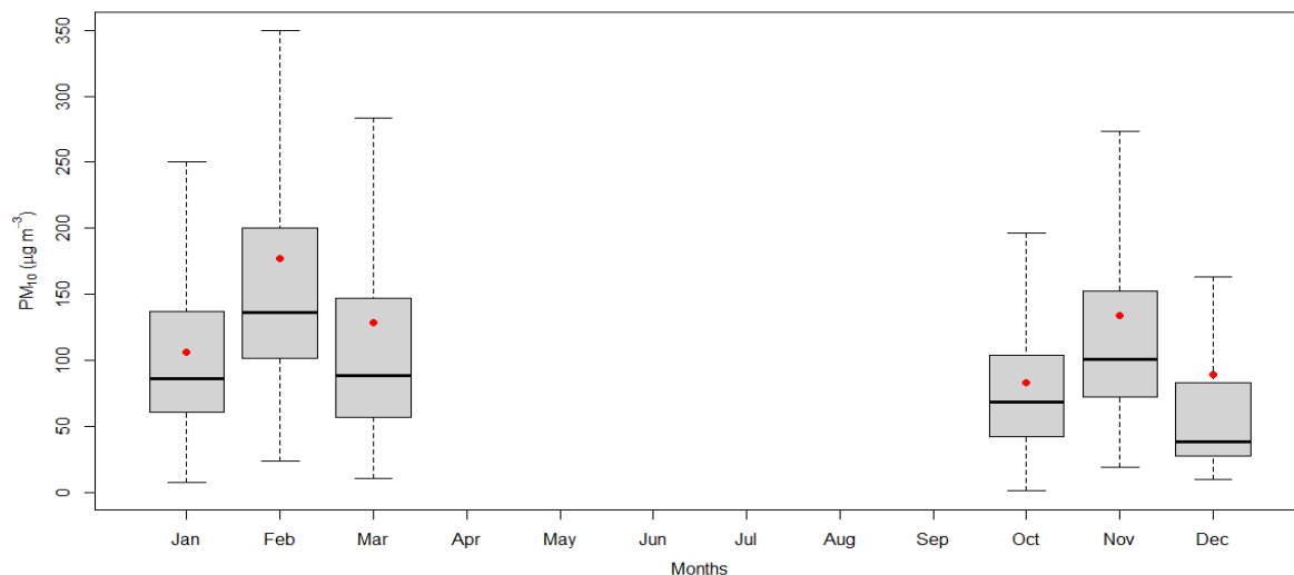
Figure 2.1.14: Monthly variation of PM 10
