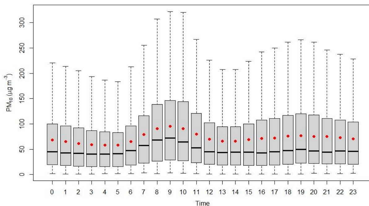
Figure 2.11.11: Diurnal variation of PM 10
