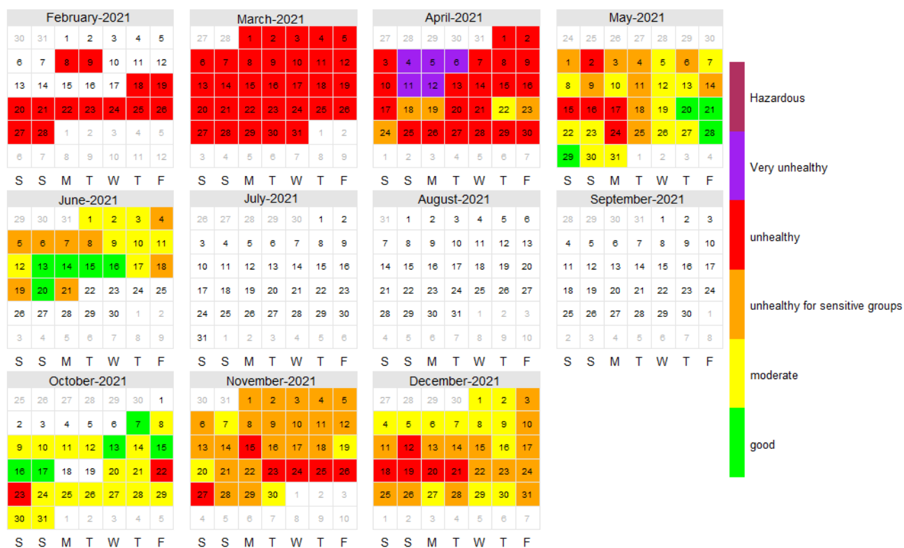
Figure 2.2.25: Calendar plot for PM 2.5 for the year 2021
