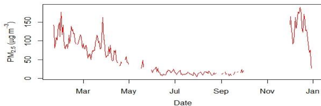
Figure 2.17.4: Daily mean concentration of PM 2.5
