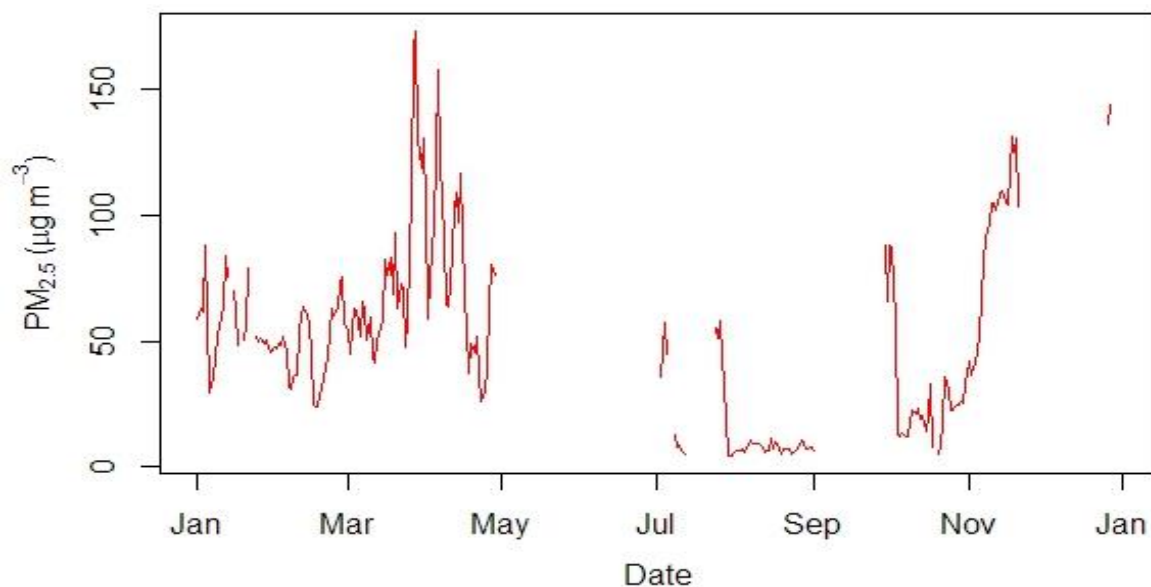
Figure 2.6.4: Daily mean concentration of PM 2.5
