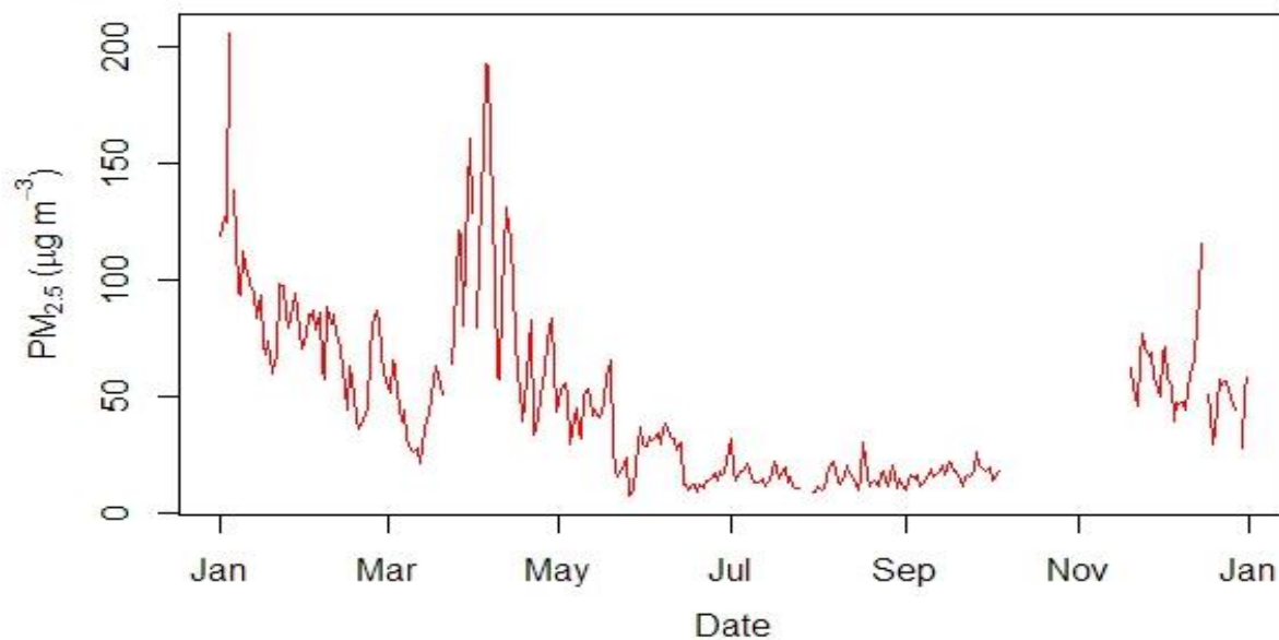
Figure 2.10.4: Daily mean concentration of PM 2.5
