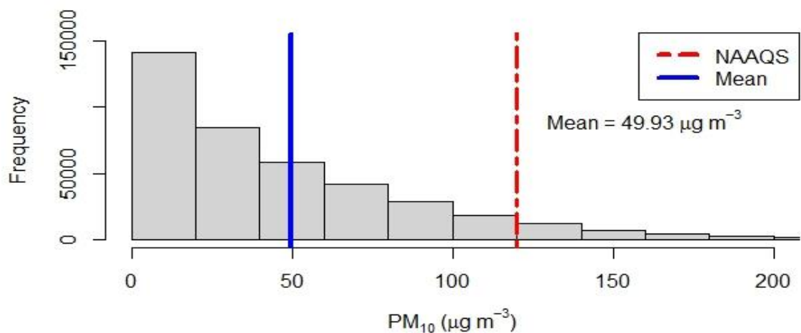
Figure 2.5.9: Histogram of PM 10
