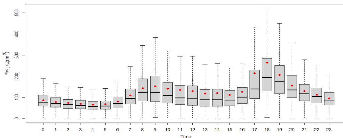
Figure 2.1.11: Diurnal variation of PM 10
