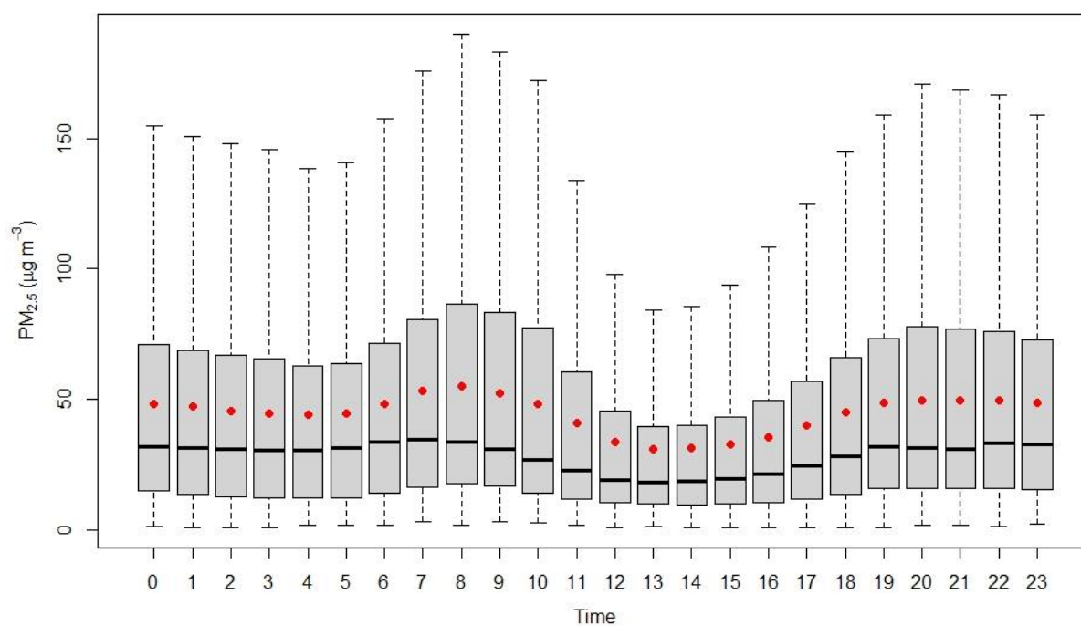
Figure 2.11.3: Diurnal variation of PM 2.5
