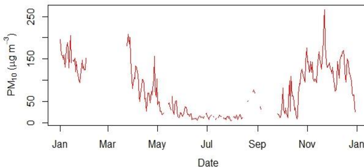
Figure 2.14.12: Daily mean concentration of PM 10
