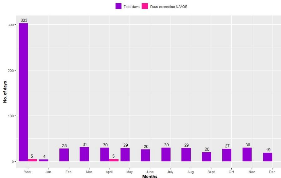
Figure 2.3.24: Compliance status of TSP
