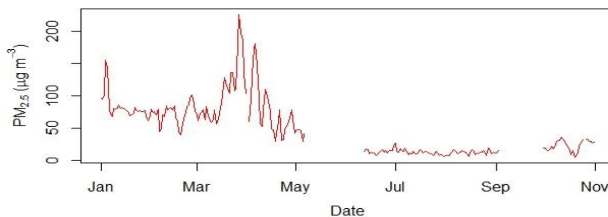
Figure 2.9.4: Daily mean concentration of PM 2.5
