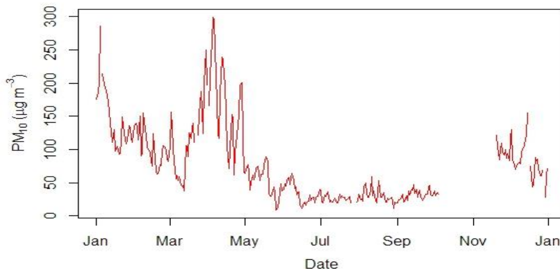
Figure 2.10.12: Daily mean concentration of PM_{10}
