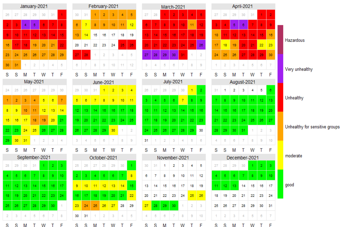
Figure 2.8.26: Calendar plot for PM 2.5 for the year 2021
