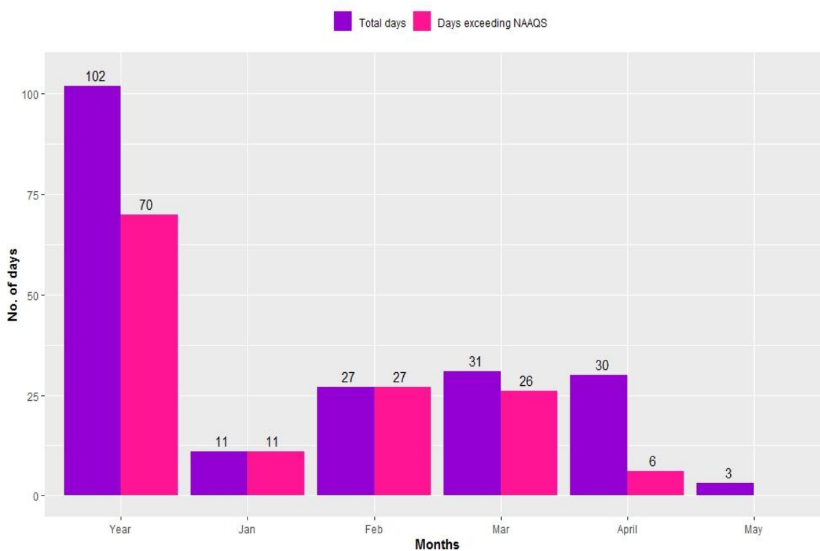
Figure 2.15.7: Compliance status of PM 2.5
