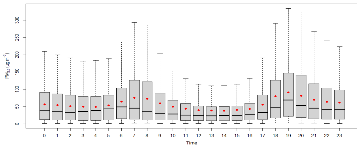
Figure 2.17.3: Diurnal variation of PM 2.5
