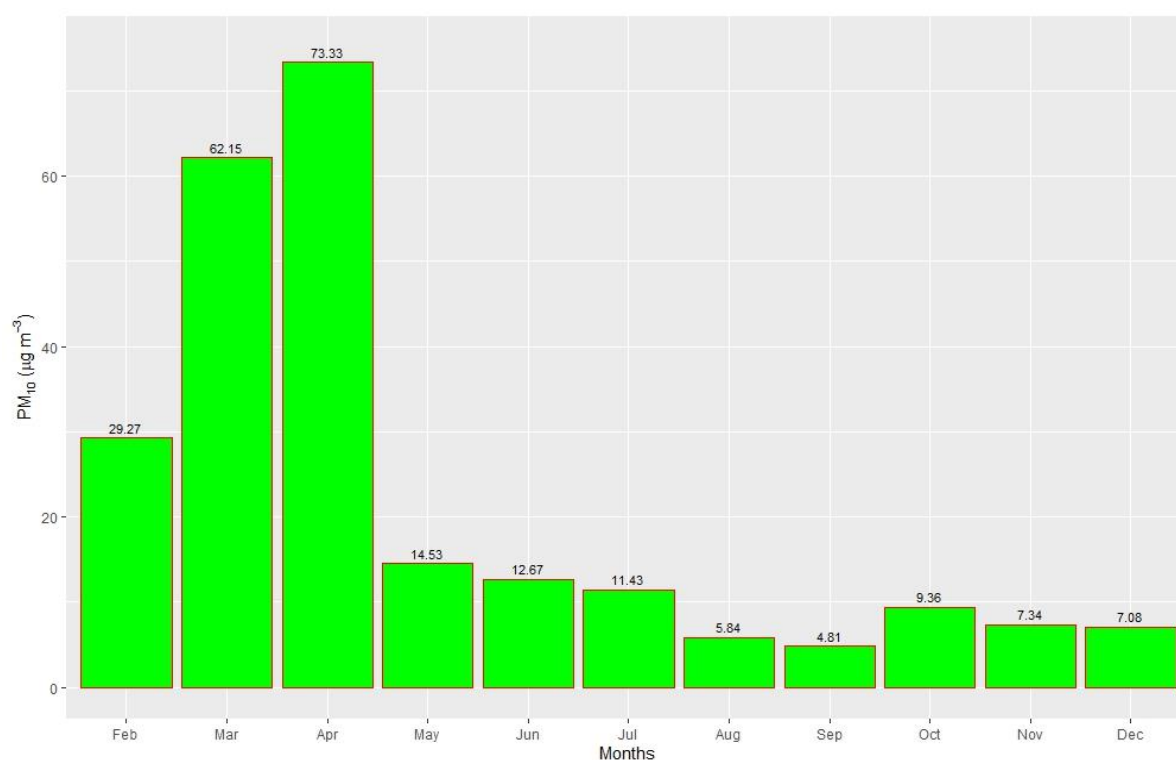
Figure 2.3.14: Monthly average of PM 10
