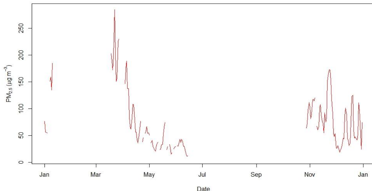
Figure 2.12.4: Daily mean concentration of PM 2.5
