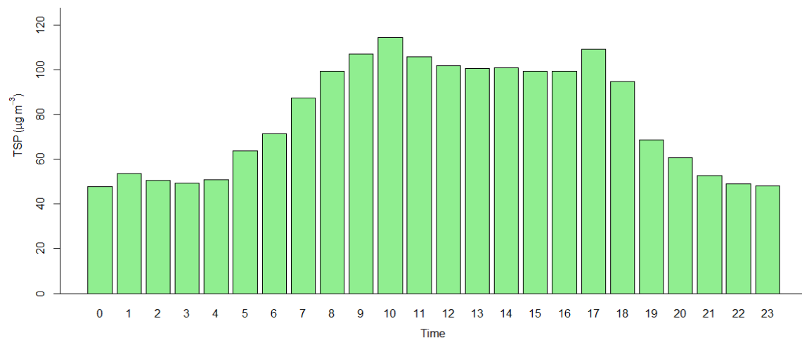
Figure 2.5.18: Hourly average of TSP
