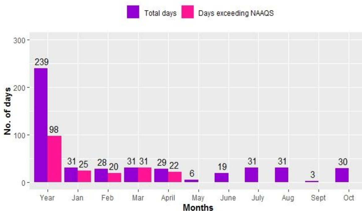
Figure 2.9.24: Compliance status of TSP
