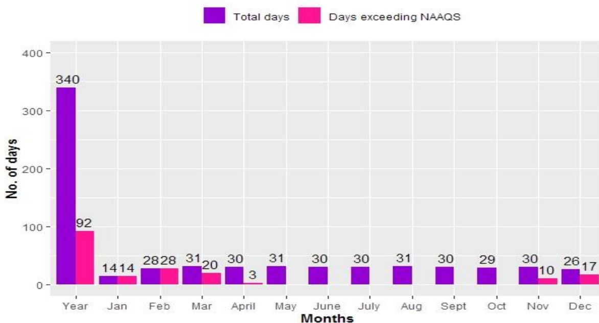
Figure 2.13.8: Compliance status of PM 2.5
