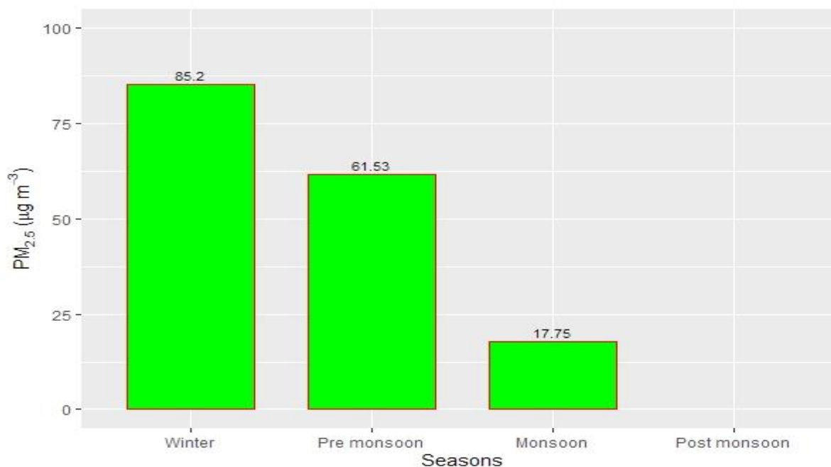
Figure 2.10.7: Seasonal variation of PM 2.5
