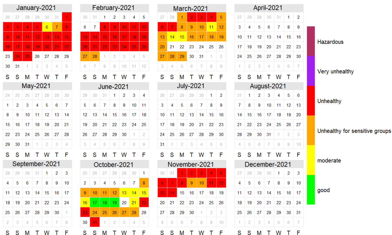
Figure 2.1.25: Calendar plot for PM 2.5 for the year 2021
