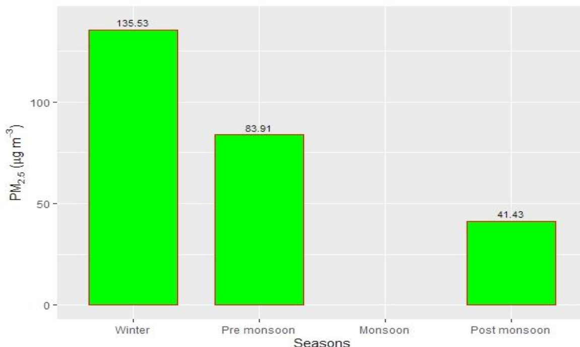
Figure 2.2.7: Seasonal variation of PM 2.5
