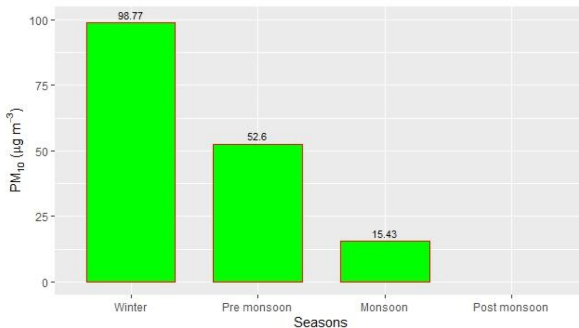
Figure 2.5.15: Seasonal variation of PM 10
