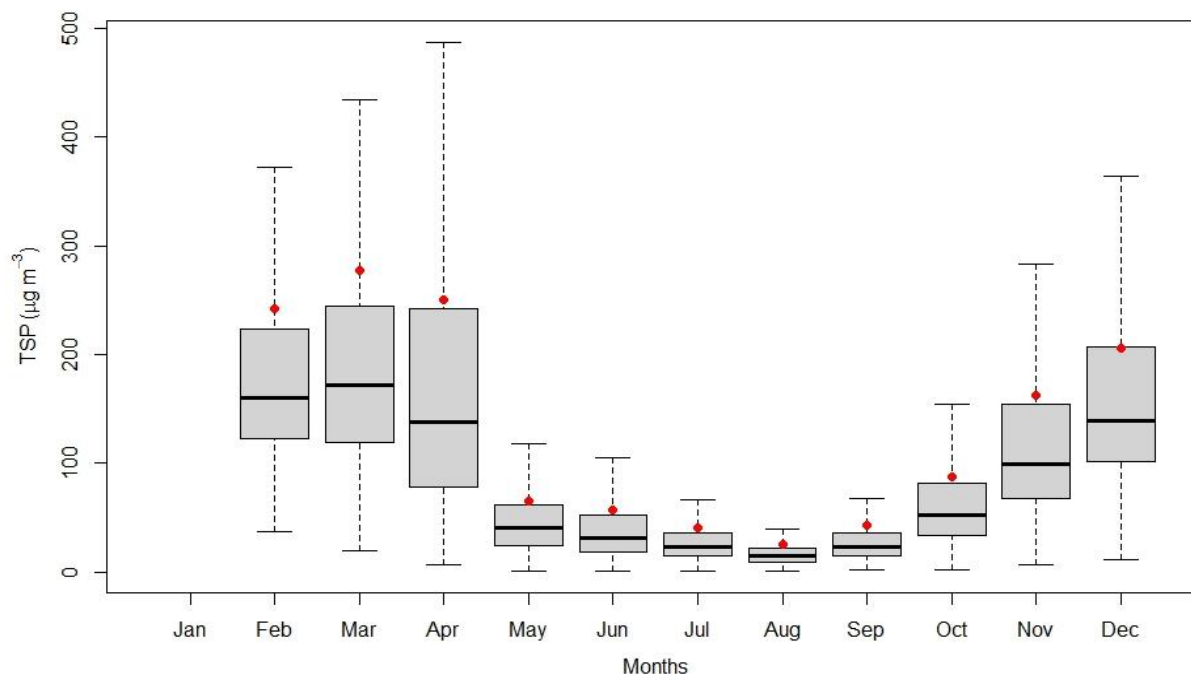
Figure 2.11.21: Monthly variation of TSP
