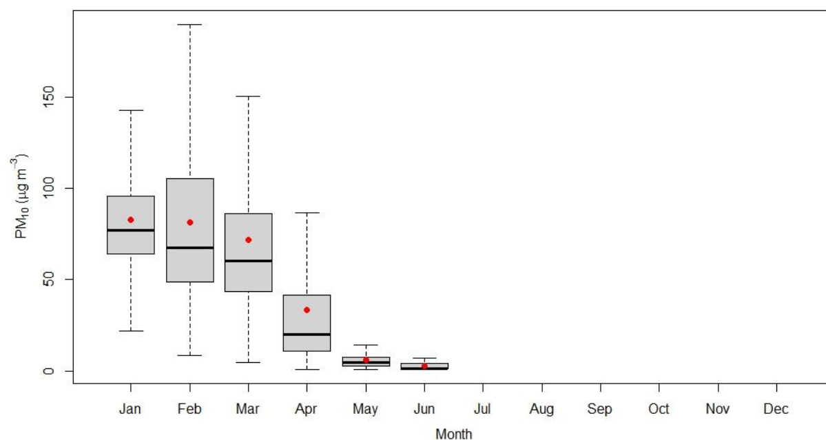
Figure 2.15.12: Monthly variation of PM 10
