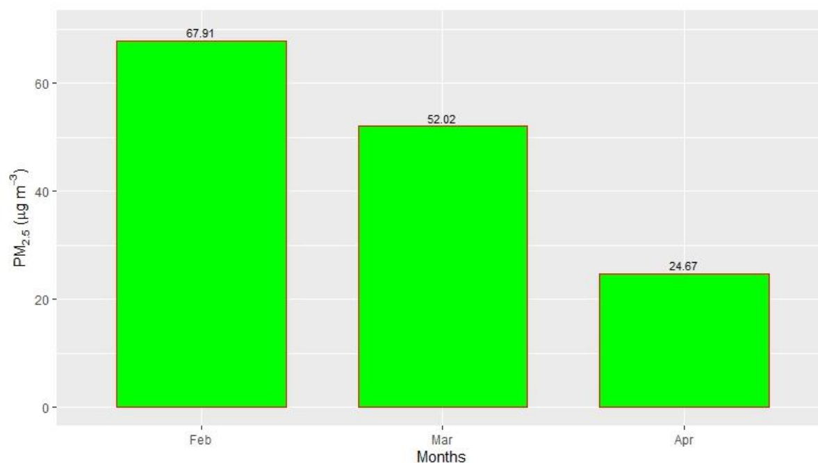
Figure 2.15.6: Monthly average PM 2.5
