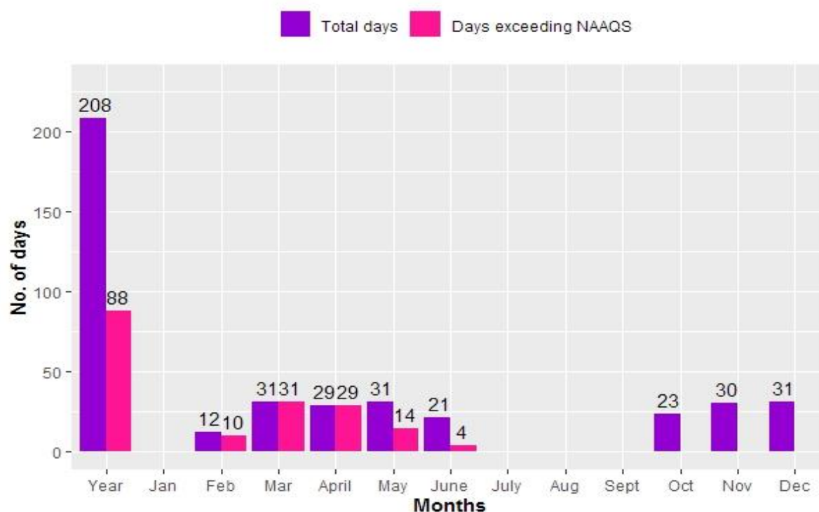
Figure 2.2.24: Compliance status of TSP
