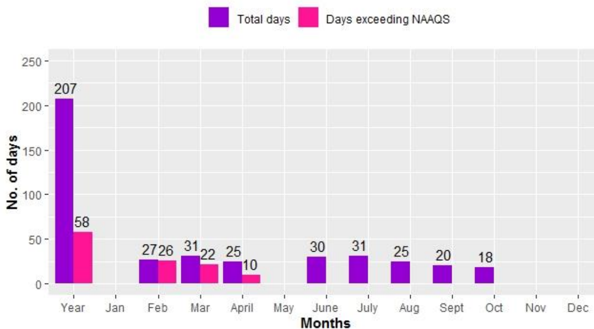
Figure 2.17.16: Compliance status of PM 10
