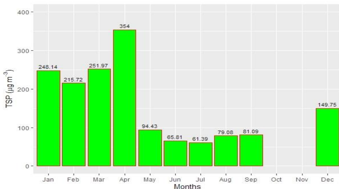
Figure 2.10.22: Monthly average of TSP
