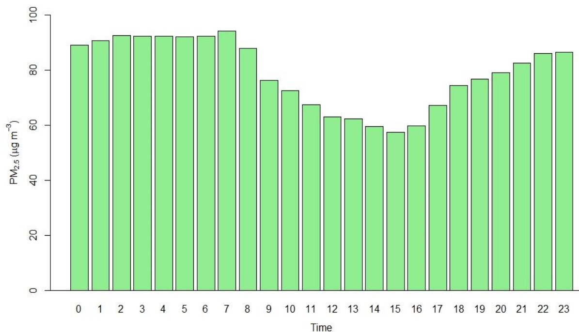
Figure 2.12.2: Hourly average of PM 2.5
