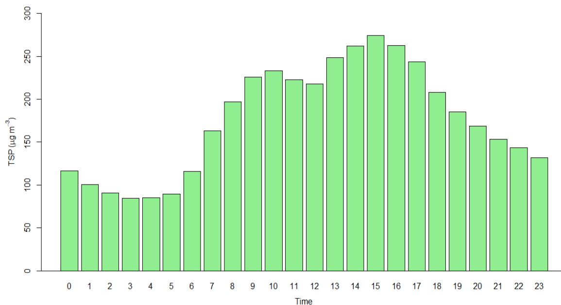
Figure 2.9.18: Hourly average of TSP
