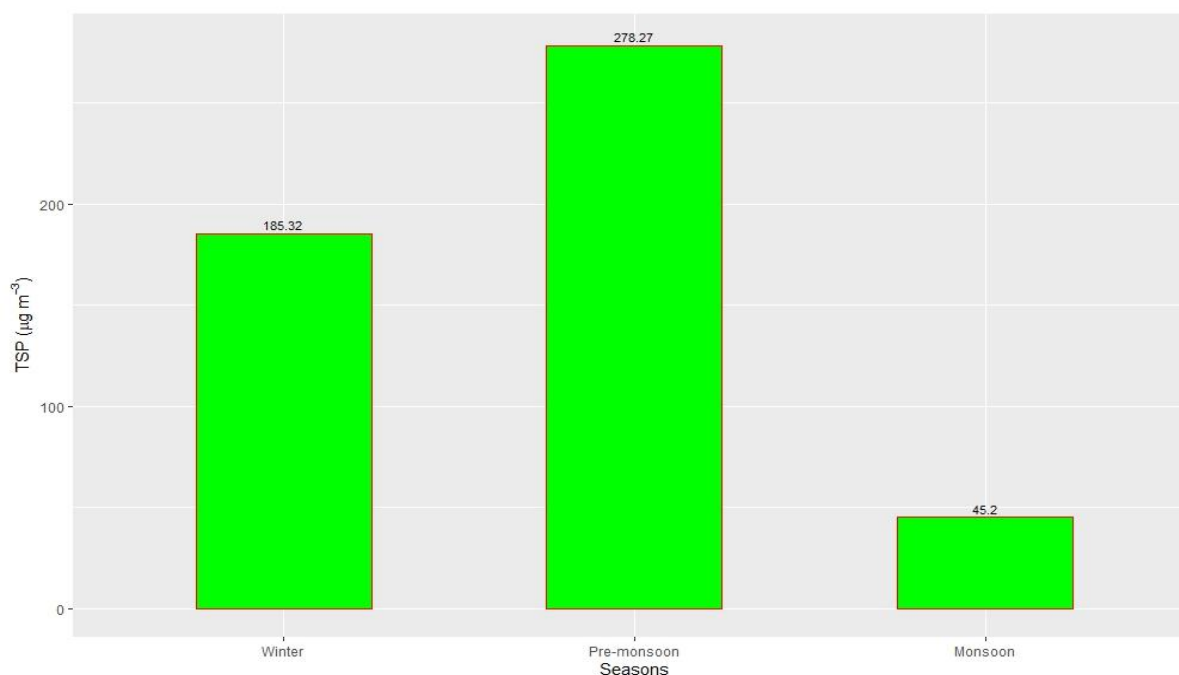
Figure 2.8.23: Seasonal variation of TSP
