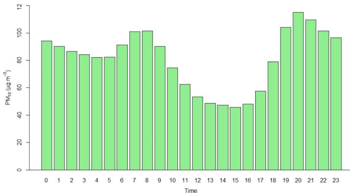
Figure 2.4.10: Hourly average of PM 10 .
