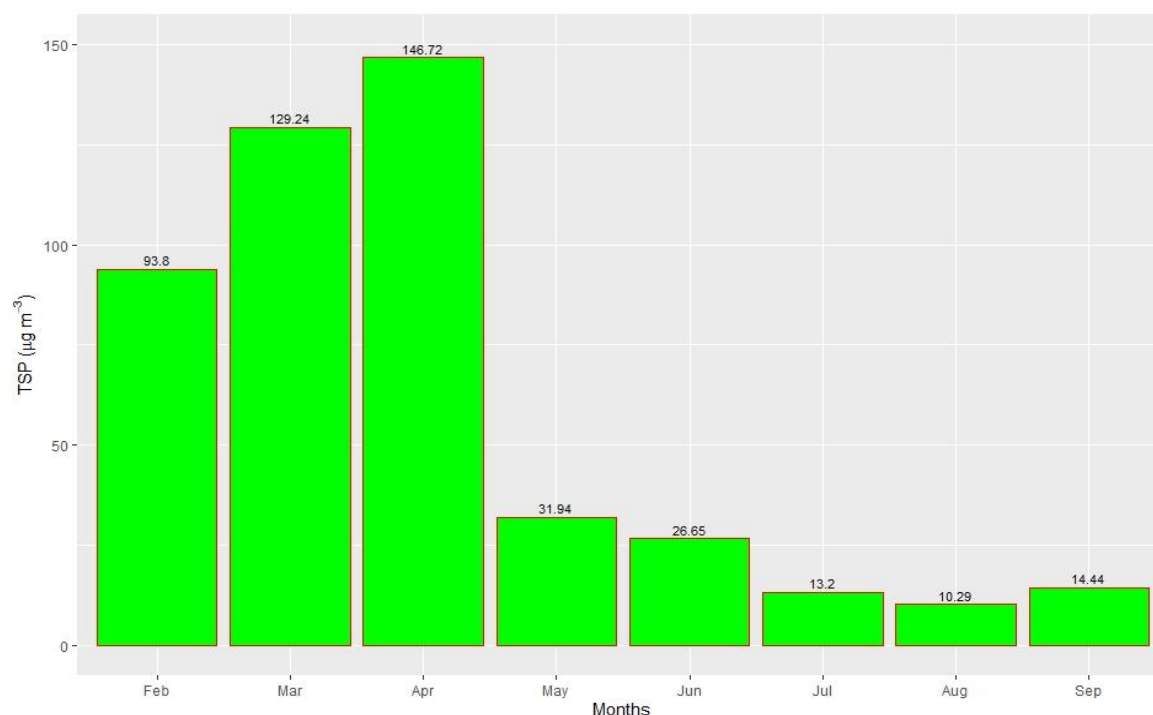
Figure 2.7.22: Monthly average of TSP
