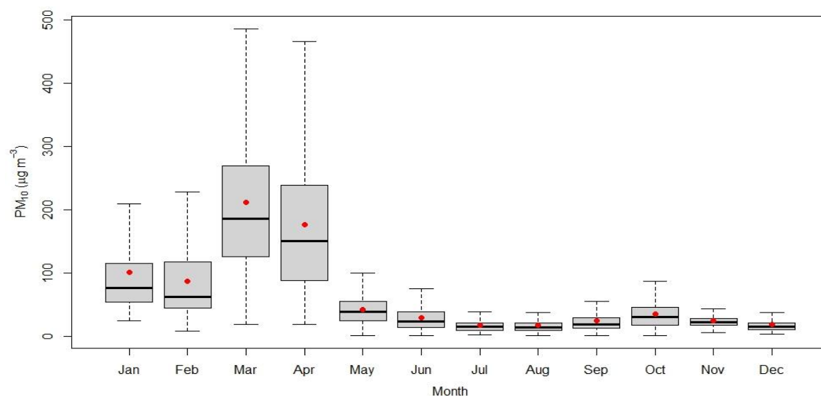
Figure 2.8.13: Monthly variation of PM 10
