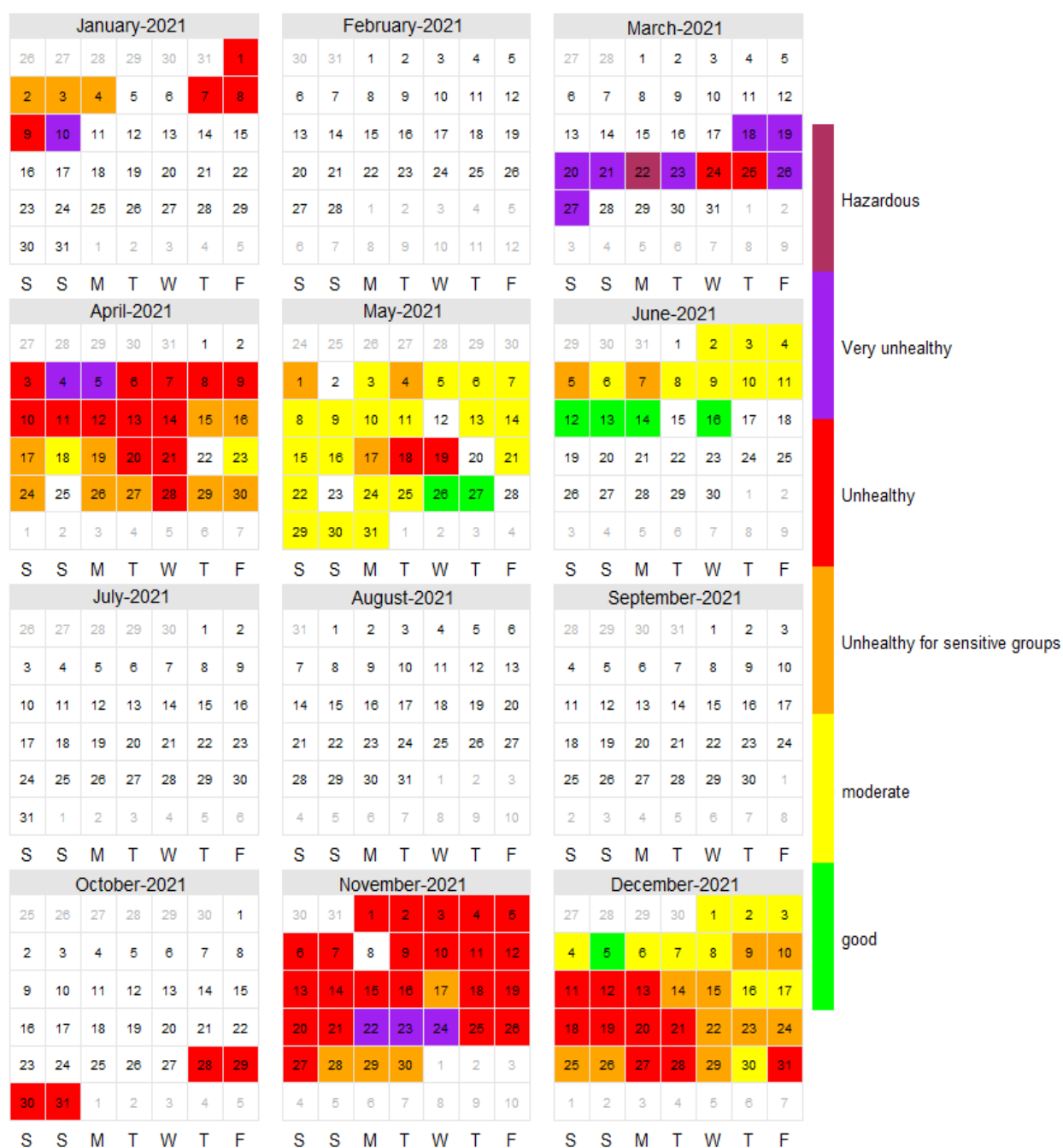
Figure 2.12.22: Calendar plot for PM 2.5 for the year 2021
