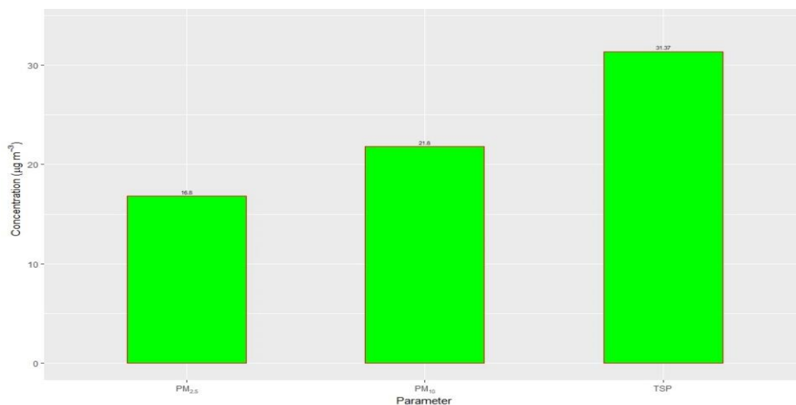
Figure 2.3.25: Annual average of PM 2.5 , PM 10 and TSP
