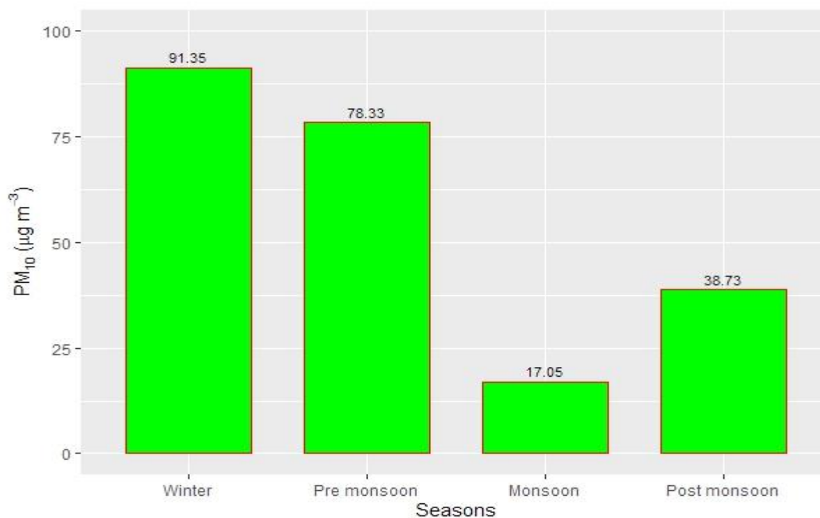
Figure 2.16.15: Seasonal variation of PM 10
