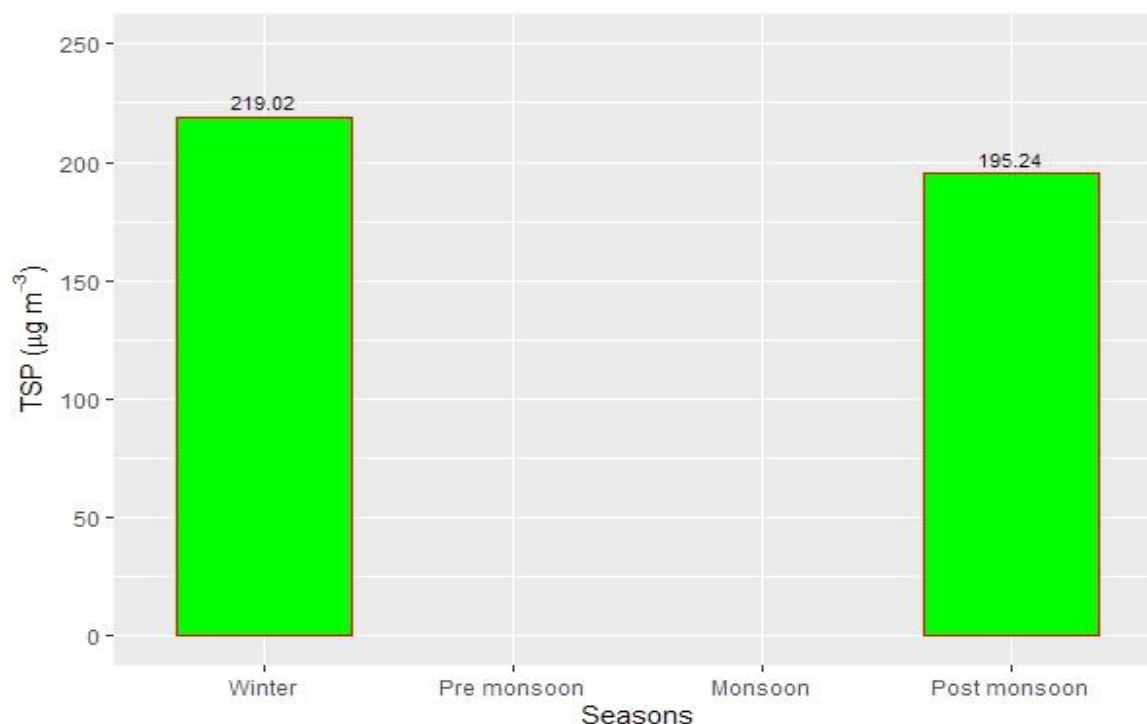
Figure 2.1.23: Seasonal variation of TSP
