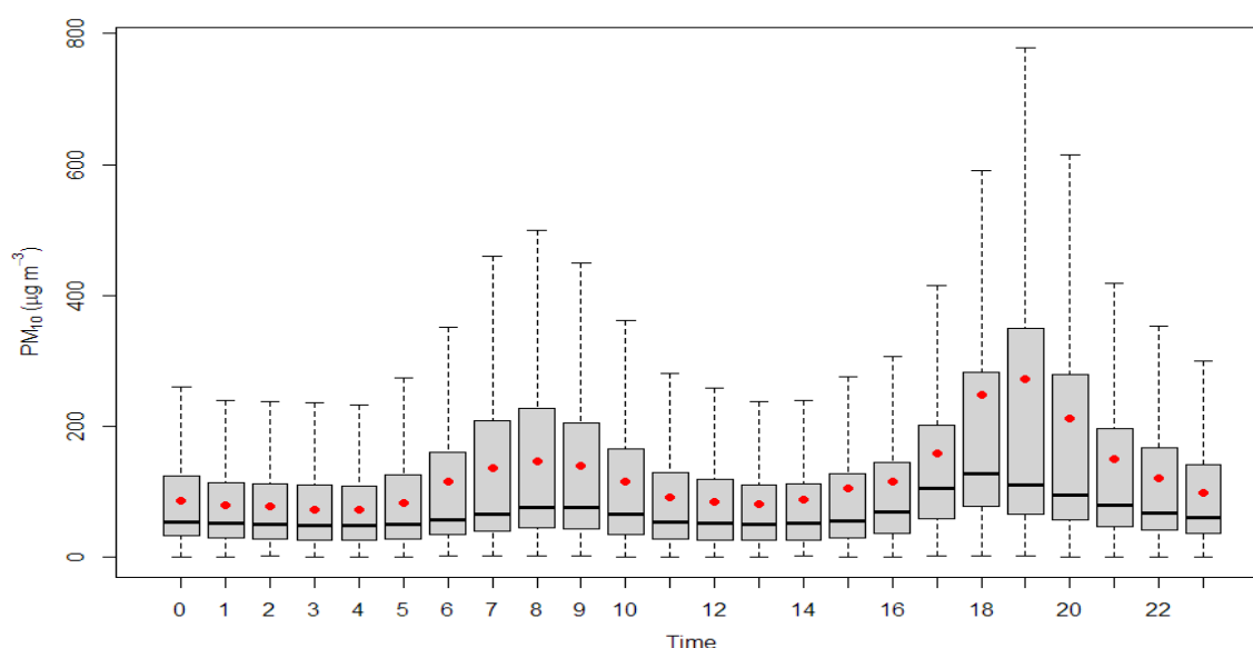
Figure 2.2.11: Diurnal variation of PM 10
