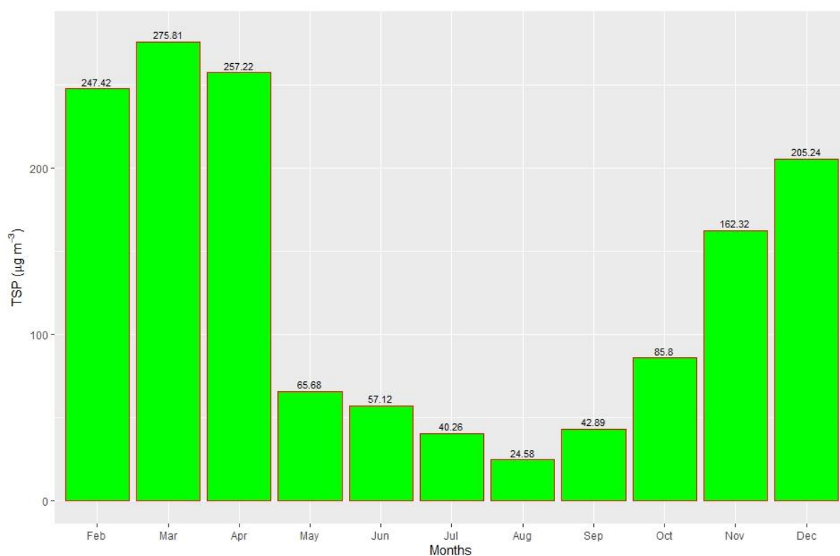
Figure 2.11.22: Monthly average of TSP
