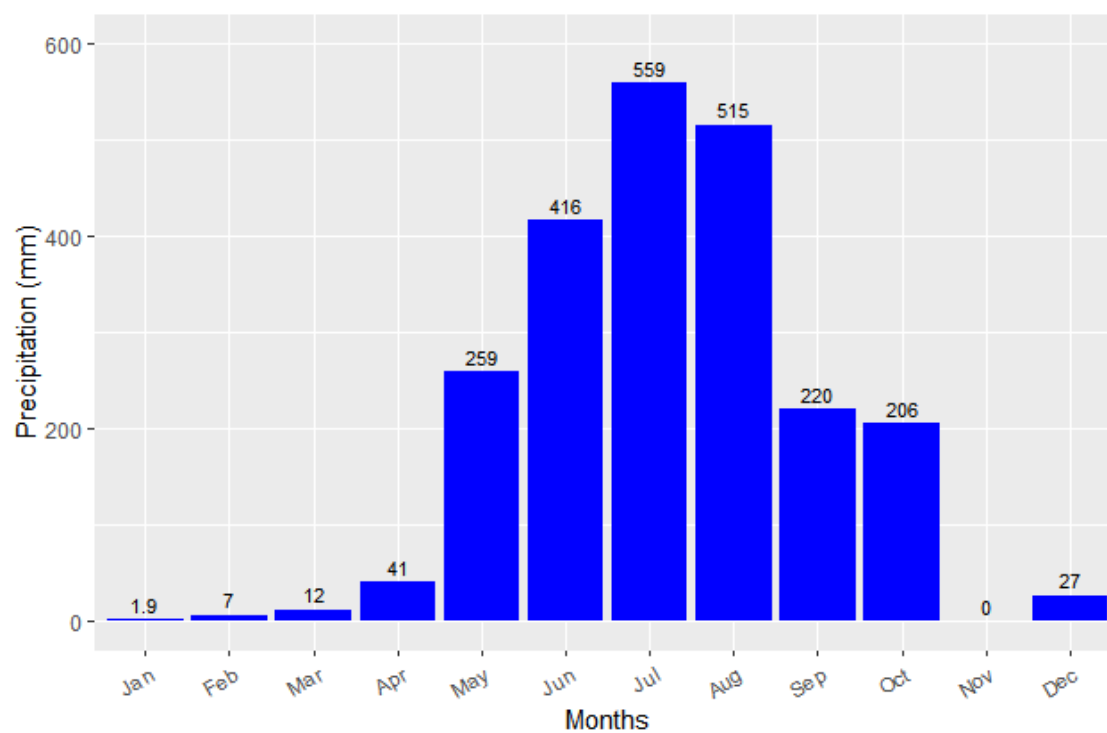
Figure 2.18.3: Monthly average precipitation with months in year 2021
