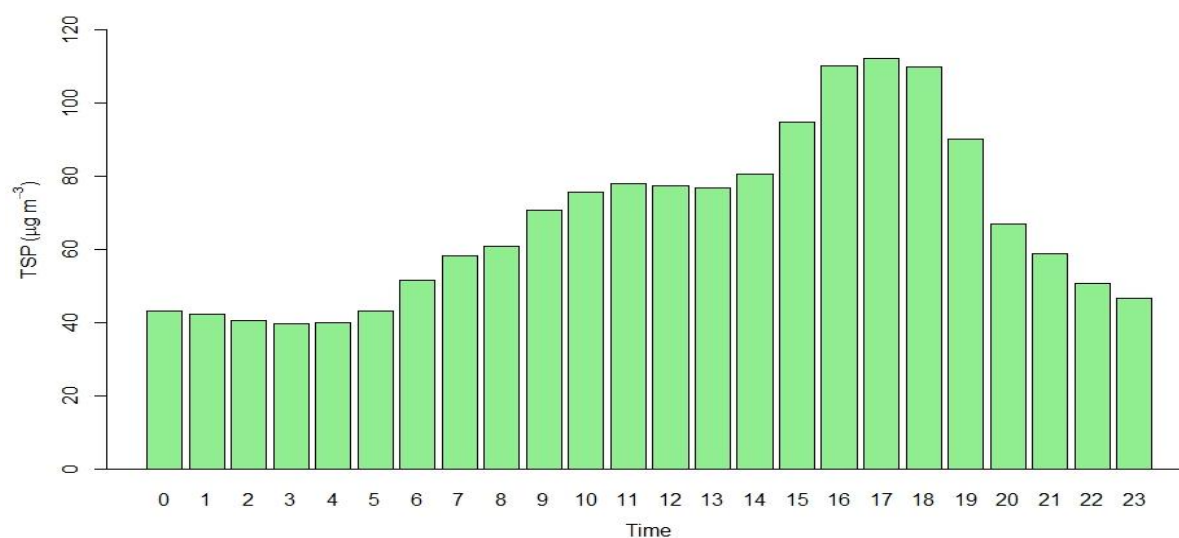
Figure 2.7.18: Hourly average of TSP
