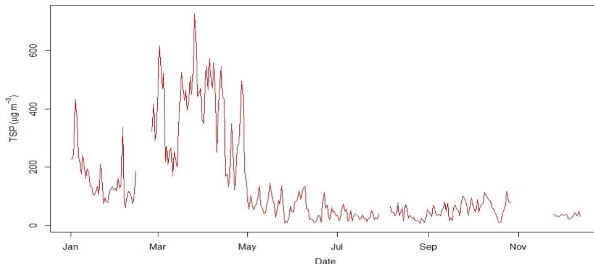
Figure 2.8.20: Daily mean concentration of TSP
