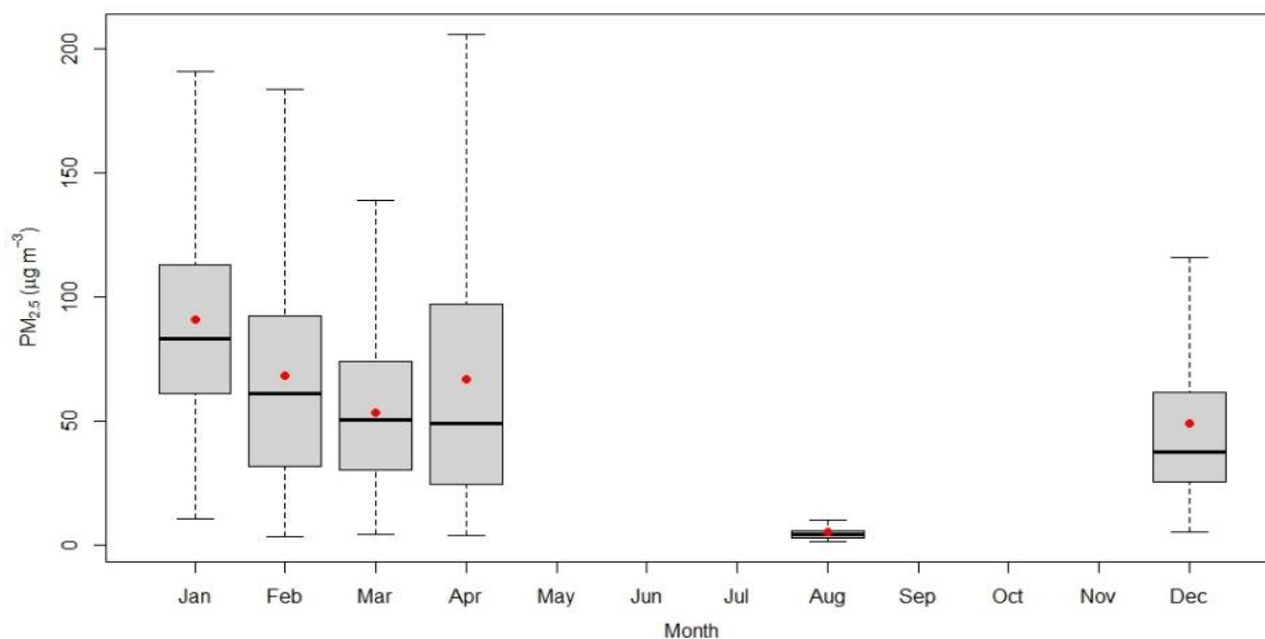
Figure 2.4.5: Monthly variation of PM 2.5
