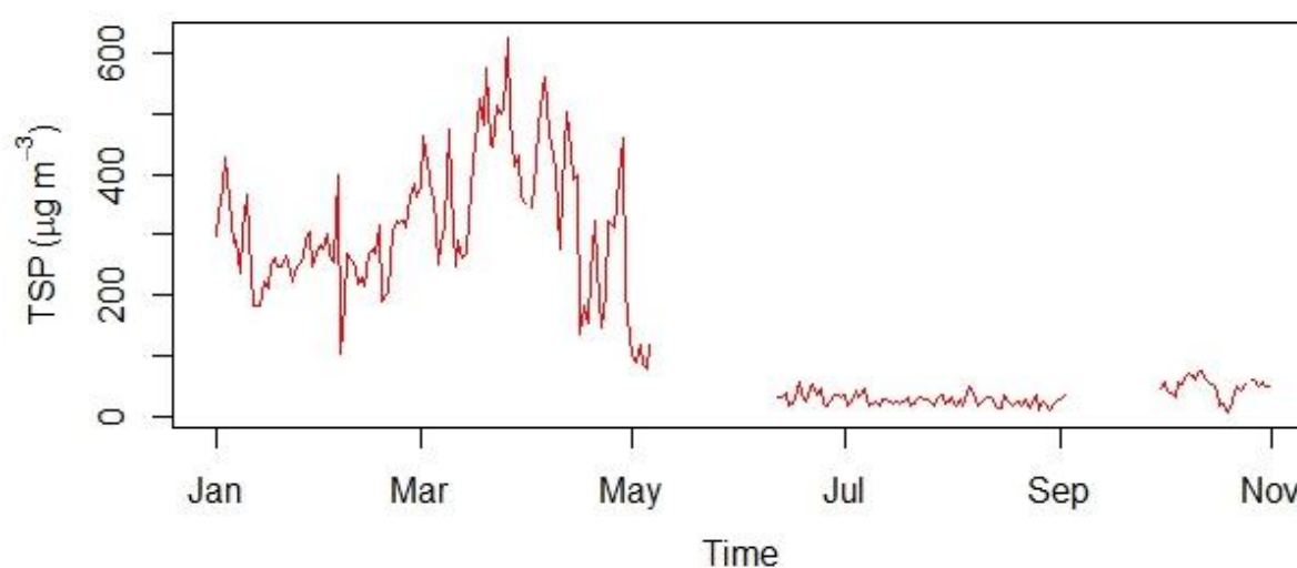
Figure 2.9.20: Daily average value of TSP
