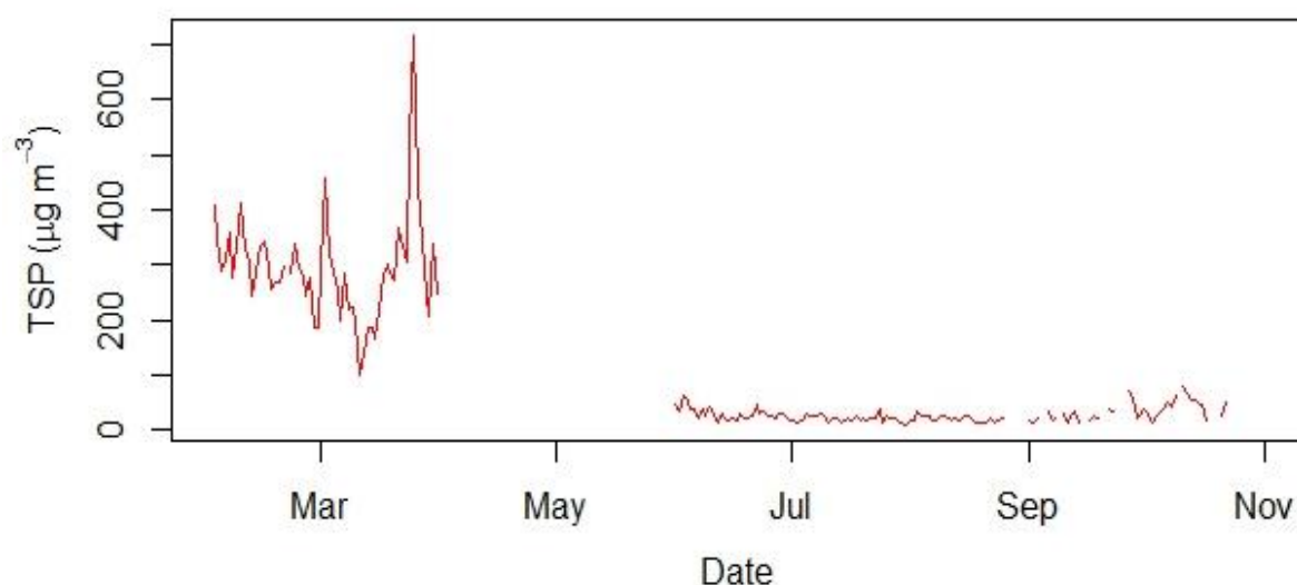
Figure 2.17.20: Daily mean concentration of TSP
