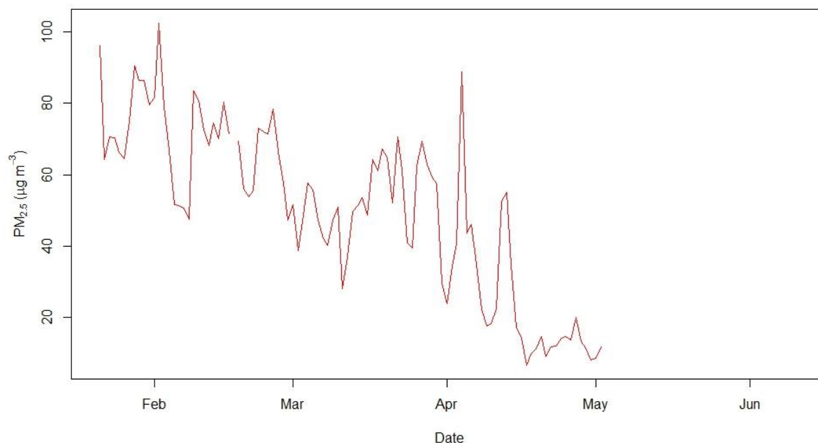
Figure 2.15.4: Daily mean concentration of PM 2.5
