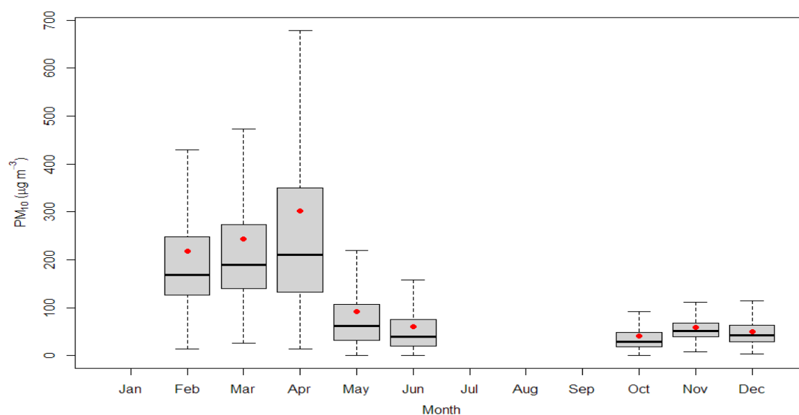
Figure 2.2.13: Monthly variation of PM 10
