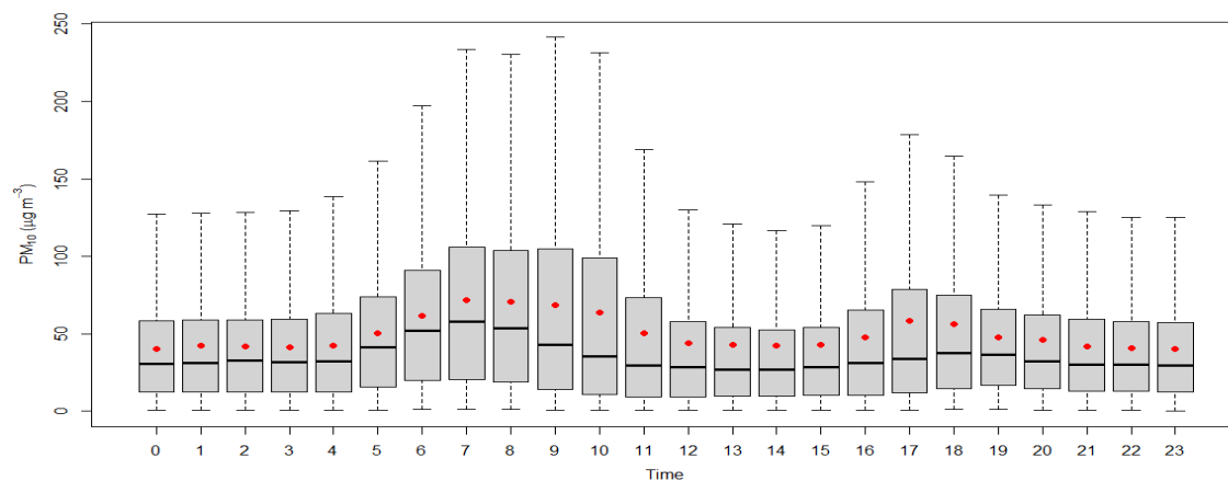
Figure 2.5.11: Diurnal variation of PM 10
