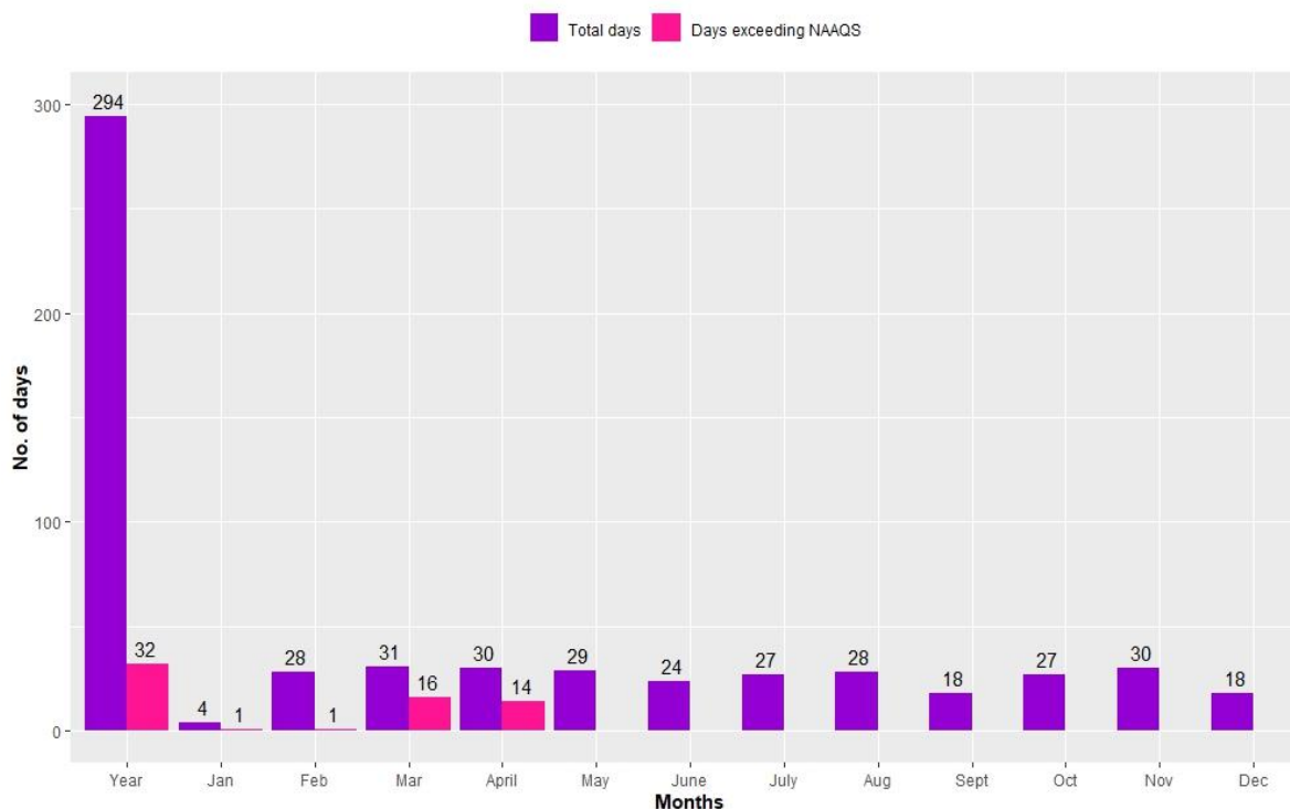
Figure 2.3.8: Compliance status of PM 2.5
