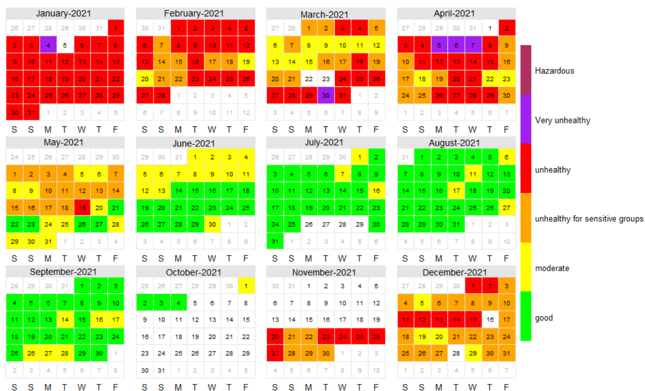
Figure 2.10.26: Calendar plot for PM 2.5 for the year 2021
