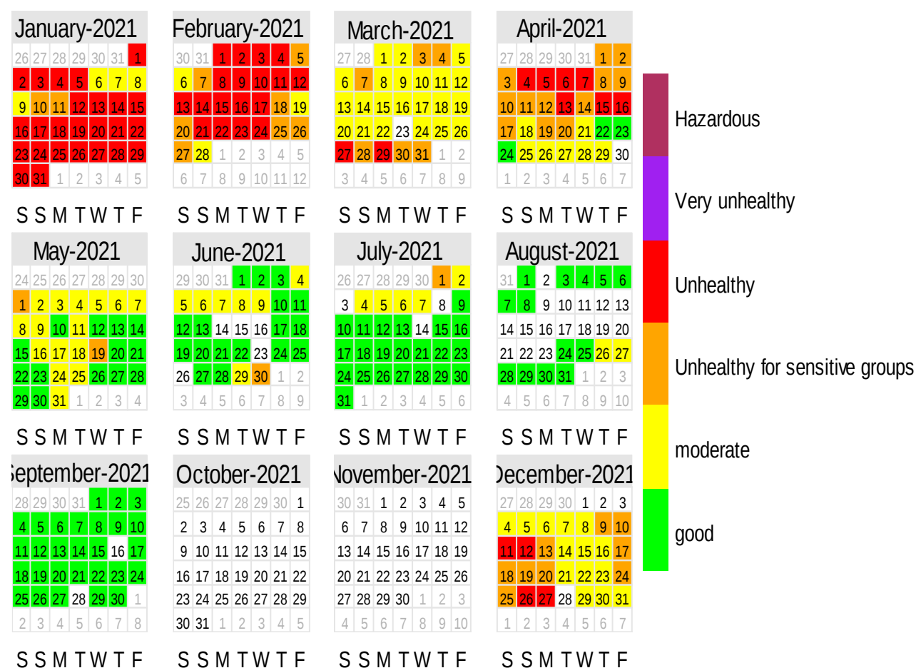
Figure 2.5.25: Calendar plot for PM 2.5 for the year 2021
