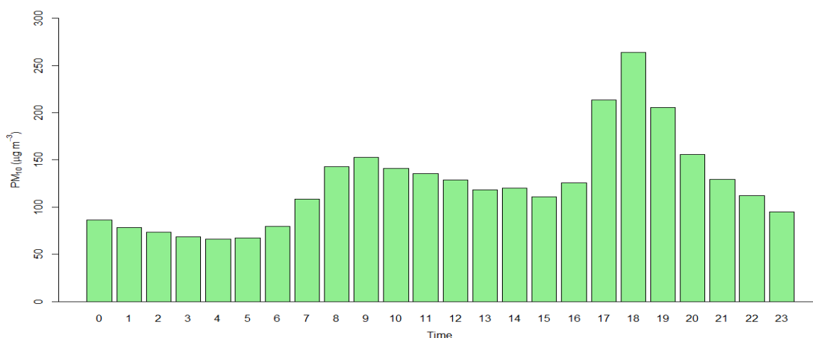
Figure 2.1.10: Hourly average of PM 10
