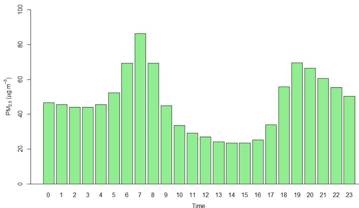
Figure 2.15.2: Hourly average of PM 2.5
