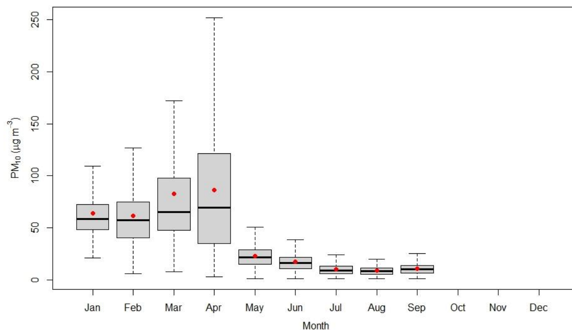
Figure 2.7.13: Monthly variation of PM 10
