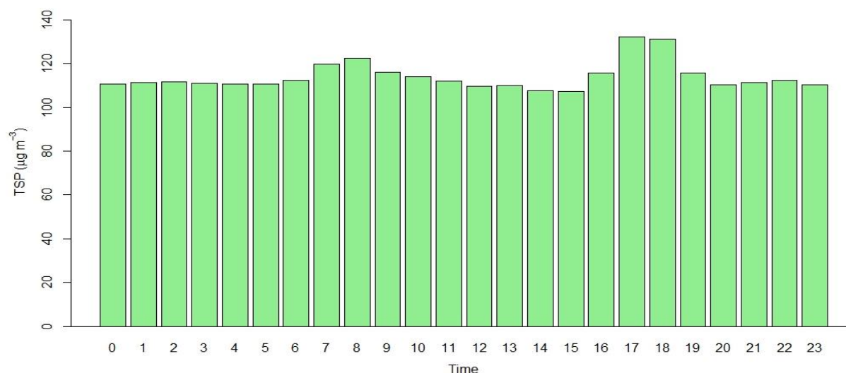
Figure 2.12.16: Hourly average of TSP
