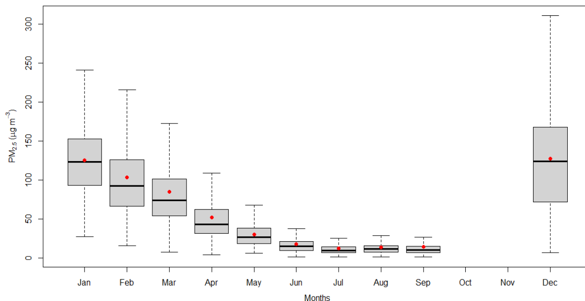
Figure 2.17.5: Monthly variation of PM_{2.5}
