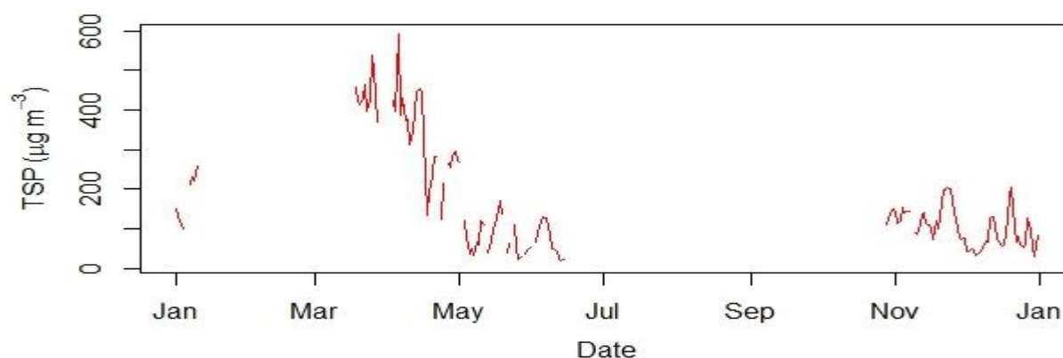
Figure 2.12.18: Daily mean concentration of TSP
