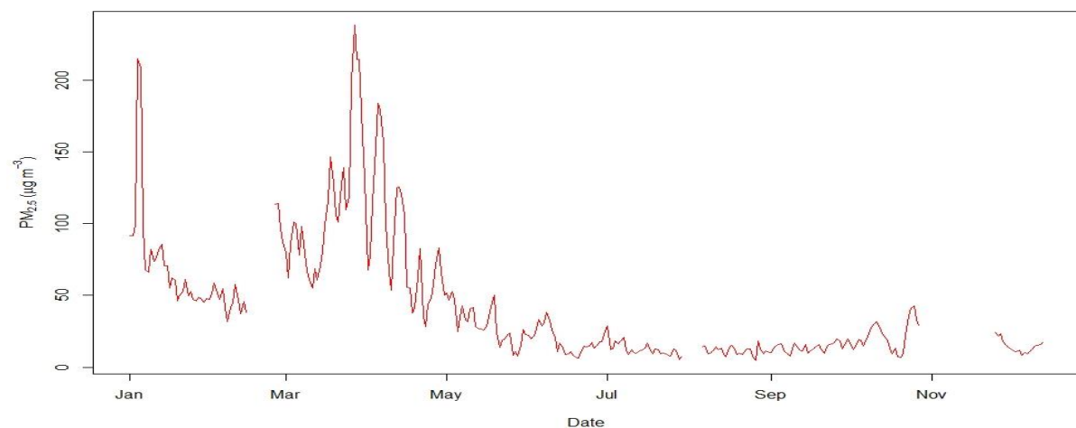
Figure 2.8.4: Daily mean concentration of PM 2.5
