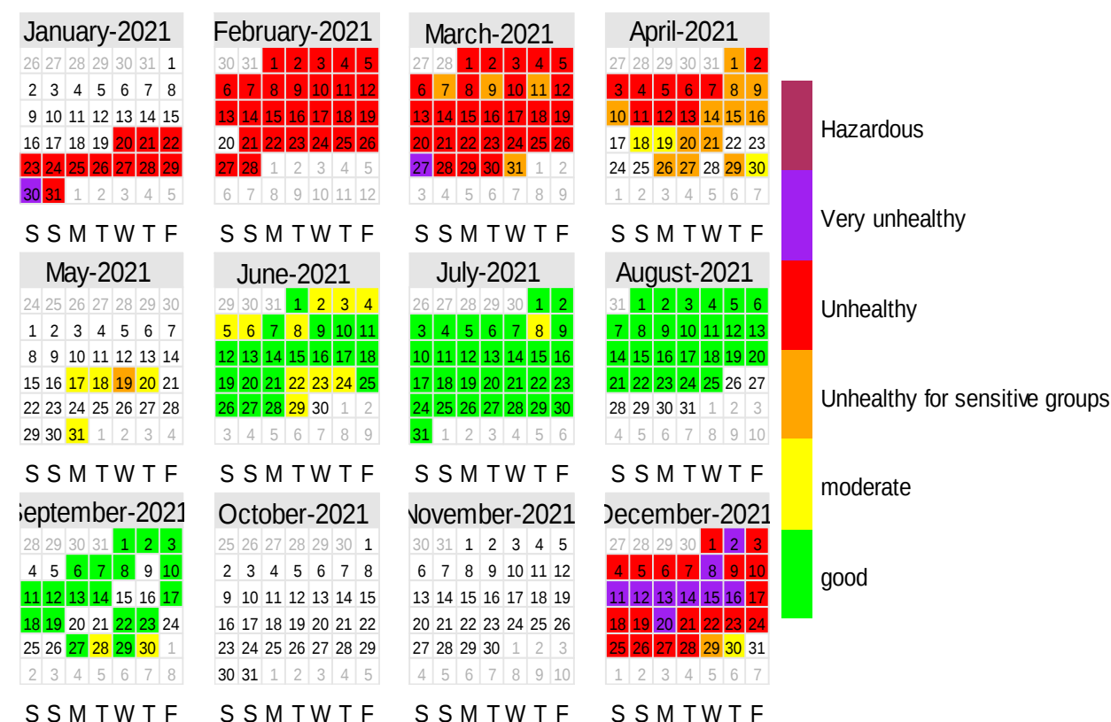
Figure 2.17.25: Calendar plot of PM 2.5 for the year 2021
