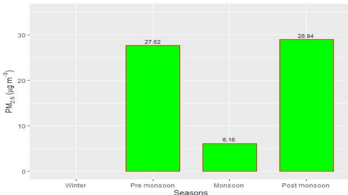
Figure 2.13.7: Seasonal variation of PM 2.5
