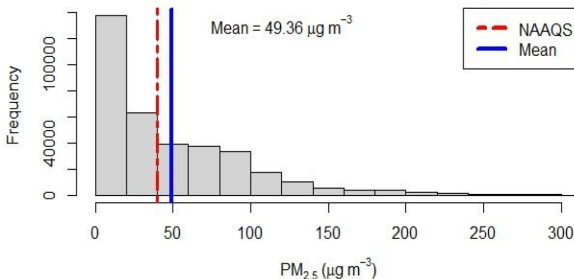
Figure 2.9.1: Histogram of PM 2.5
