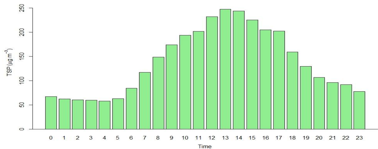
Figure 2.8.18: Hourly average of TSP
