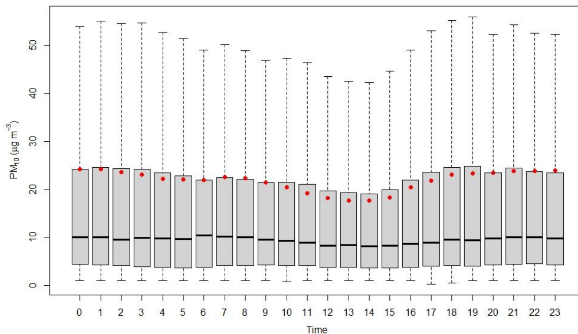
Figure 2.3.11: Diurnal variation of PM 10
