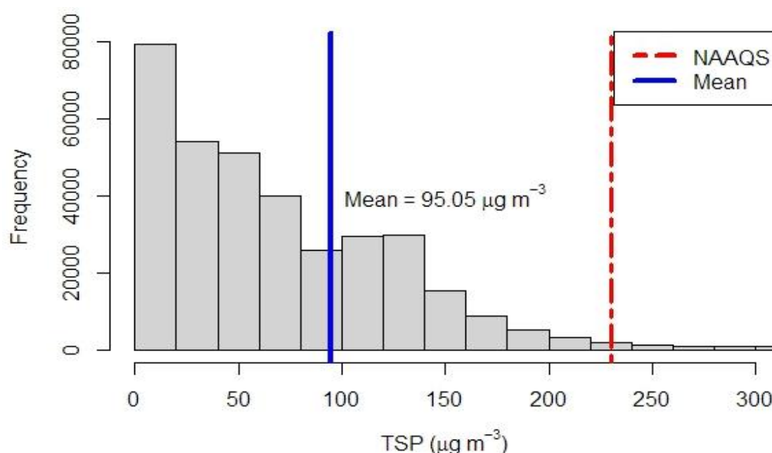
Figure 2.6.17: Histogram of TSP
