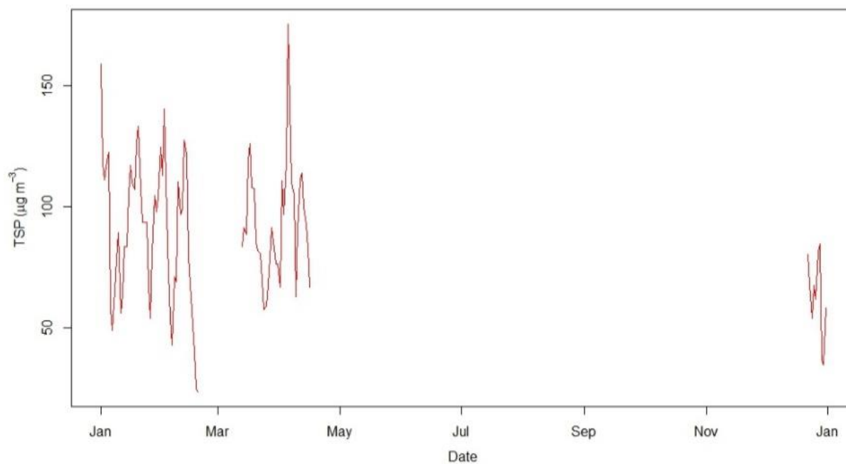
Figure 2.4.20: Daily mean concentration of TSP
