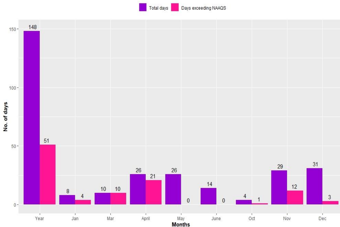
Figure 2.12.21: Compliance status of TSP
