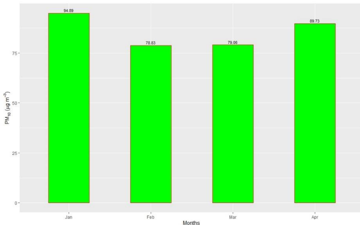
Figure 2.4.14: Monthly average of PM 10
