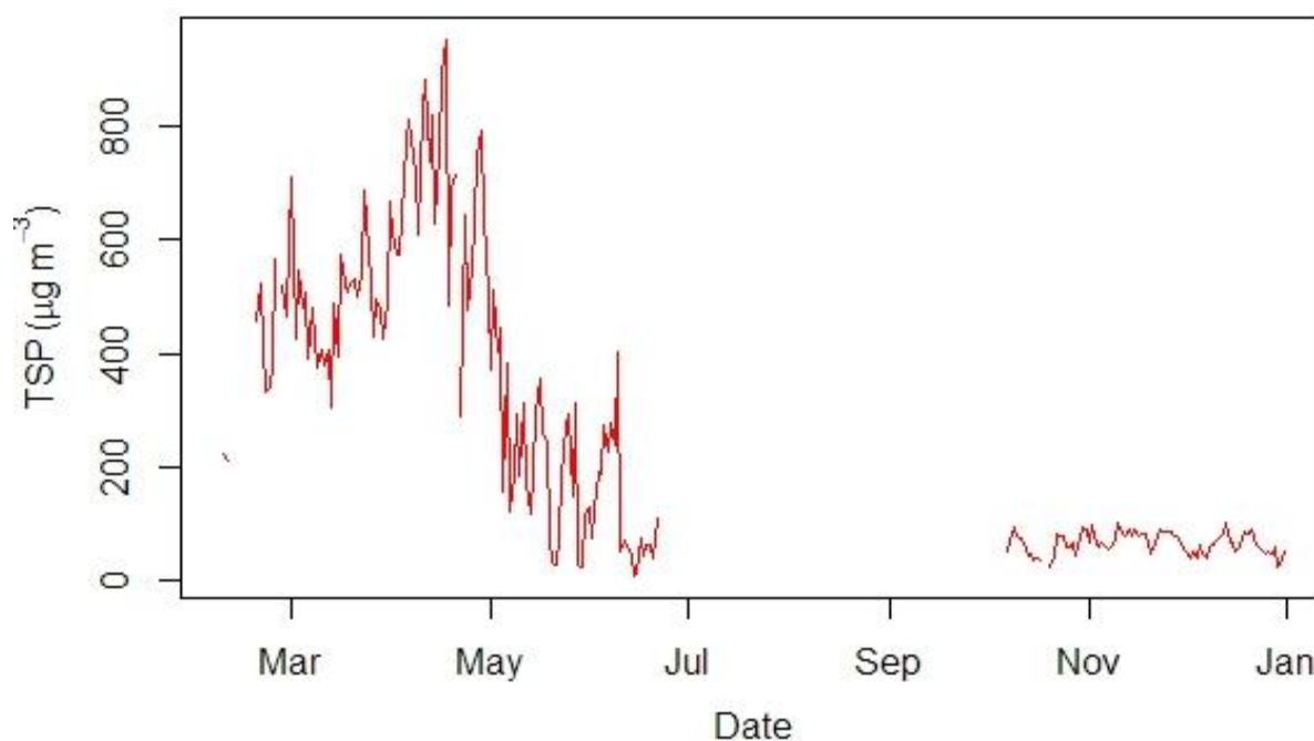
Figure 2.2.20: Daily mean concentration of TSP
