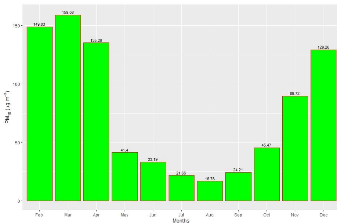
Figure 2.11.14: Monthly average of PM 10
