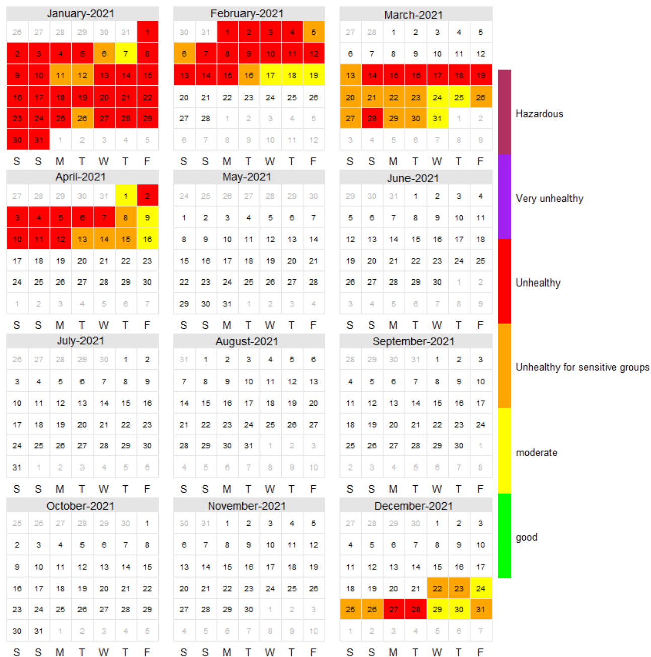
Figure 2.4.24: Calendar plot for PM 2.5 for the year 2021
