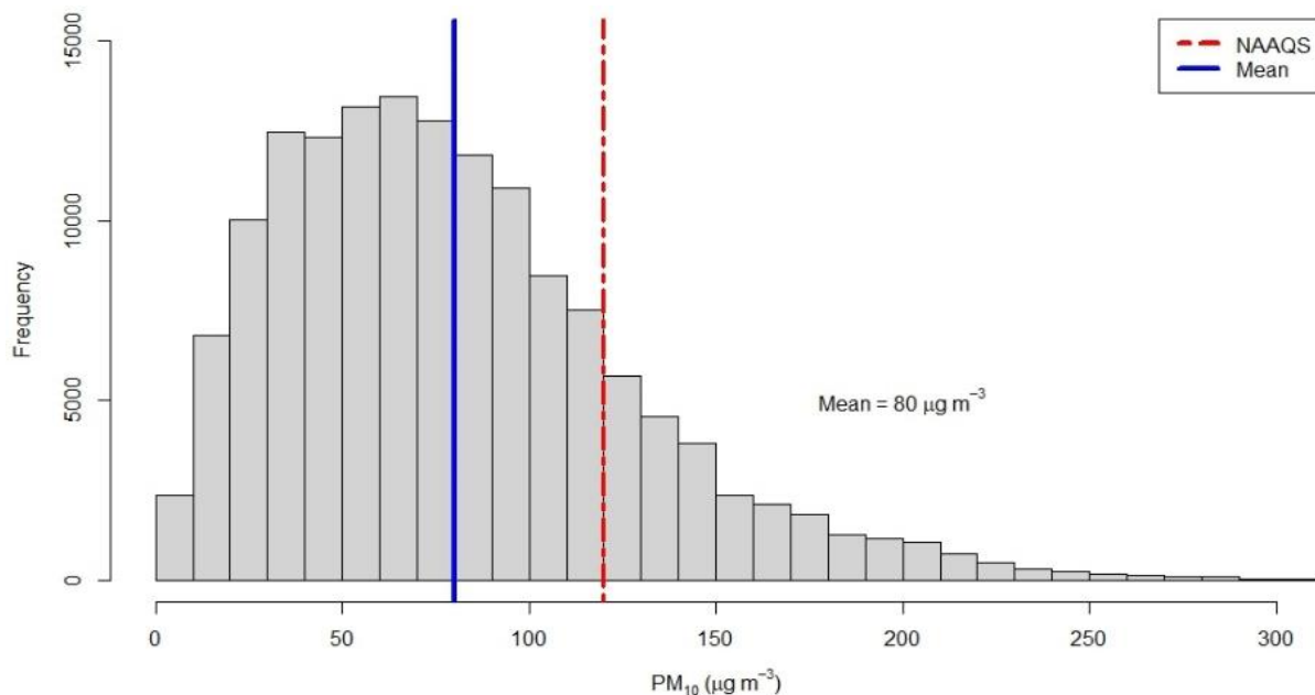
Figure 2.4.9: Histogram of PM 10
