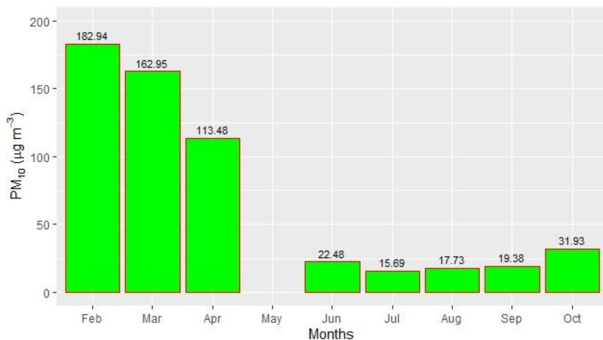
Figure 2.17.14: Monthly average of PM 10
