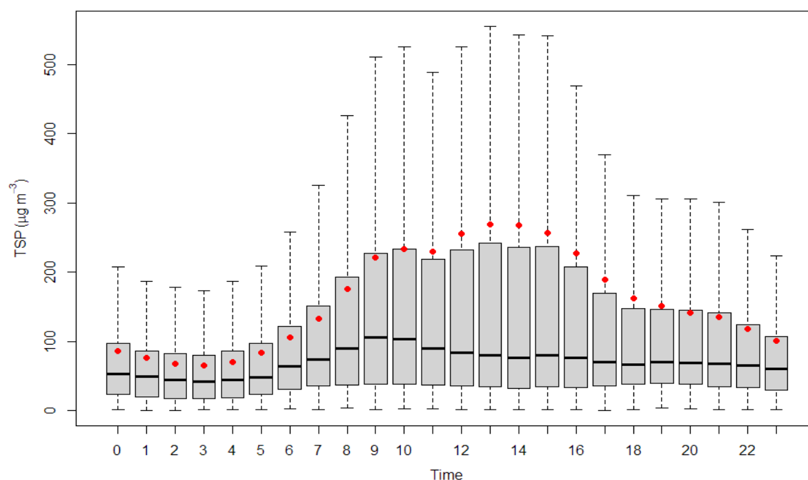
Figure 2.10.19: Diurnal variation of TSP
