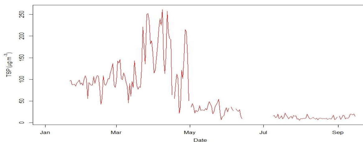
Figure 2.7.20: Daily mean concentration of TSP
