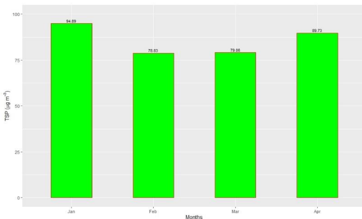
Figure 2.4.22: Monthly average of TSP
