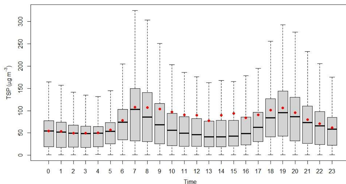
Figure 2.17.19: Diurnal variation of TSP
