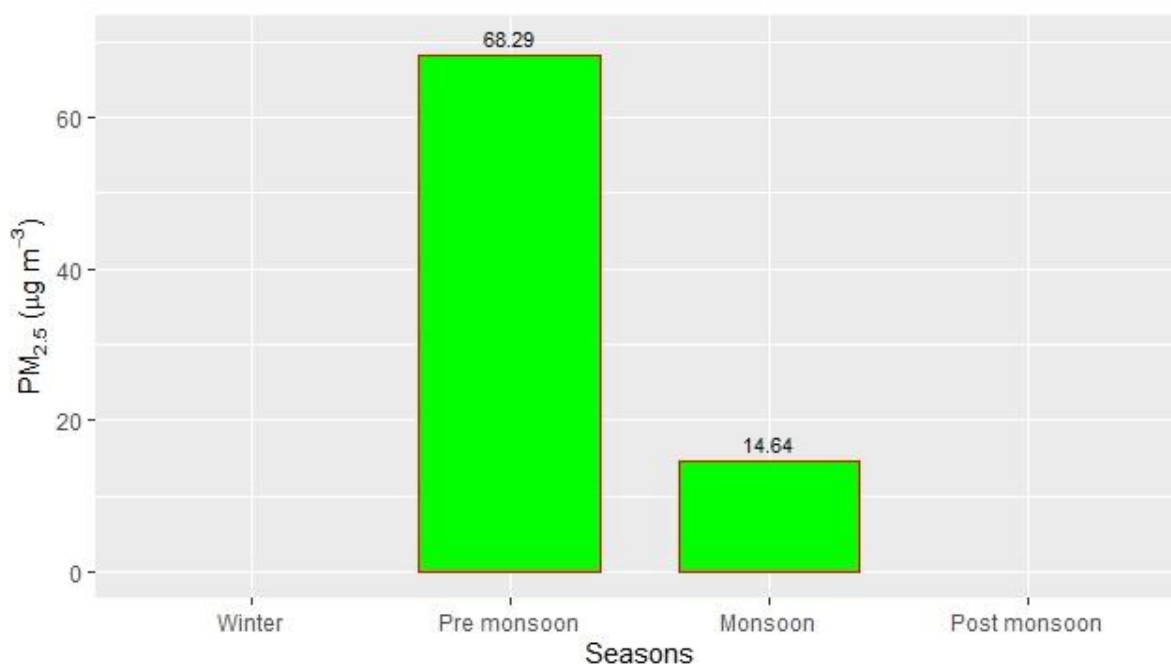
Figure 2.17.7: Seasonal variation of PM 2.5
