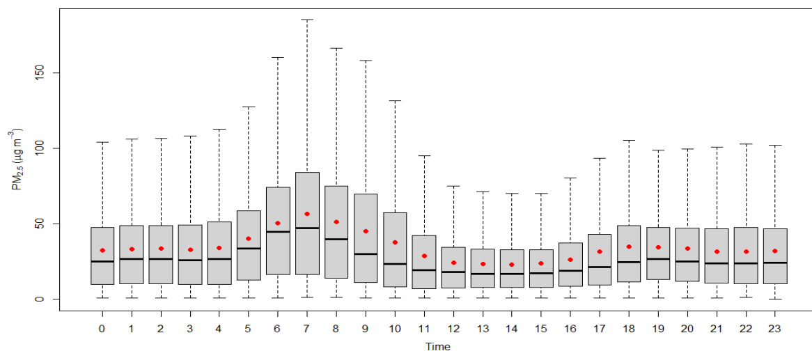
Figure 2.5.3: Diurnal variation of PM 2.5
