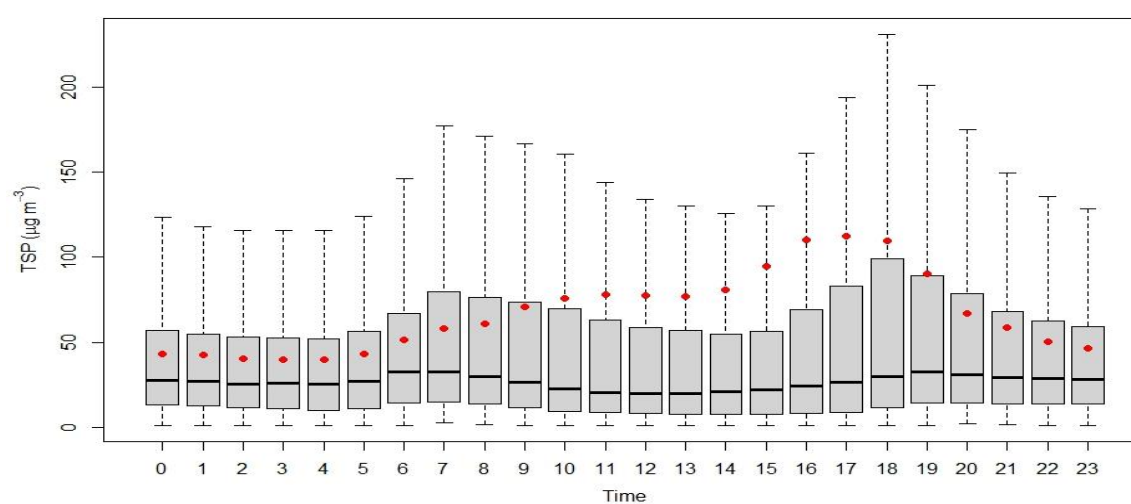
Figure 2.7.19: Diurnal variation of TSP
