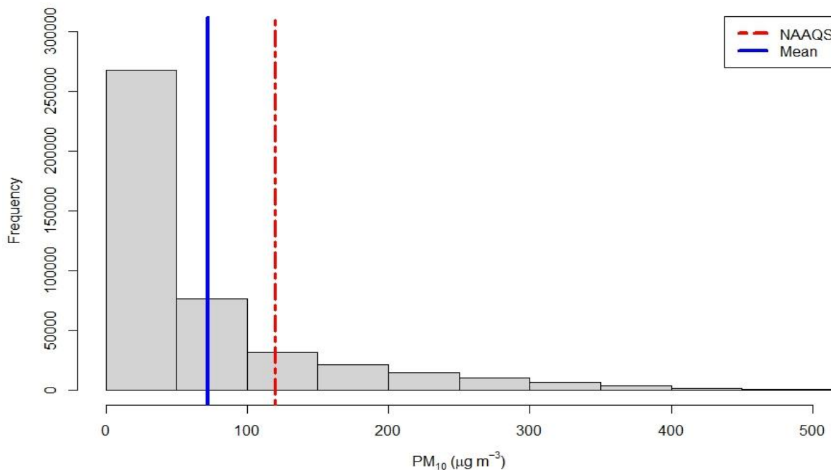
Figure 2.8.9: Histogram of PM 10
