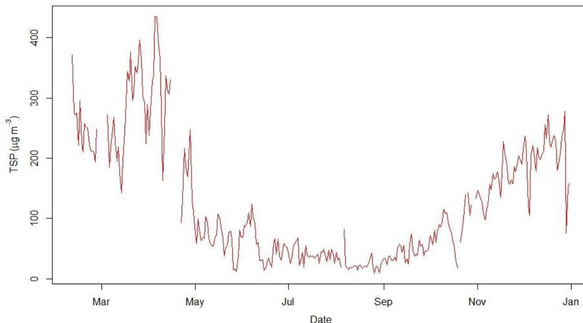
Figure 2.11.20: Daily mean concentration of TSP
