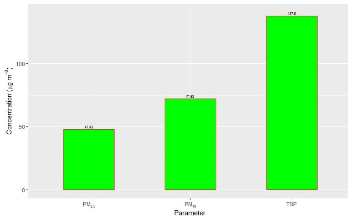
Figure 2.8.25: Annual average of PM 2.5 , PM 10 and TSP
