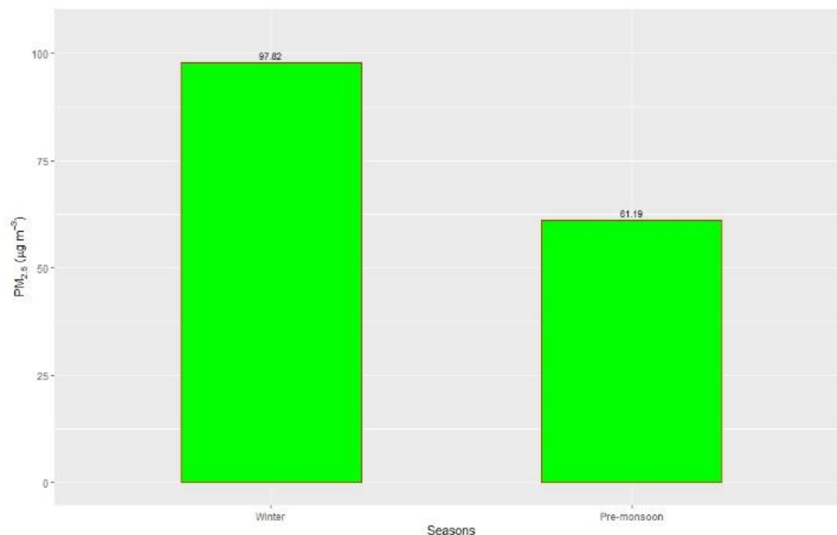
Figure 2.4.7: Seasonal variation of PM 2.5
