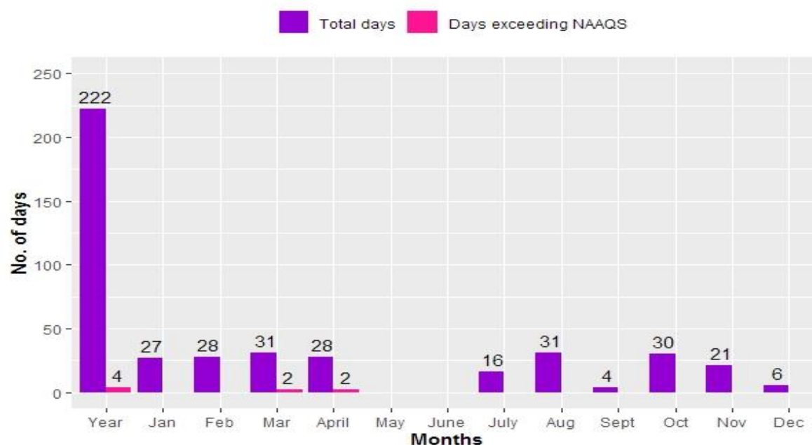
Figure 2.6.24: Compliance status of TSP
