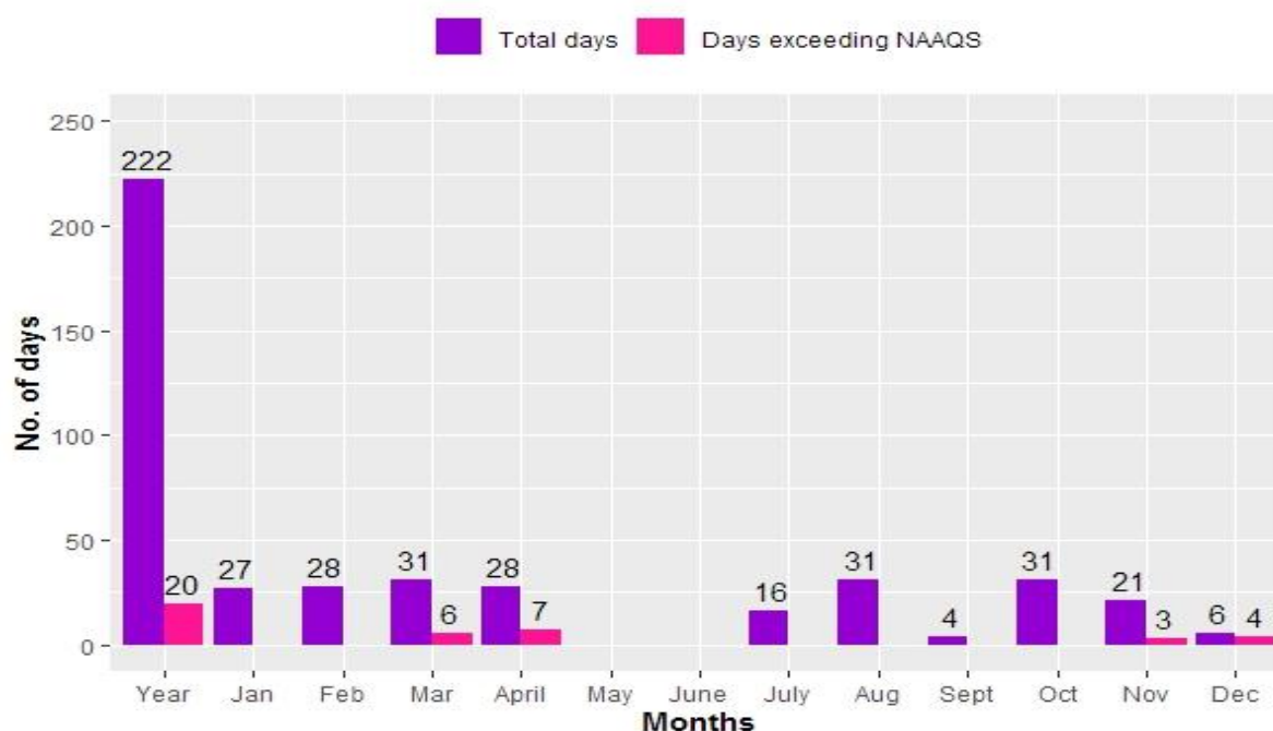
Figure 2.6.16: Compliance status of PM 10
