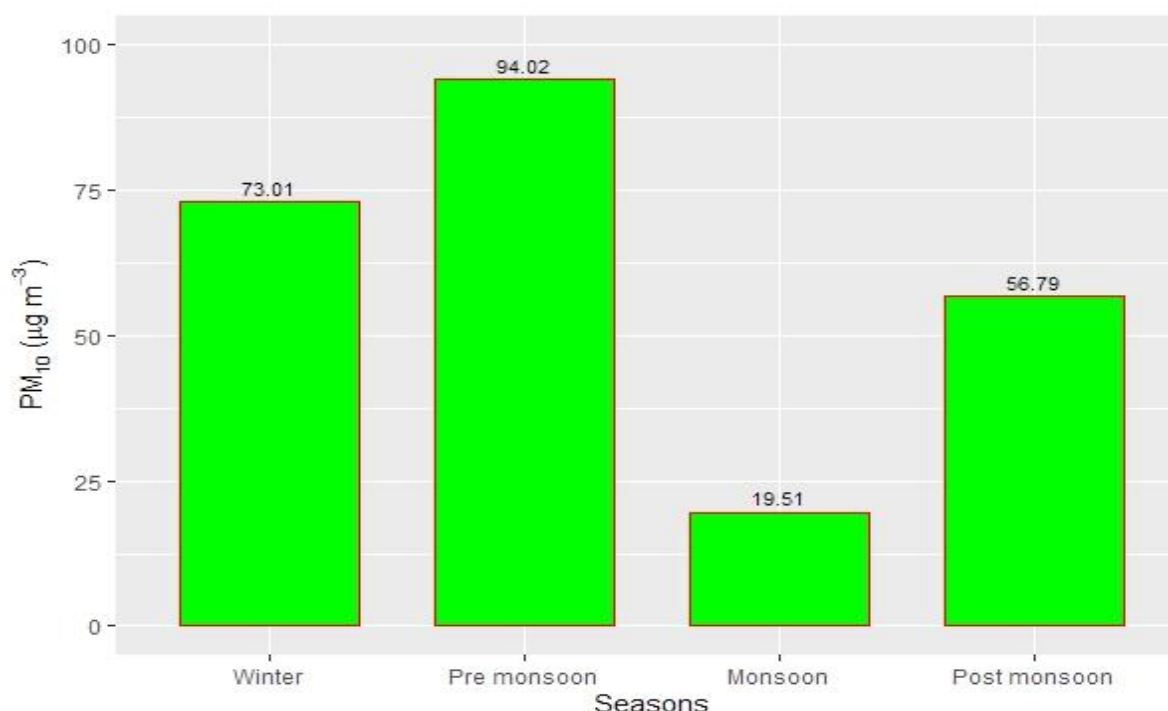
Figure 2.6.15: Seasonal variation of PM 10
