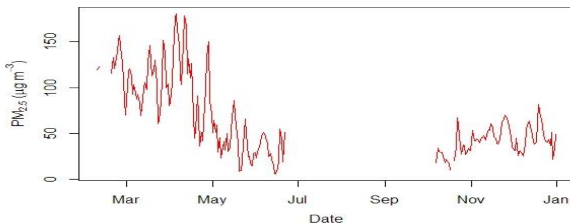
Figure 2.2.4: Daily mean concentration of PM 2.5
