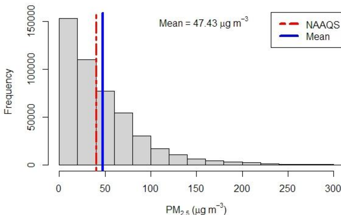
Figure 2.10.1: Histogram of PM 2.5
