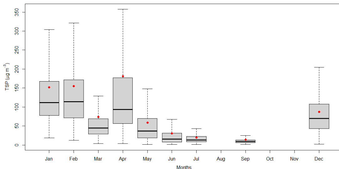
Figure 2.5.21: Monthly variation of TSP
