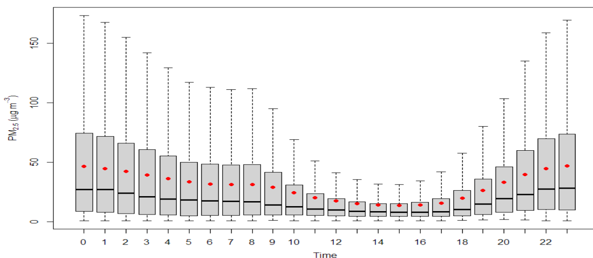
Figure 2.13.3: Diurnal variation of PM 2.5
