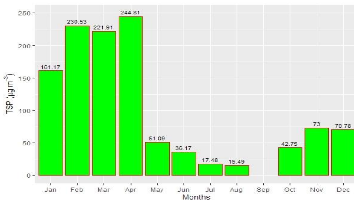
Figure 2.16.22: Monthly average of TSP
