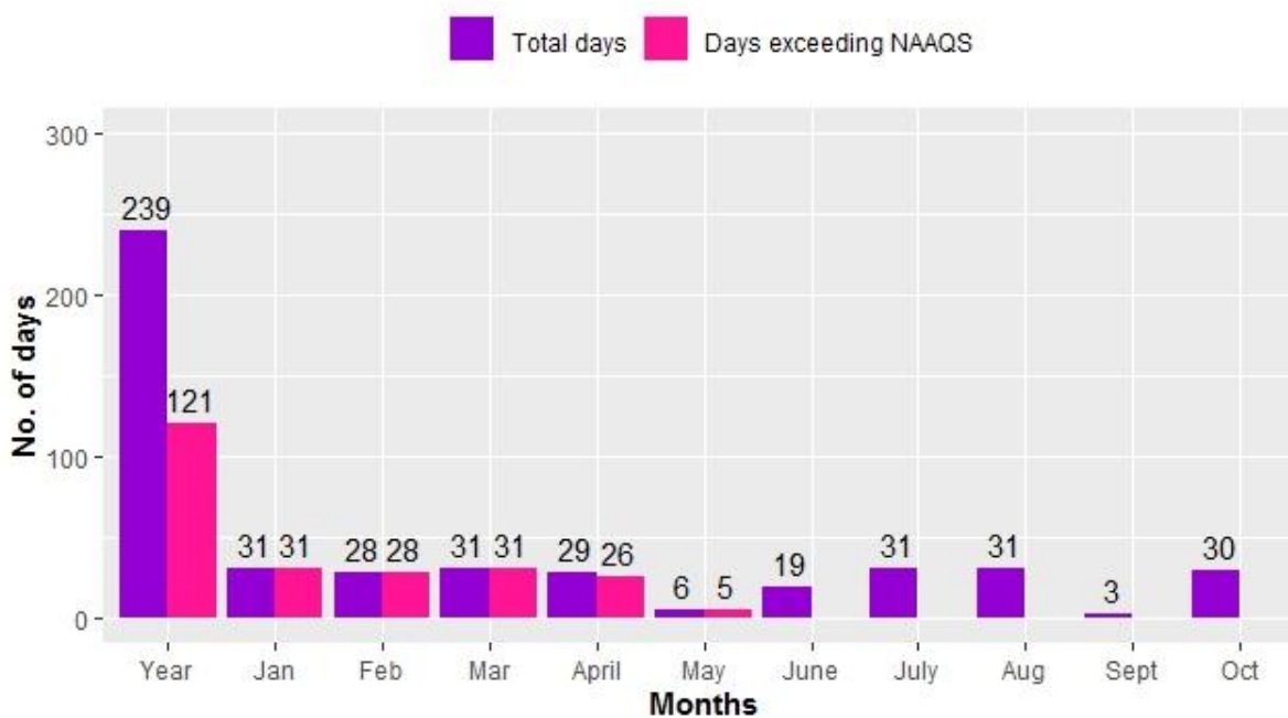
Figure 2.9.8: Compliance status of \text{PM}_{2.5}
