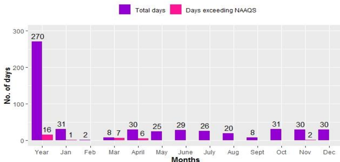
Figure 2.14.24: Compliance status of TSP
