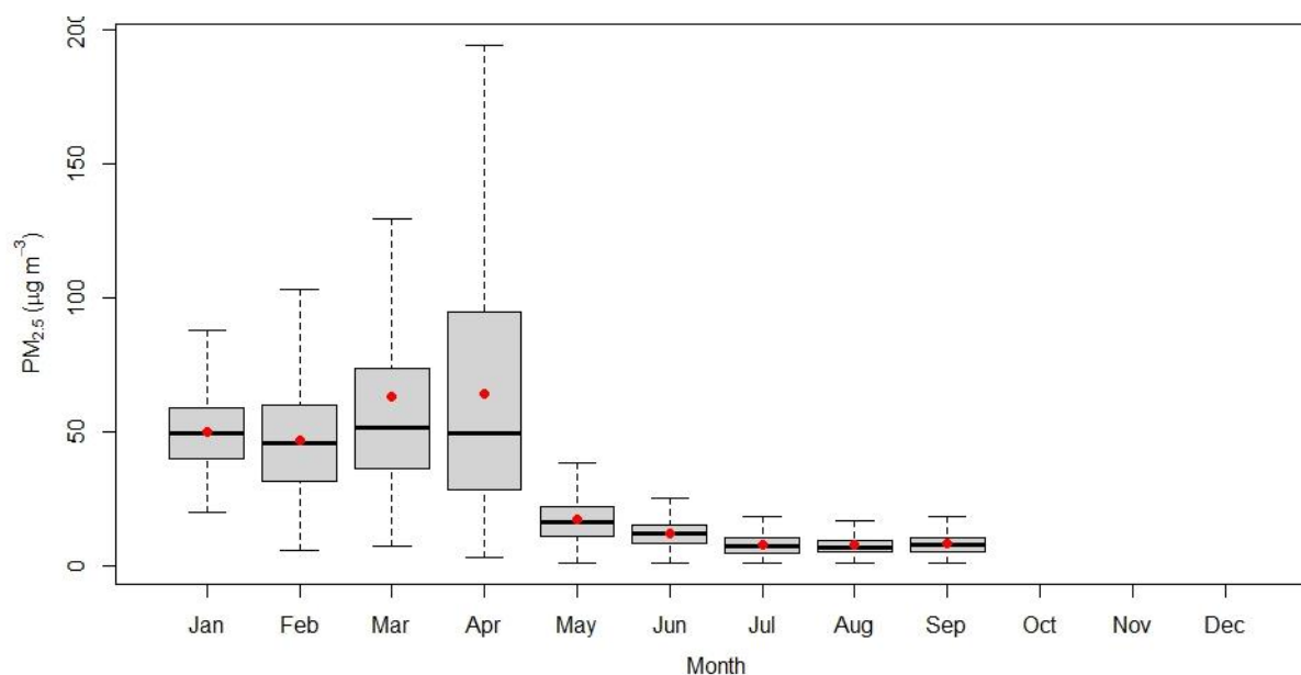
Figure 2.7.5: Monthly variation of PM 2.5
