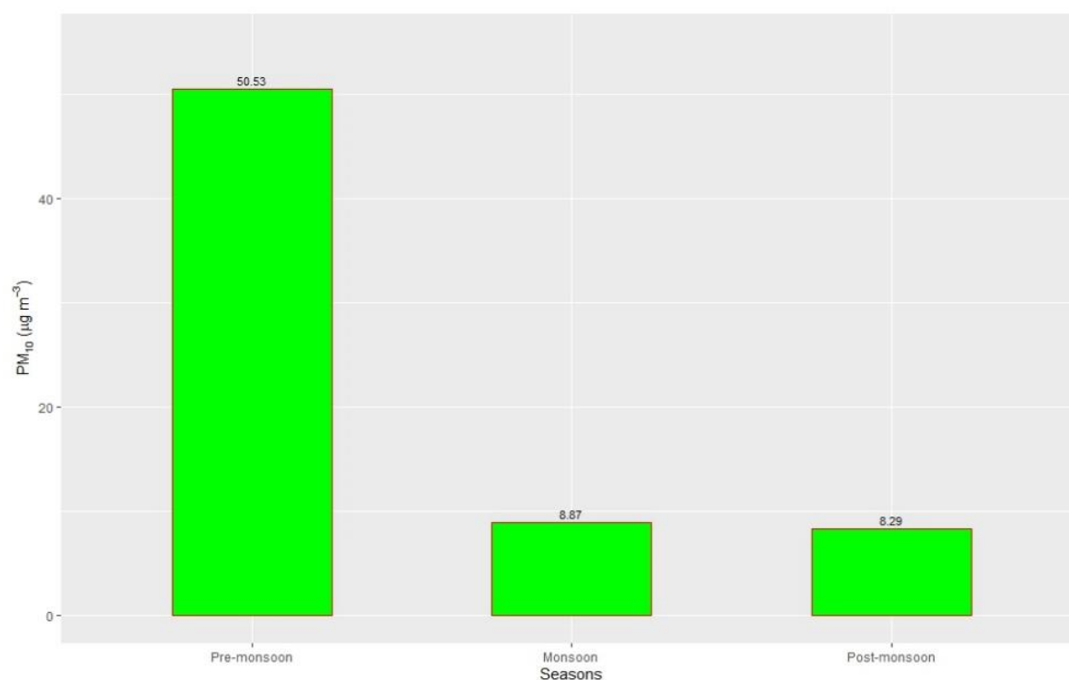
Figure 2.3.15: Seasonal variation of PM 10
