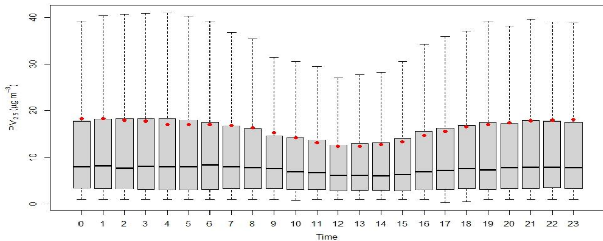
Figure 2.3.3: Diurnal variation of PM 2.5
