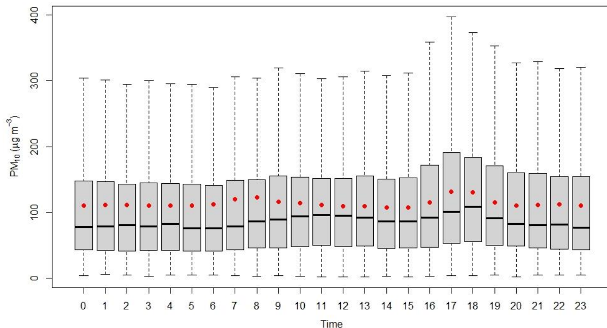
Figure 2.12.10: Diurnal variation of PM 10
