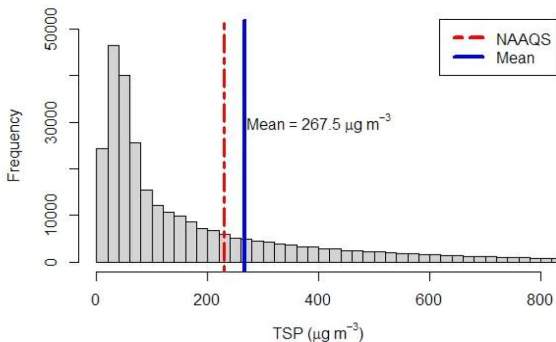
Figure 2.2.17: Histogram of TSP
