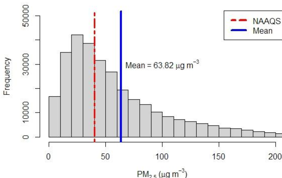
Figure 2.2.1: Histogram of PM 2.5
