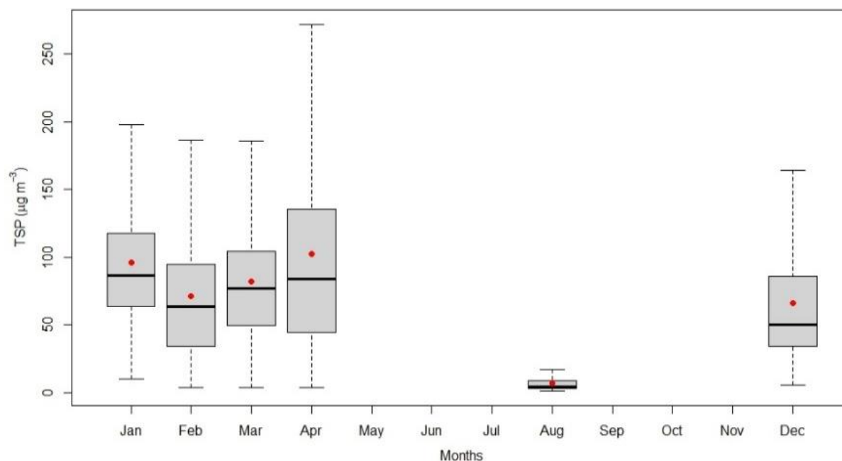
Figure 2.4.21: Monthly variation of TSP
