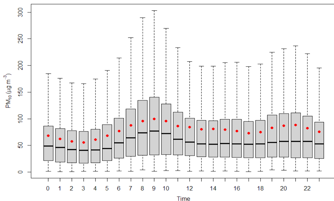
Figure 2.10.11: Diurnal variation of PM_{10}
