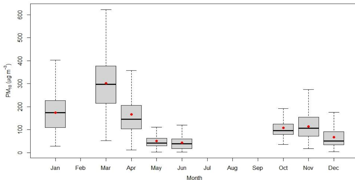
Figure 2.12.12: Monthly variation of PM 10
