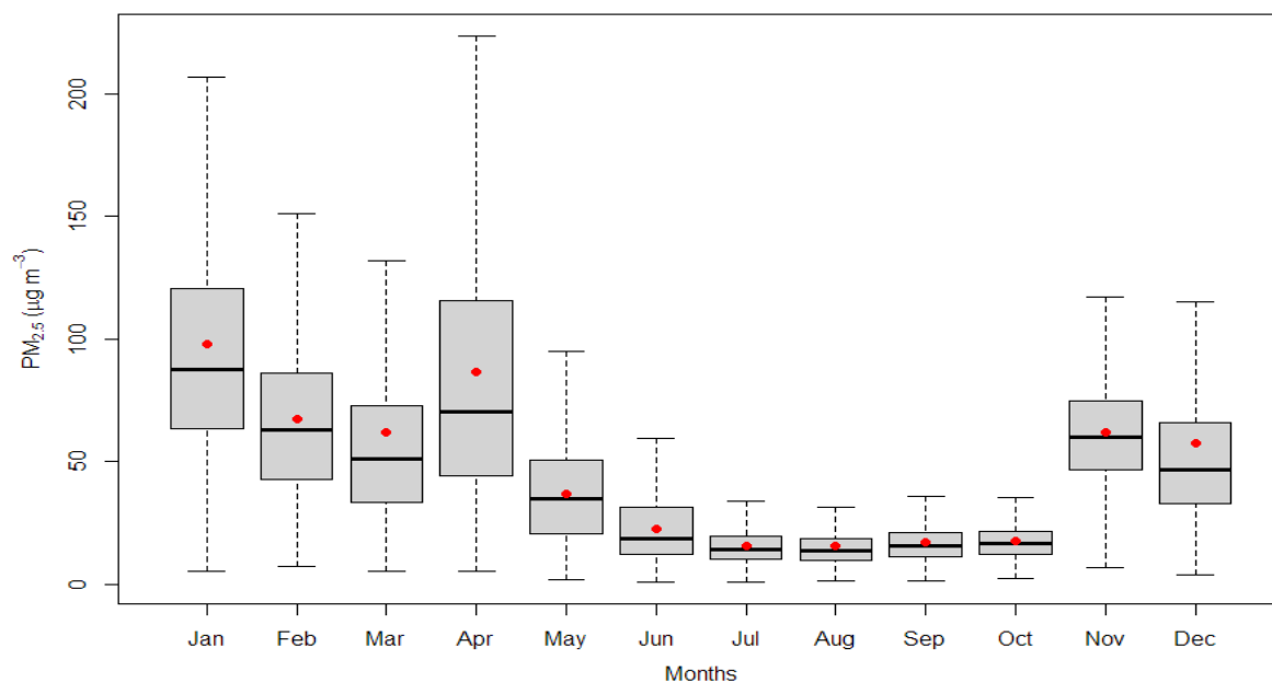
Figure 2.10.5: Monthly variation of PM 2.5
