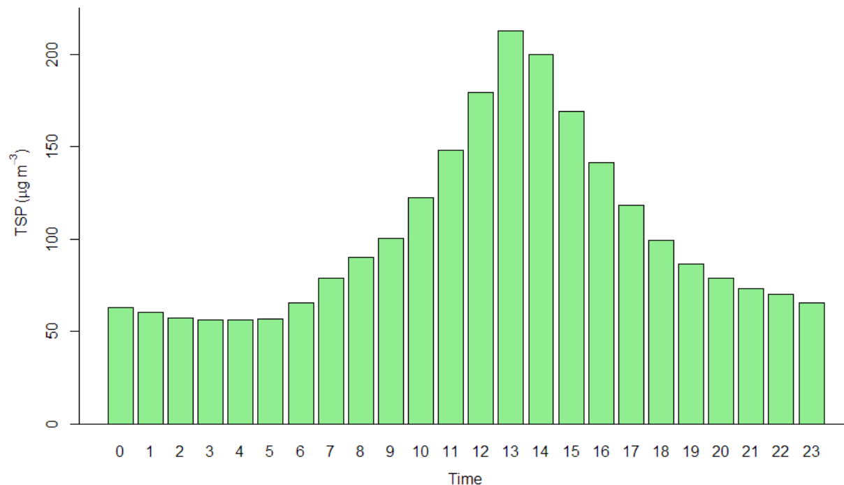
Figure 2.16.18: Hourly average of TSP
