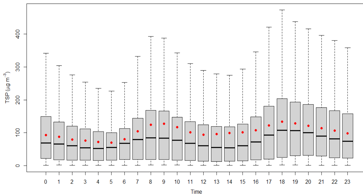
Figure 2.14.19: Diurnal variation of TSP
