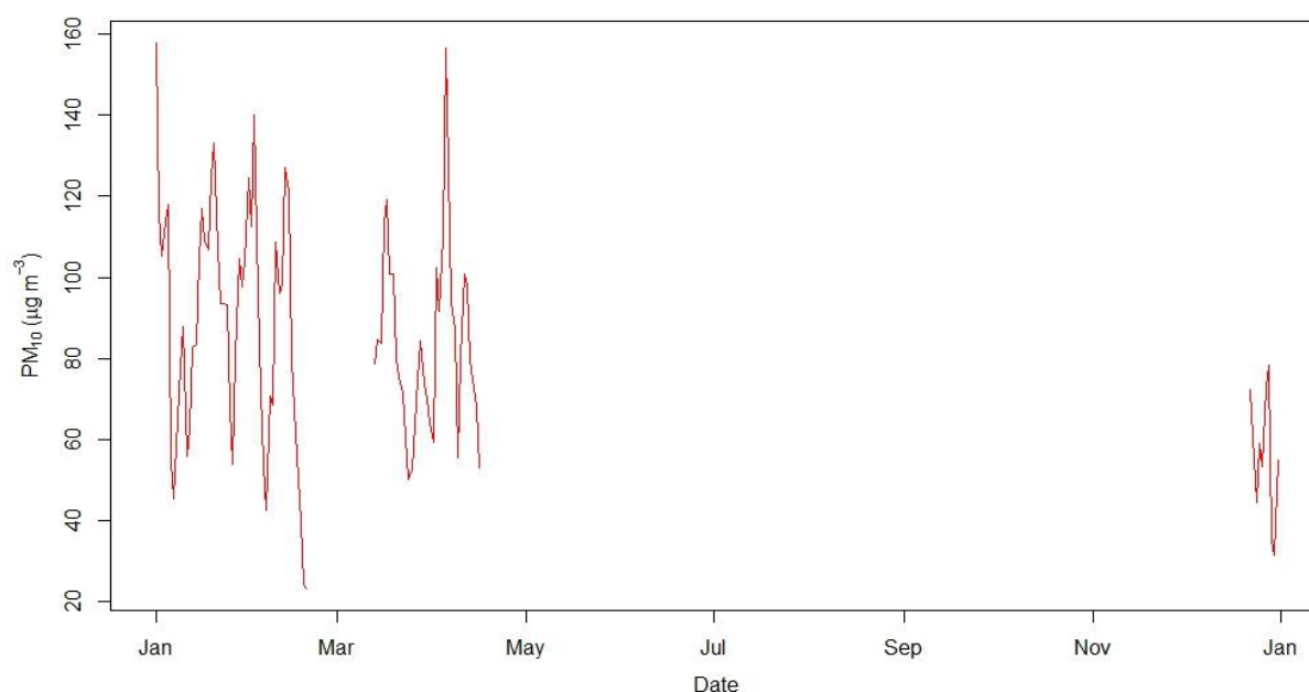
Figure 2.4.12: Daily mean concentration of PM 10
