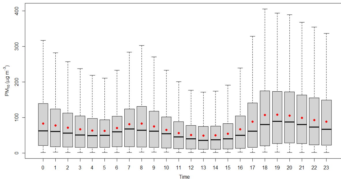
Figure 2.14.11: Diurnal variation of PM 10
