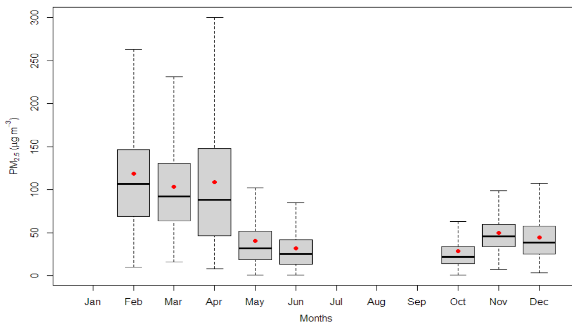
Figure 2.2.5: Monthly variation of PM 2.5
