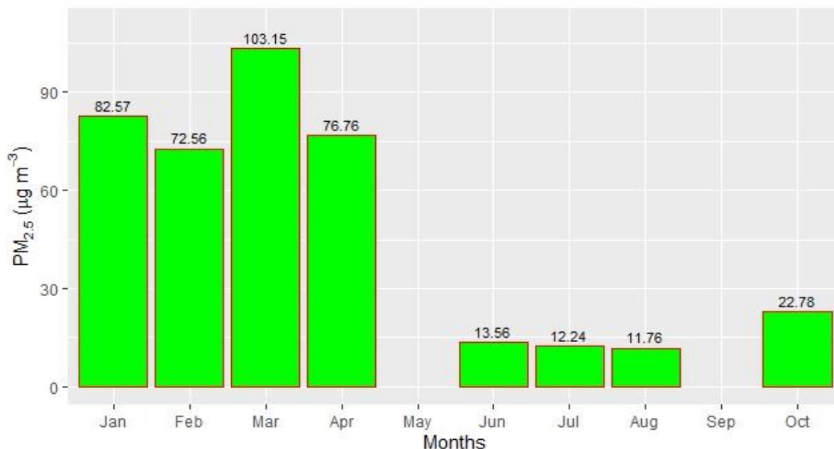
Figure 2.9.5: Monthly average PM 2.5
