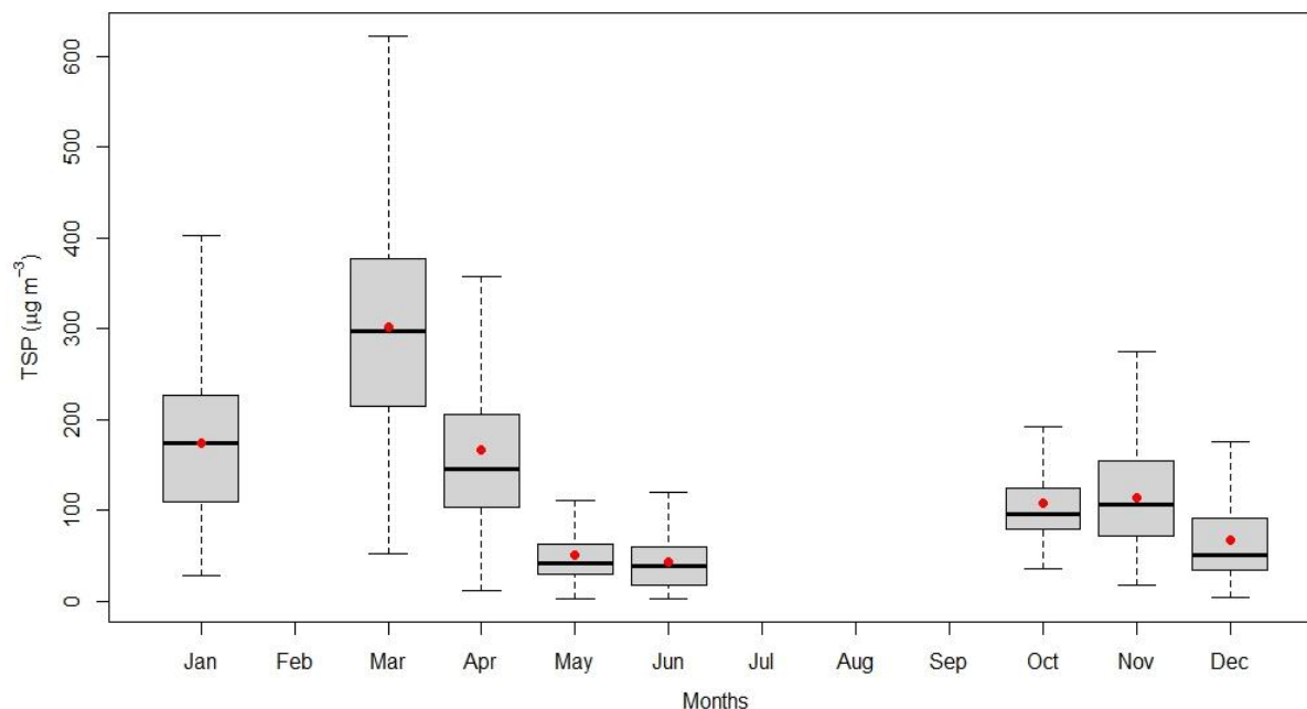
Figure 2.12.19: Monthly variation of TSP
