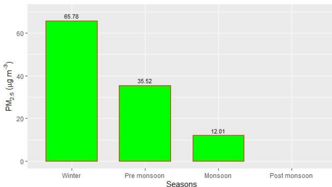
Figure 2.5.7: Seasonal variation of PM 2.5
