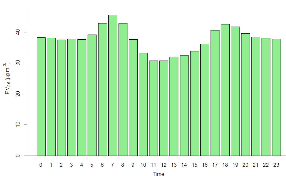
Figure 2.16.2: Hourly average of PM 2.5 .
