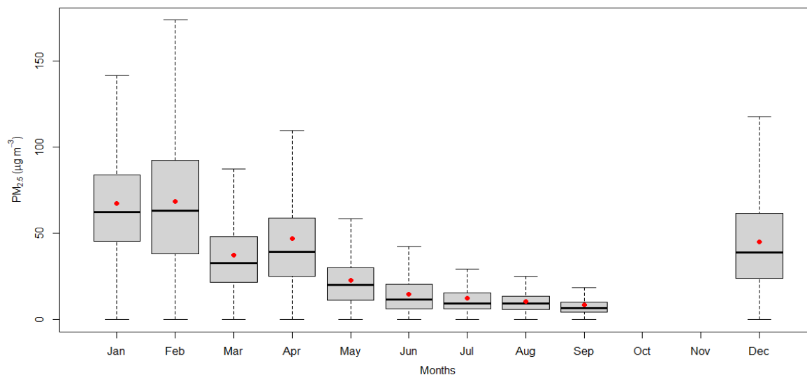
Figure 2.5.5: Monthly variation of PM 2.5
