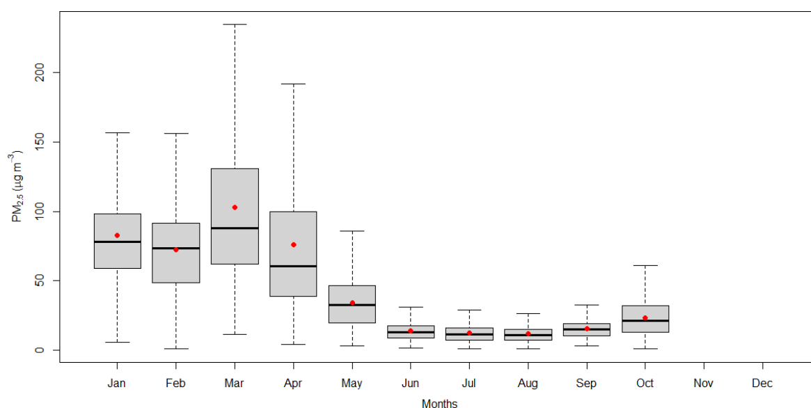
Figure 2.9.6: Monthly variation of PM 2.5
