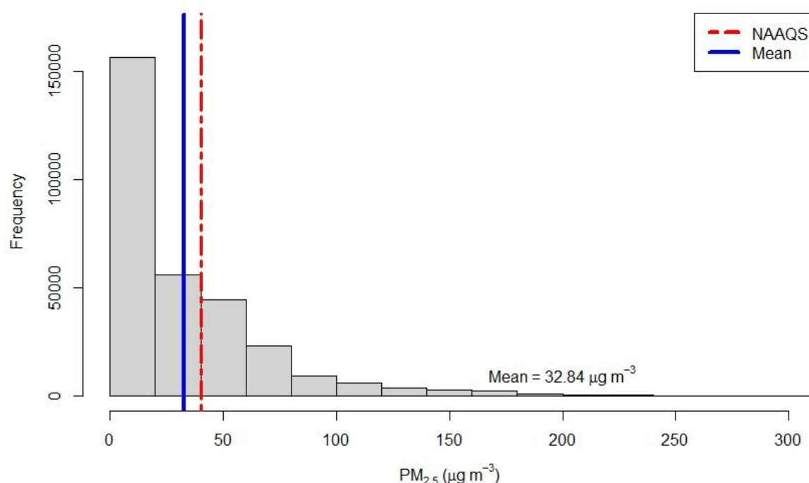
Figure 2.7.1: Histogram of PM 2.5
