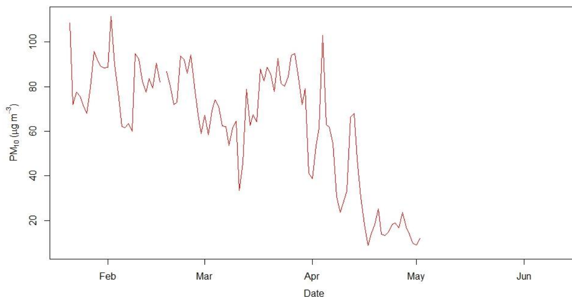
Figure 2.15.11: Daily mean concentration of PM 10
