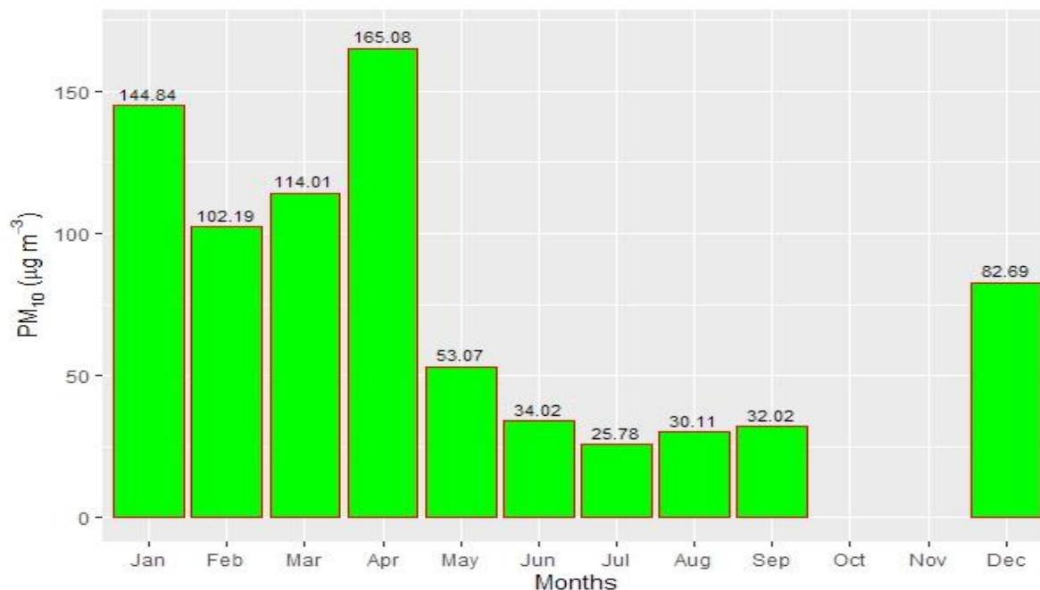
Figure 2.10.14: Monthly average of PM 10
