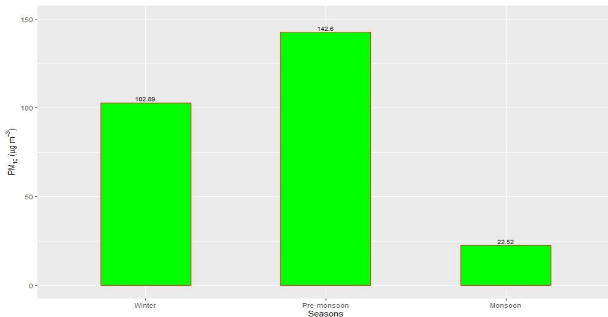
Figure 2.8.15: Seasonal variation of PM 10
