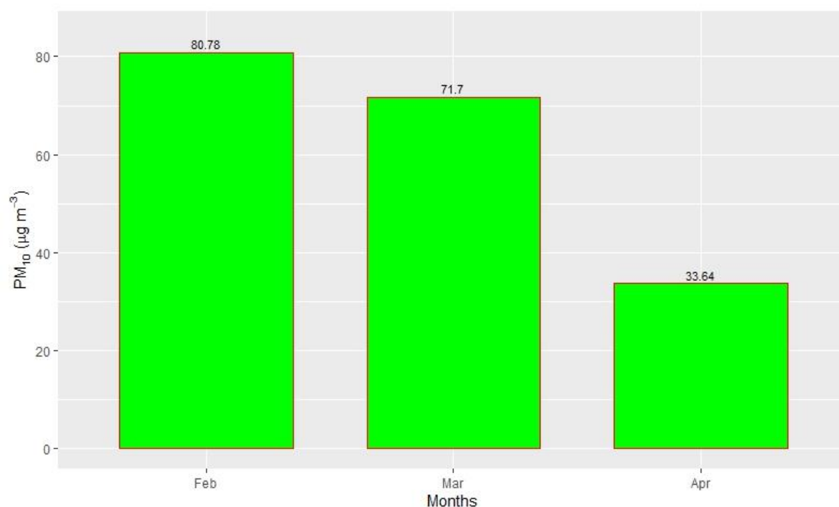
Figure 2.15.13: Seasonal variation of PM 10
