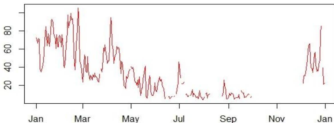
Figure 2.5.4: Daily mean concentration of PM 2.5
