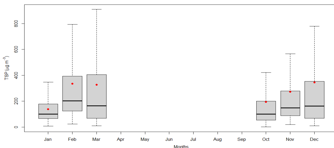
Figure 2.1.22: Monthly variation of TSP
