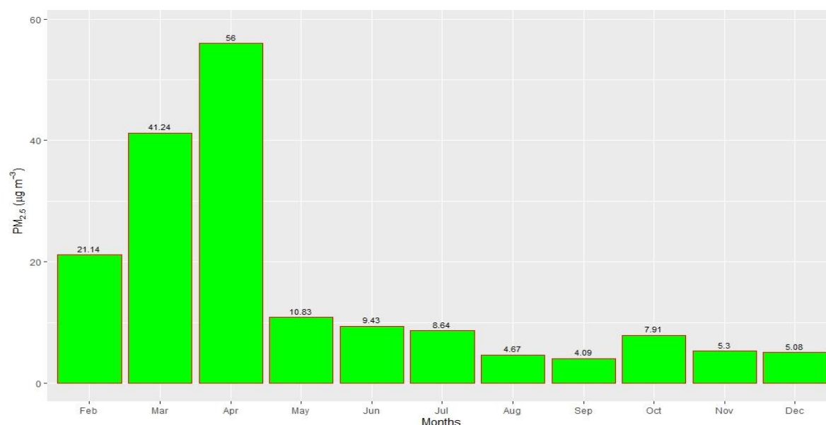
Figure 2.3.6: Monthly average PM_{2.5}
