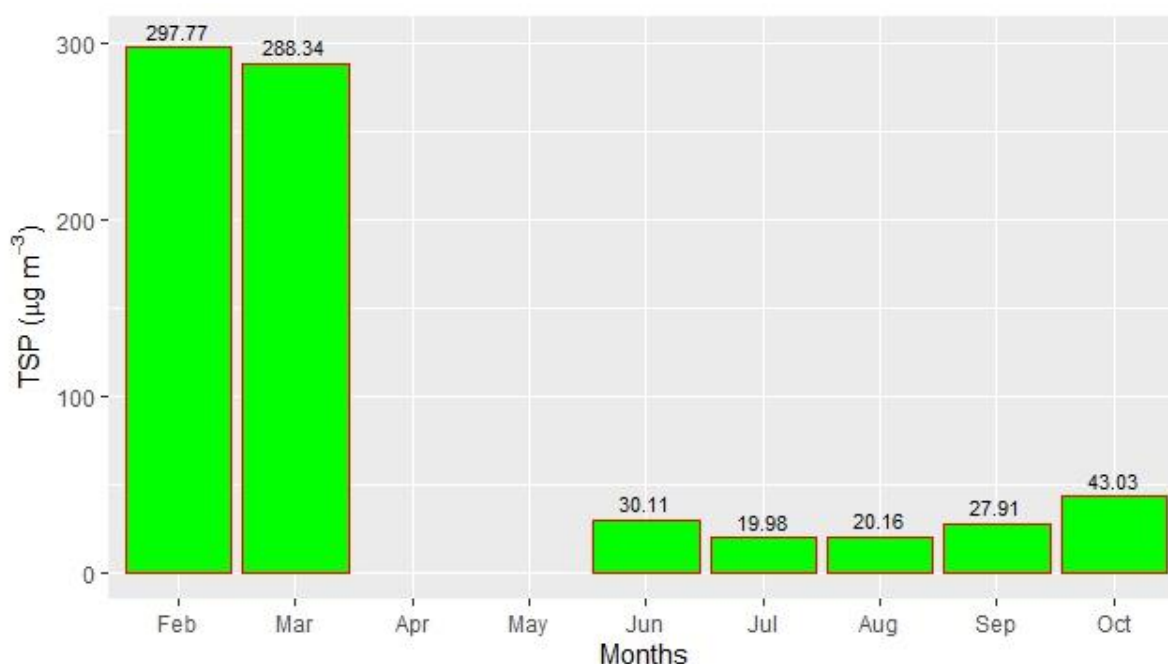
Figure 2.17.22: Monthly average of TSP
